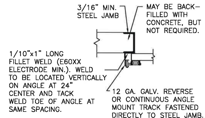
SECTION 3-3
