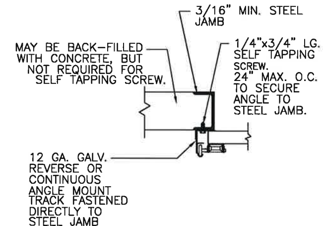
SECTION 3-3
