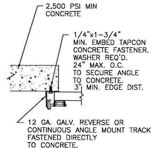
SECTION 3-3
