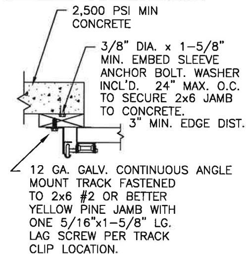
SECTION 3-3
