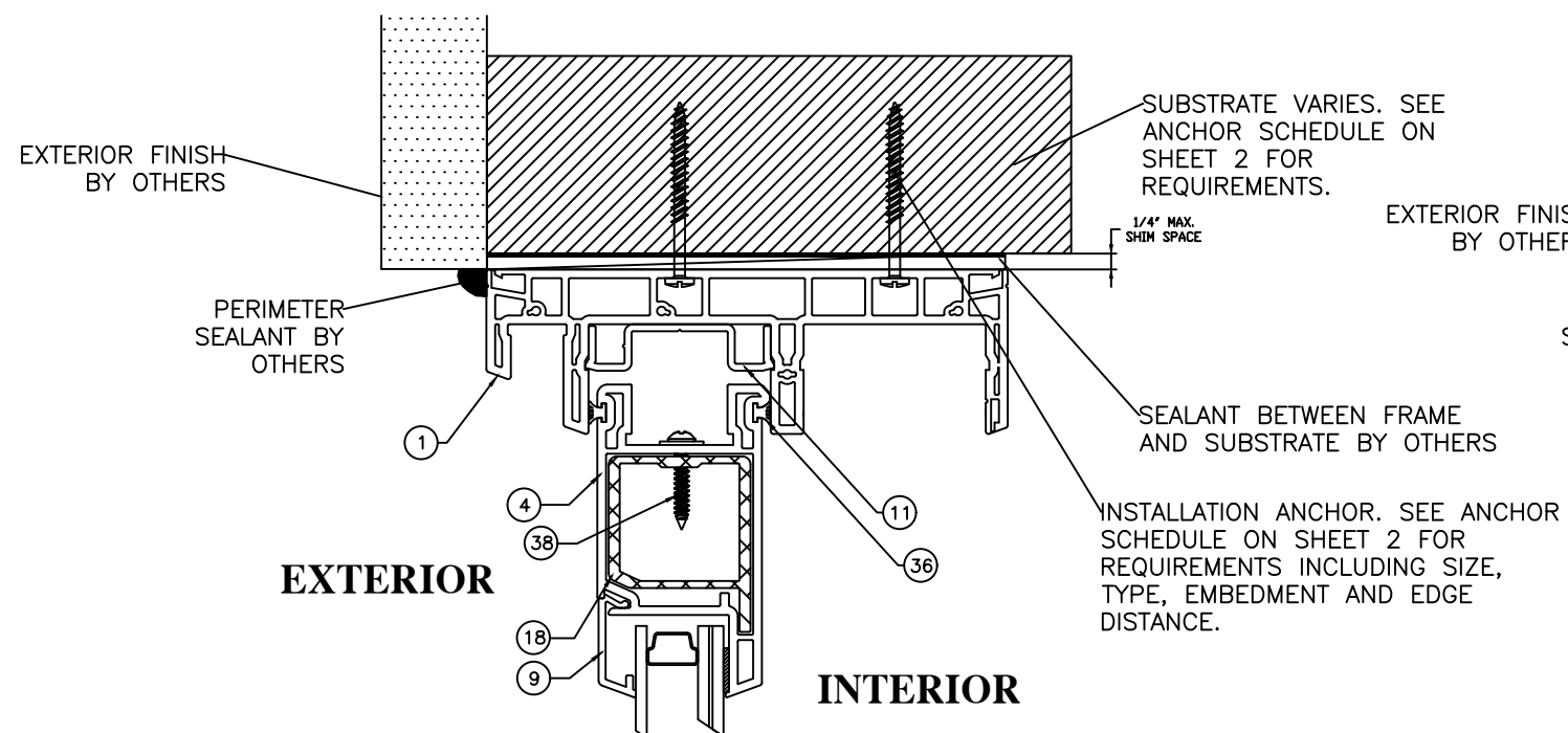
HEAD CROSS SECTION THROUGH-FRAME INSTALLATION FIXED DOOR PANEL
