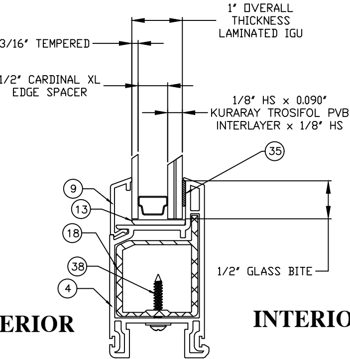
GLAZING DETAIL A
