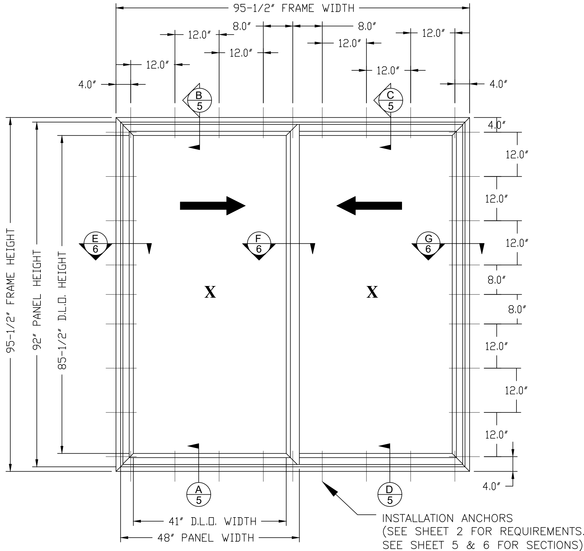
SERIES 9700 VINYL XX SLIDING GLASS DOOR - GLAZING DETAIL A EXTERIOR VIEW (95-1/2" X 95-1/2" SIZE SHOWN, NOMINAL 96" X 96")
