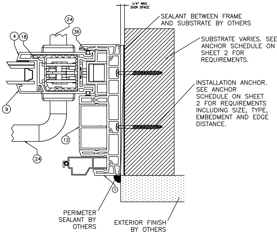
G 6 JAMB CROSS SECTION THROUGH-FRAME INSTALLATION OPERABLE DOOR PANEL
