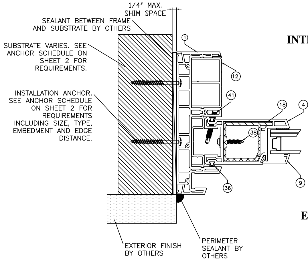
F 7 JAMB CROSS SECTION THROUGH-FRAME INSTALLATION FIXED DOOR PANEL
