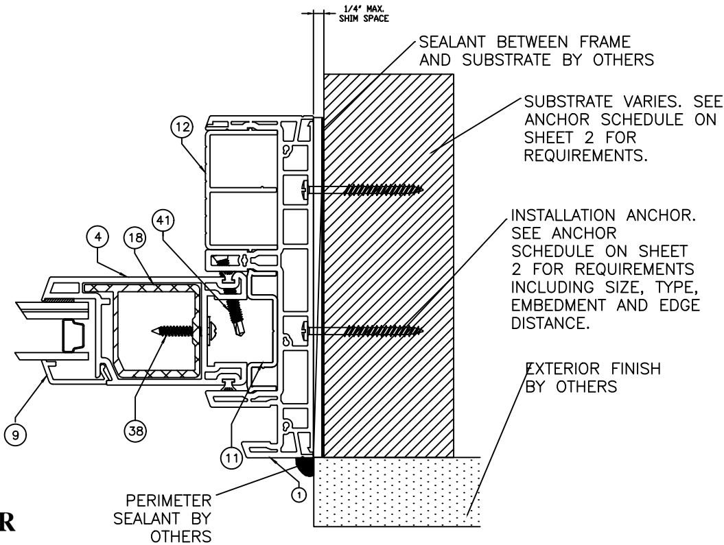
I 7 JAMB CROSS SECTION THROUGH-FRAME INSTALLATION FIXED DOOR PANEL
