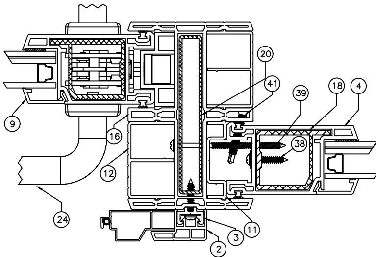
H 7 OXO ADAPTER CROSS SECTION THROUGH-FRAME INSTALLATION OPERABLE/FIXED DOOR PANEL
