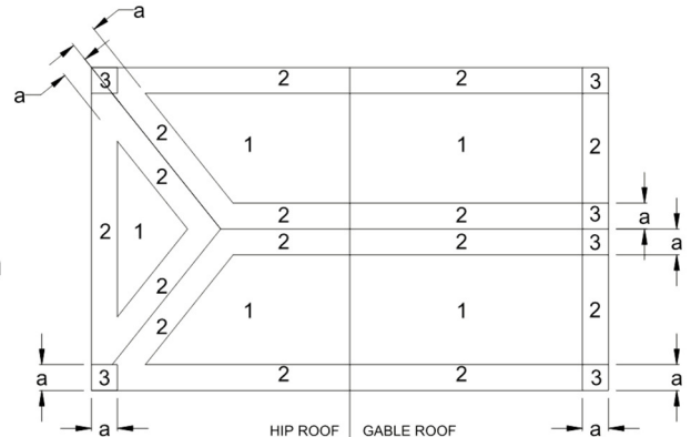
ROOF ZONES FOR GENERIC BUILDING
