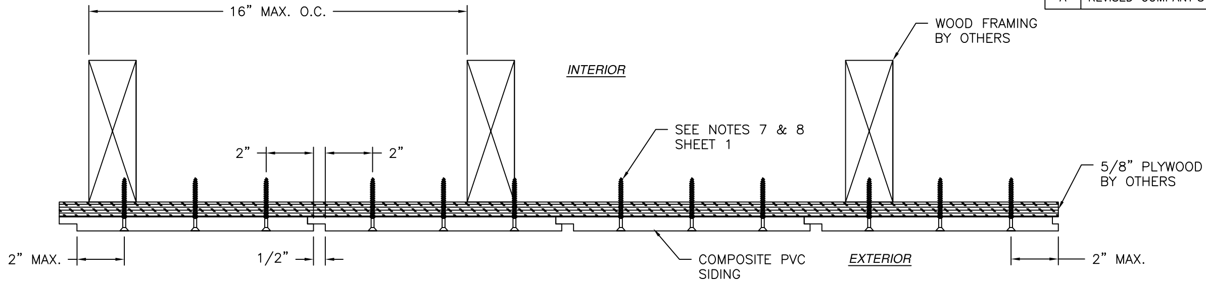
1/2" GROOVE INSTALLATION DETAIL 10" MODERN SHIPLAP SIDING SHOWN, 4", 6" AND 8" SIMILAR
