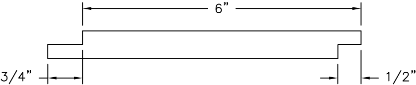
6" MODERN SHIPLAP, 1/4" GROOVE COMPOSITE PVC 5/8" THICK
