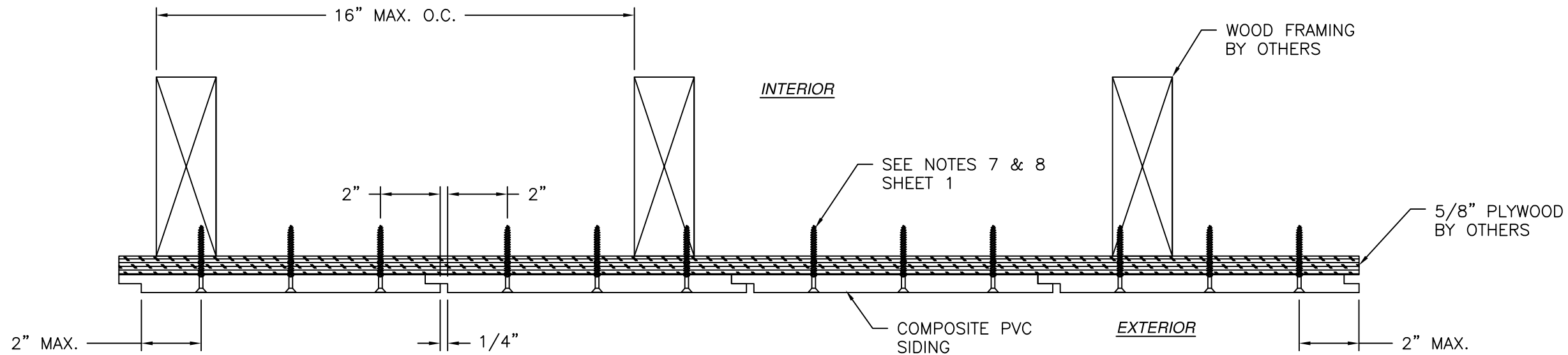
1/4" GROOVE INSTALLATION DETAIL 10" MODERN SHIPLAP SIDING SHOWN, 4", 6" AND 8" SIMILAR
