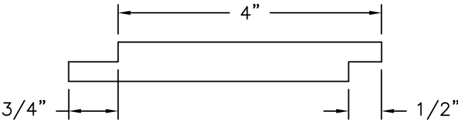
4" MODERN SHIPLAP, 1/4" GROOVE COMPOSITE PVC 5/8" THICK
