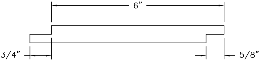
6" MODERN SHIPLAP, 1/8" GROOVE COMPOSITE PVC 5/8" THICK
