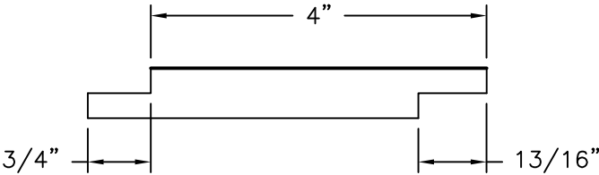
4" MODERN SHIPLAP FLUSH FIT COMPOSITE PVC 5/8" THICK
