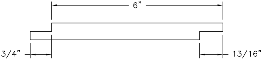
6" MODERN SHIPLAP FLUSH FIT COMPOSITE PVC 5/8" THICK
