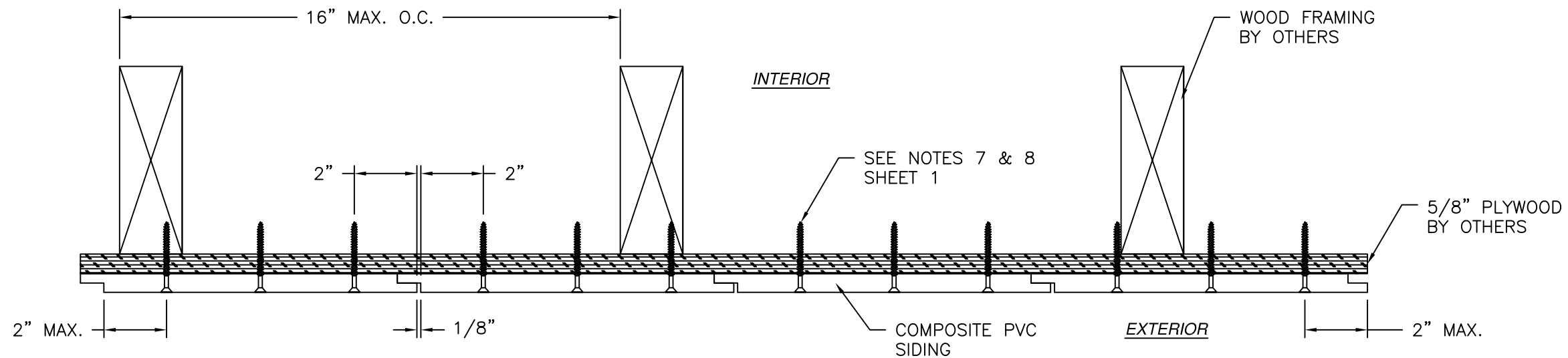
1/8" GROOVE INSTALLATION DETAIL 10" MODERN SHIPLAP SIDING SHOWN, 4", 6" AND 8" SIMILAR
