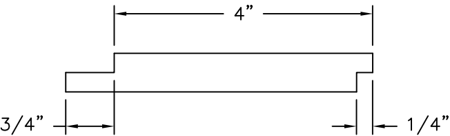
4" MODERN SHIPLAP, 1/2" GROOVE COMPOSITE PVC 5/8" THICK
