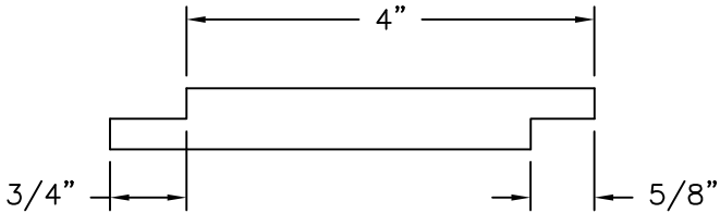
4" MODERN SHIPLAP, 1/8" GROOVE COMPOSITE PVC 5/8" THICK
