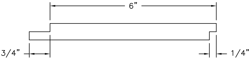
6" MODERN SHIPLAP, 1/2" GROOVE COMPOSITE PVC 5/8" THICK
