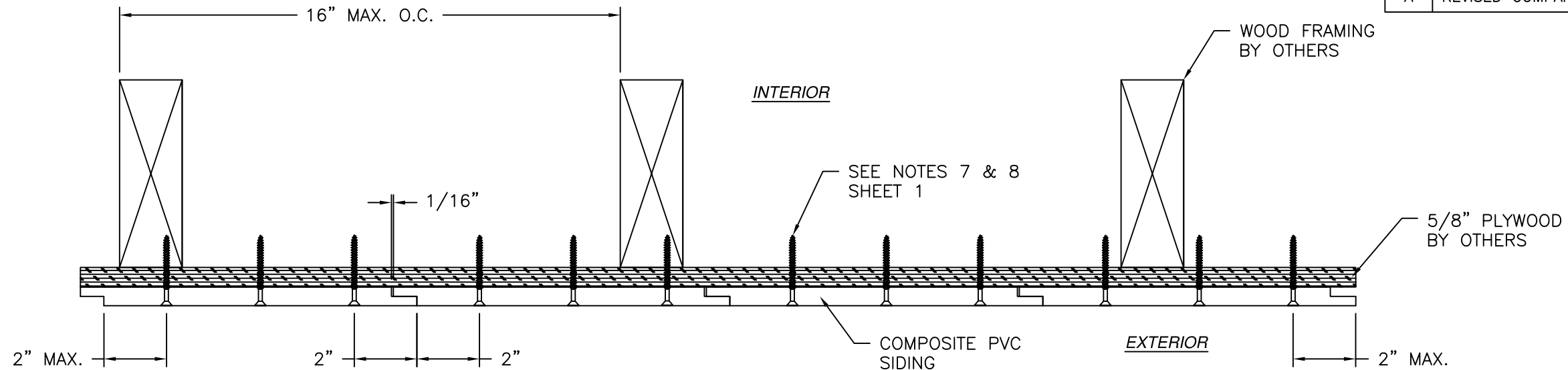
FLUSH FIT INSTALLATION DETAIL 10" MODERN SHIPLAP SIDING SHOWN, 4", 6" AND 8" SIMILAR
