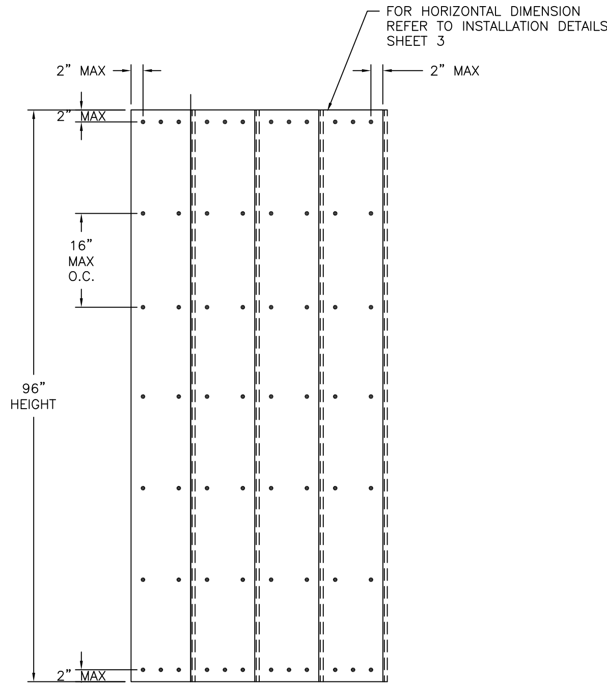
MODERN SHIPLAP VERTICAL SIDING EXTERIOR VIEW
