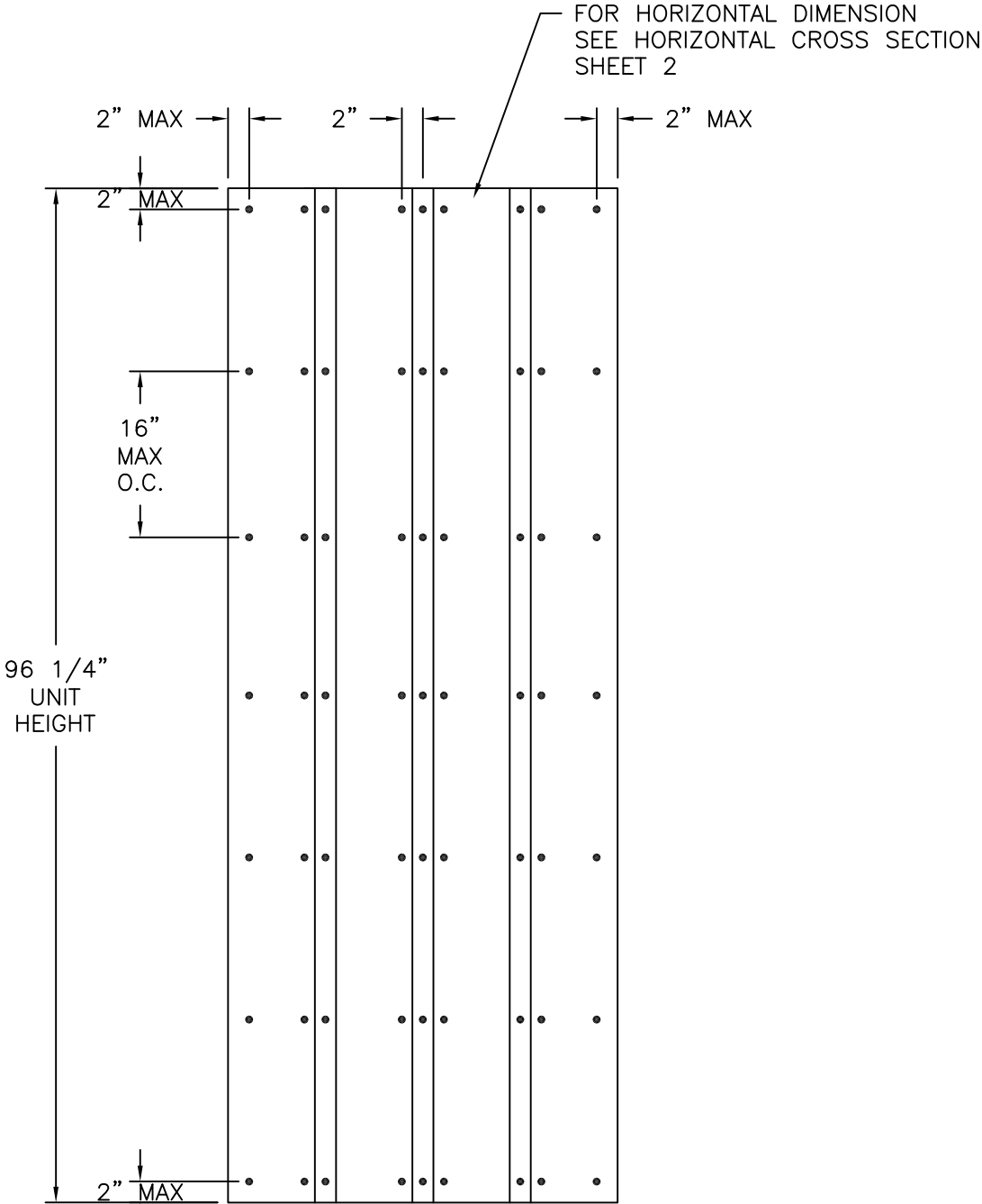
BOARD AND BATTEN 10" VERTICAL SIDING EXTERIOR VIEW
