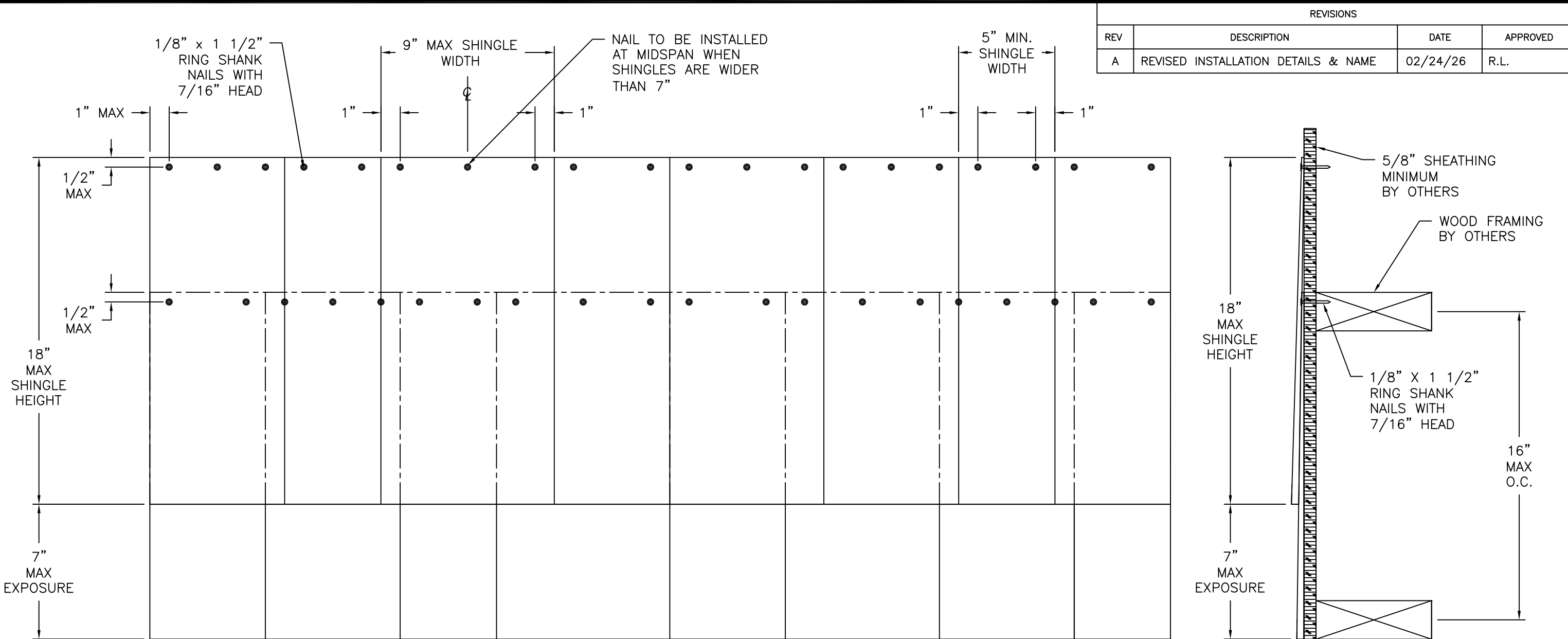
NUCEDAR 18" ROUGHSAWN SHINGLES EXTERIOR VIEW
