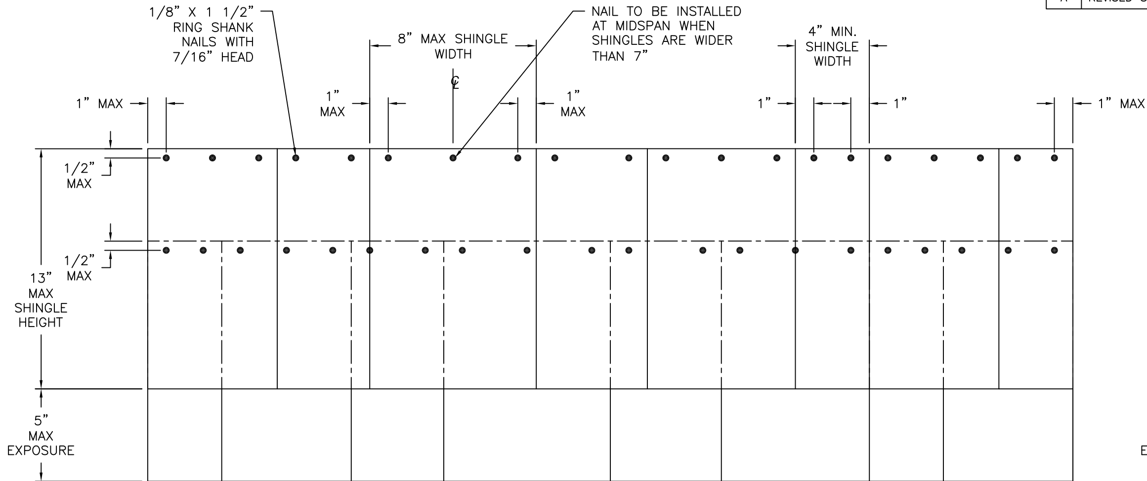
NUCEDAR 13" ROUGHSAWN SHINGLES EXTERIOR VIEW
