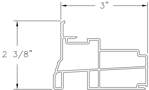
HEAD AND SILL FRAME EXTRUDED PVC (10002930)
