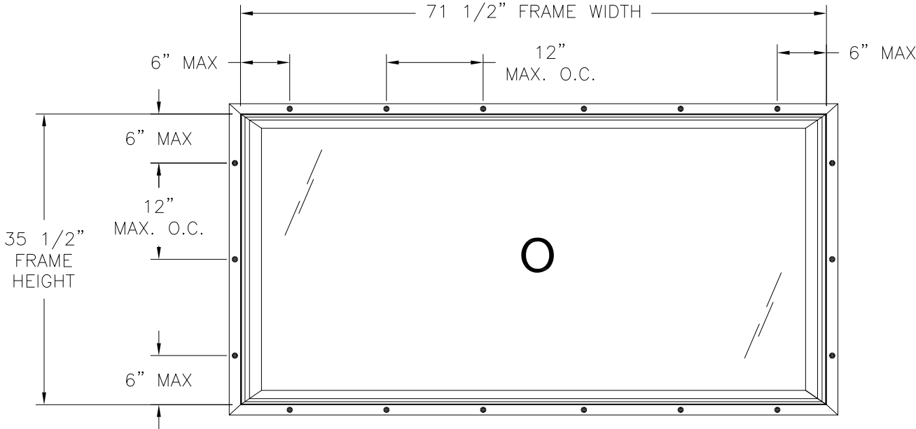
SERIES 901/951 PVC FIXED WINDOW EXTERIOR VIEW FIN INSTALLATION
