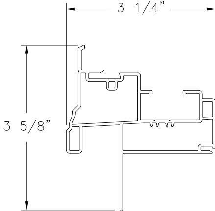
JAMB FIN INSTALLATION EXTRUDED PVC (10002932)
