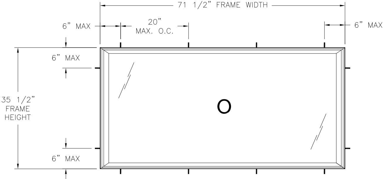
SERIES 901/951 PVC FIXED WINDOW EXTERIOR VIEW FRAME INSTALLATION
