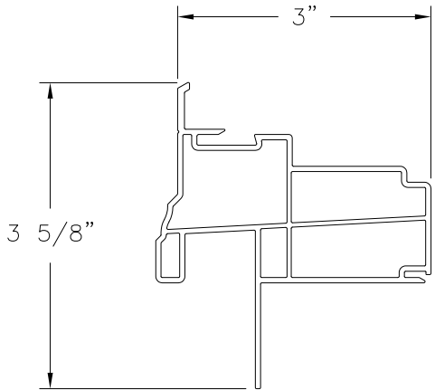
HEAD AND SILL FRAME FIN INSTALLATION EXTRUDED PVC (10002930)
