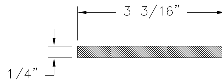
MULLION REINFORCEMENT 6063-T6 ALUMINUM (1538)
