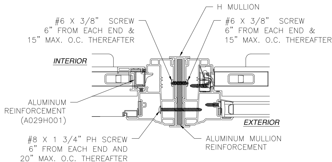
VERTICAL MULLION INSTALLATION DETAIL
