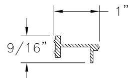
STILE REINFORCEMENT 6063-T6 ALUMINUM (A029H001)
