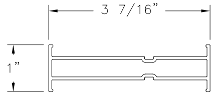
H MULLION EXTRUDED PVC (10002941)
