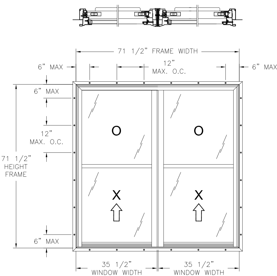
SERIES 900/950 PVC TWIN SINGLE HUNG WINDOW EXTERIOR VIEW FIN INSTALLATION
