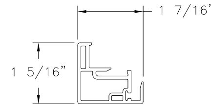
LOCK RAIL EXTRUDED PVC (10007703)
