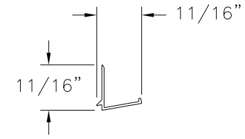
GLAZING BEAD RIGID PVC (VR-2445)
