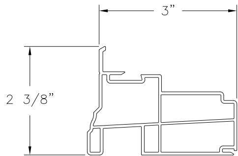
HEAD EXTRUDED PVC (10002930)
