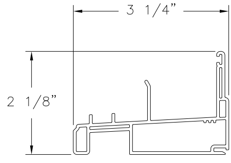
SILL EXTRUDED PVC (10002931)
