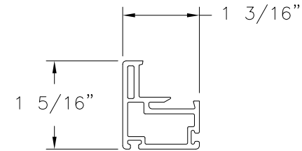
STILE EXTRUDED PVC (10004104)
