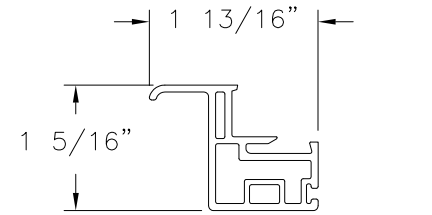
LIFT RAIL EXTRUDED PVC (10004105)
