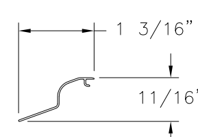
BALANCE COVER EXTRUDED PVC (10002942)
