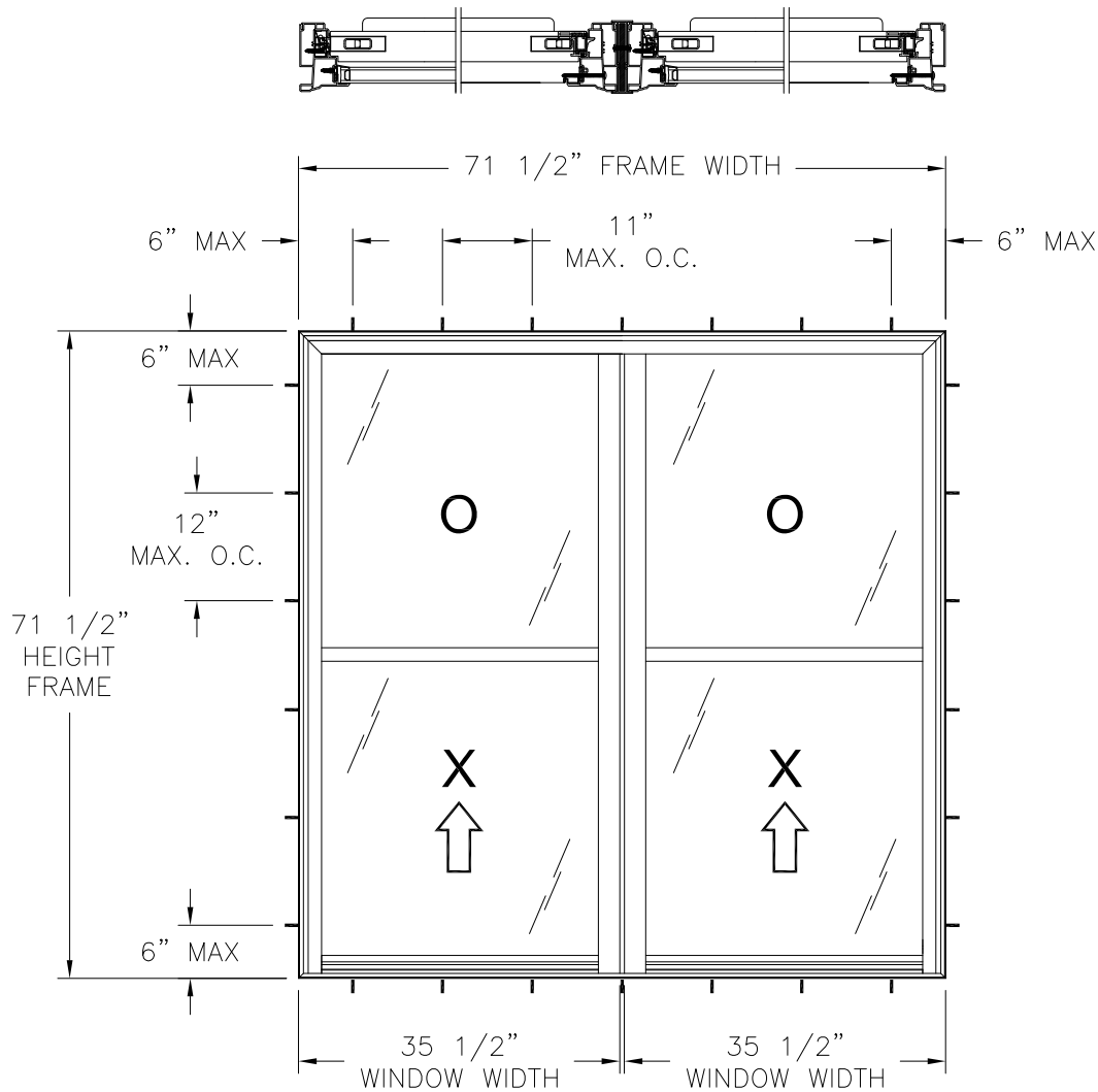
SERIES 900/950 PVC TWIN SINGLE HUNG WINDOW EXTERIOR VIEW FRAME INSTALLATION
