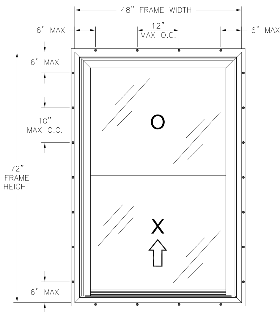
SERIES 900/950 VINYL SINGLE HUNG WINDOW EXTERIOR VIEW FIN INSTALLATION
