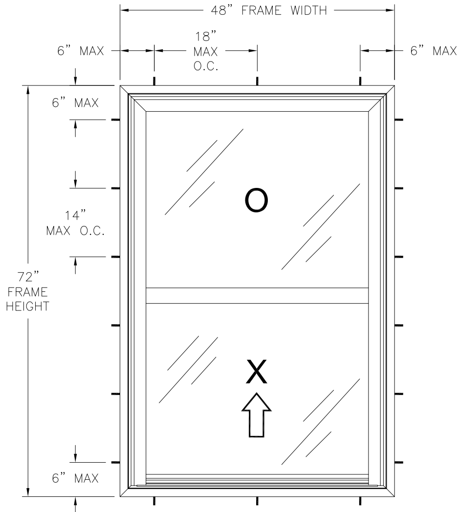
SERIES 900/950 VINYL SINGLE HUNG WINDOW EXTERIOR VIEW FRAME INSTALLATION
