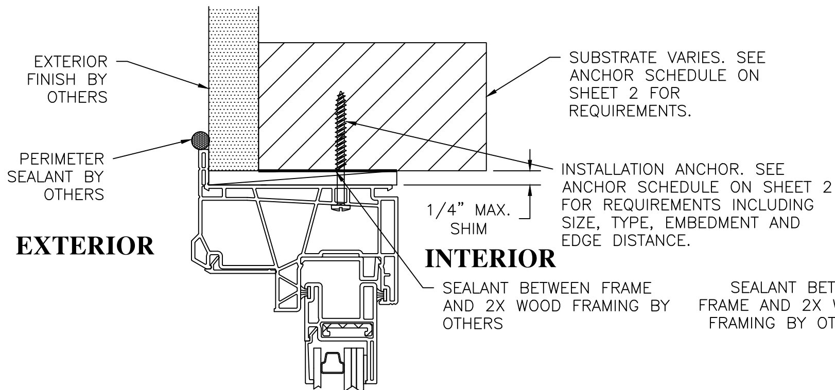
B 8 HEAD CROSS SECTION FLANGE THROUGH-FRAME INSTALLATION (SASH SHOWN, FIXED LITE SIMILAR)
