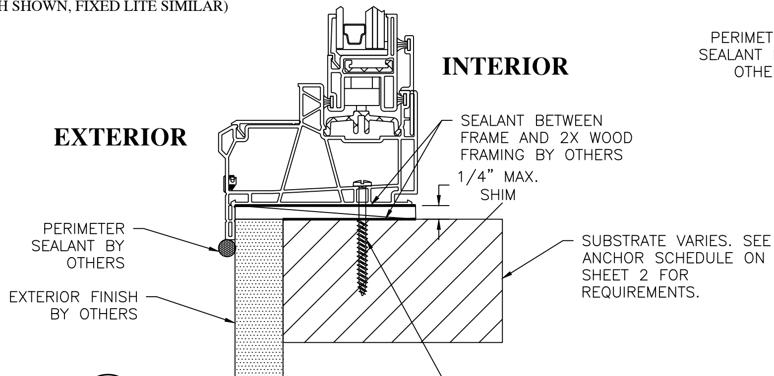
A 8 SILL CROSS SECTION FLANGE THROUGH-FRAME INSTALLATION (SASH SHOWN, FIXED LITE SIMILAR)
