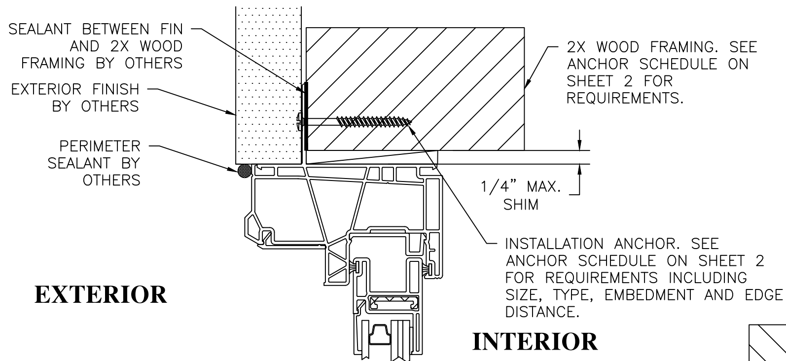
B 9 HEAD CROSS SECTION NAILING FIN FRAME INSTALLATION (SHOWN W/O FLANGE)
