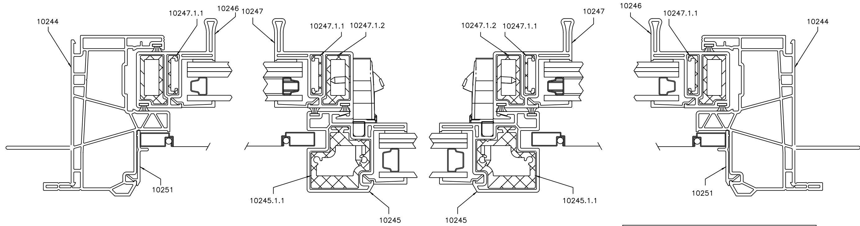
SECTION VIEWS WITH COMPONENT PART NUMBERS
