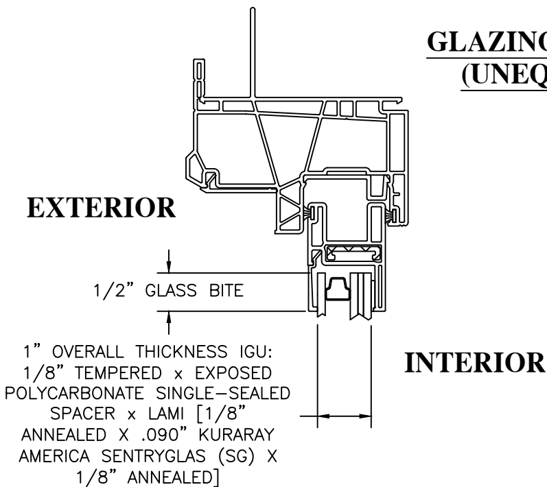
GLAZING DETAIL A
