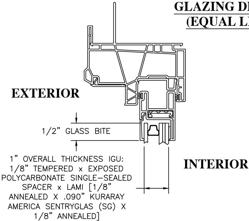
GLAZING DETAIL C
