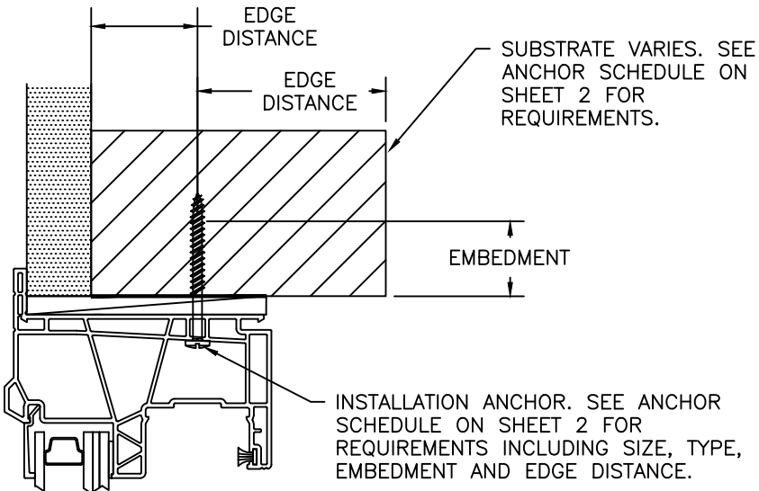
EMBEDMENT AND EDGE DISTANCE FLANGE THROUGH-FRAME INSTALLATION
