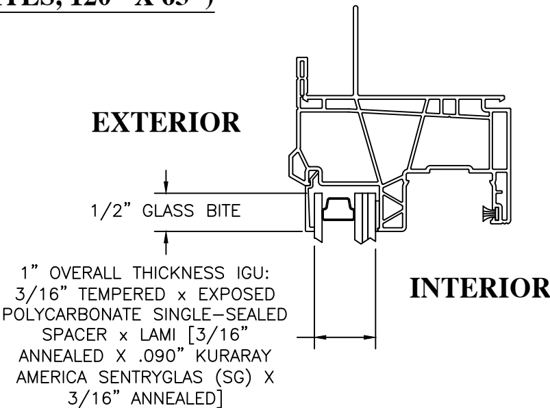
GLAZING DETAIL B
