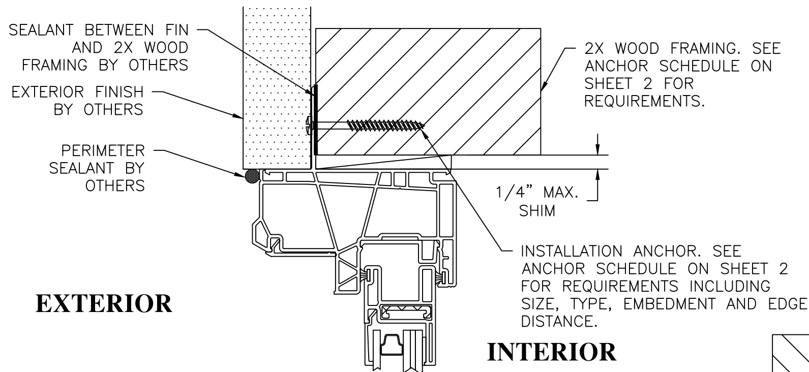
B 6 HEAD CROSS SECTION NAILING FIN FRAME INSTALLATION (SHOWN W/O FLANGE)
