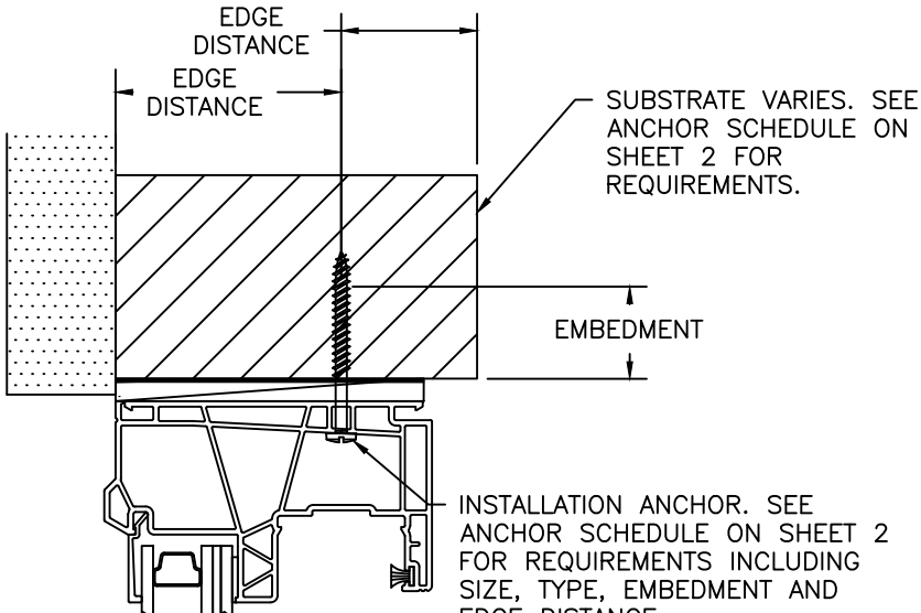
EMBEDMENT AND EDGE DISTANCE THROUGH-FRAME INSTALLATION
