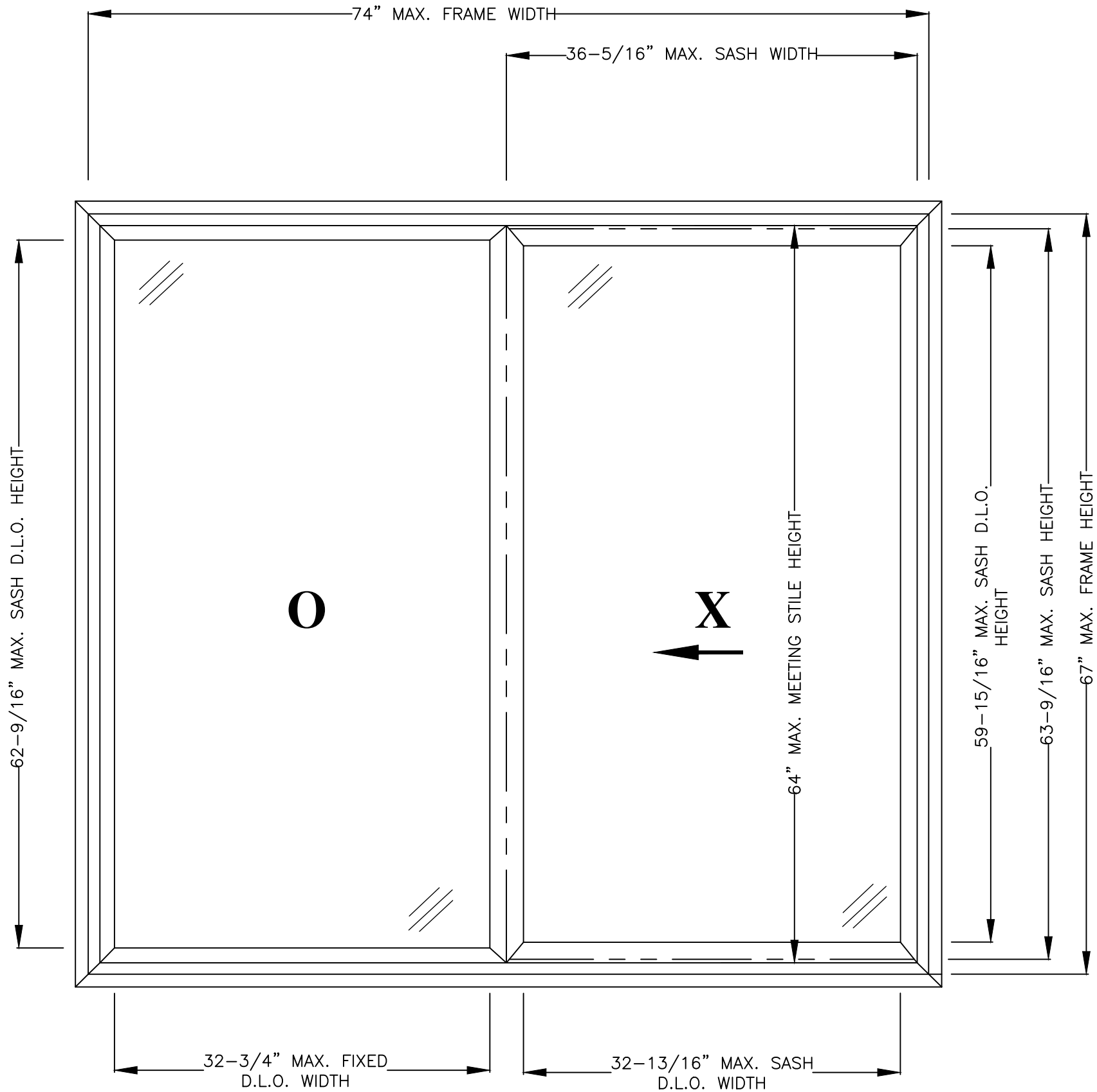
SERIES 10400 VINYL HORIZONTAL SLIDING WINDOW EXTERIOR VIEW 74" x 67" NOMINAL SIZE (OX SHOWN - XO ENVELOPED) FIN FRAME SHOWN (FOR THROUGH FRAME ANCHORING, FIN IS REMOVED)
