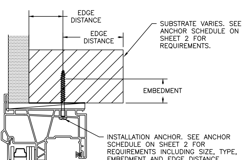
EMBEDMENT AND EDGE DISTANCE FLANGE THROUGH-FRAME INSTALLATION
