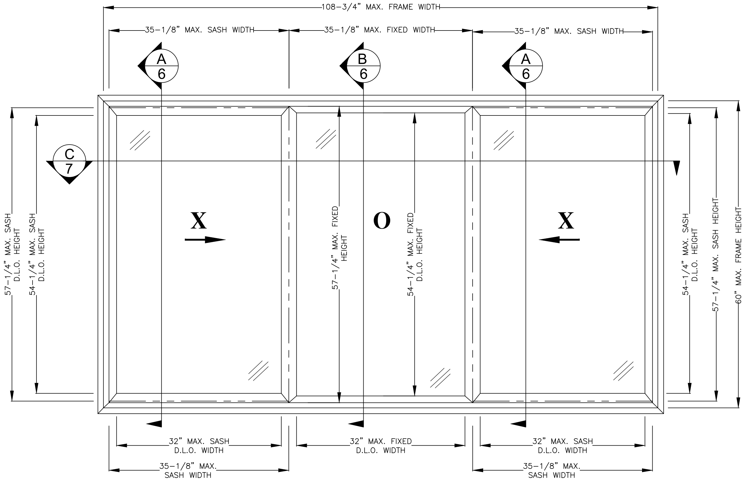
SERIES 8500 VINYL HORIZONTAL SLIDING WINDOW EXTERIOR VIEW - FIN FRAME SHOWN (FOR THROUGH FRAME ANCHORING, FIN IS REMOVED) 108" X 60" NOMINAL SIZE SHOWN XOX SHOWN
