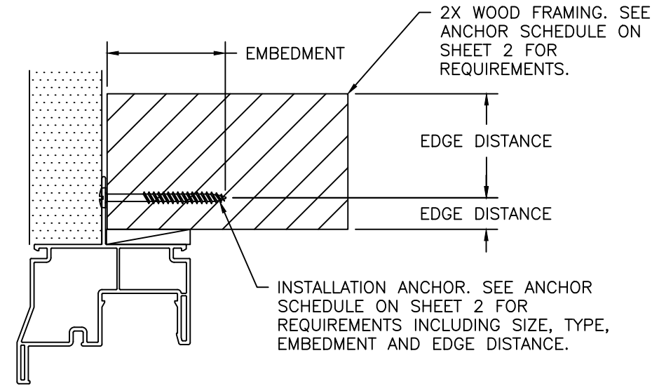
EMBEDMENT AND EDGE DISTANCE NAILING FIN FRAME INSTALLATION
