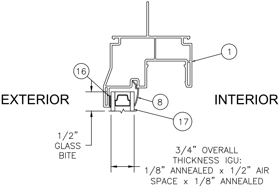
GLAZING DETAIL A
