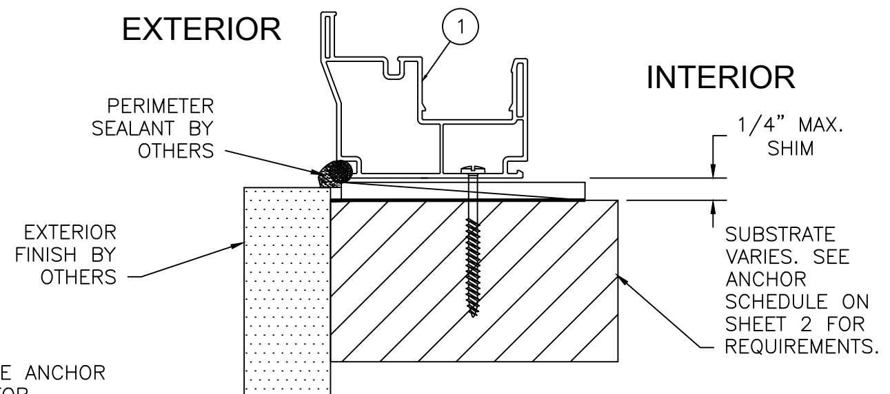
C 8 VERTICAL CROSS SECTION AT HEAD SHOWN. HORIZONTAL THROUGH JAMBS SAME. SNAP-ON FLANGE THROUGH-FRAME INSTALLATION
