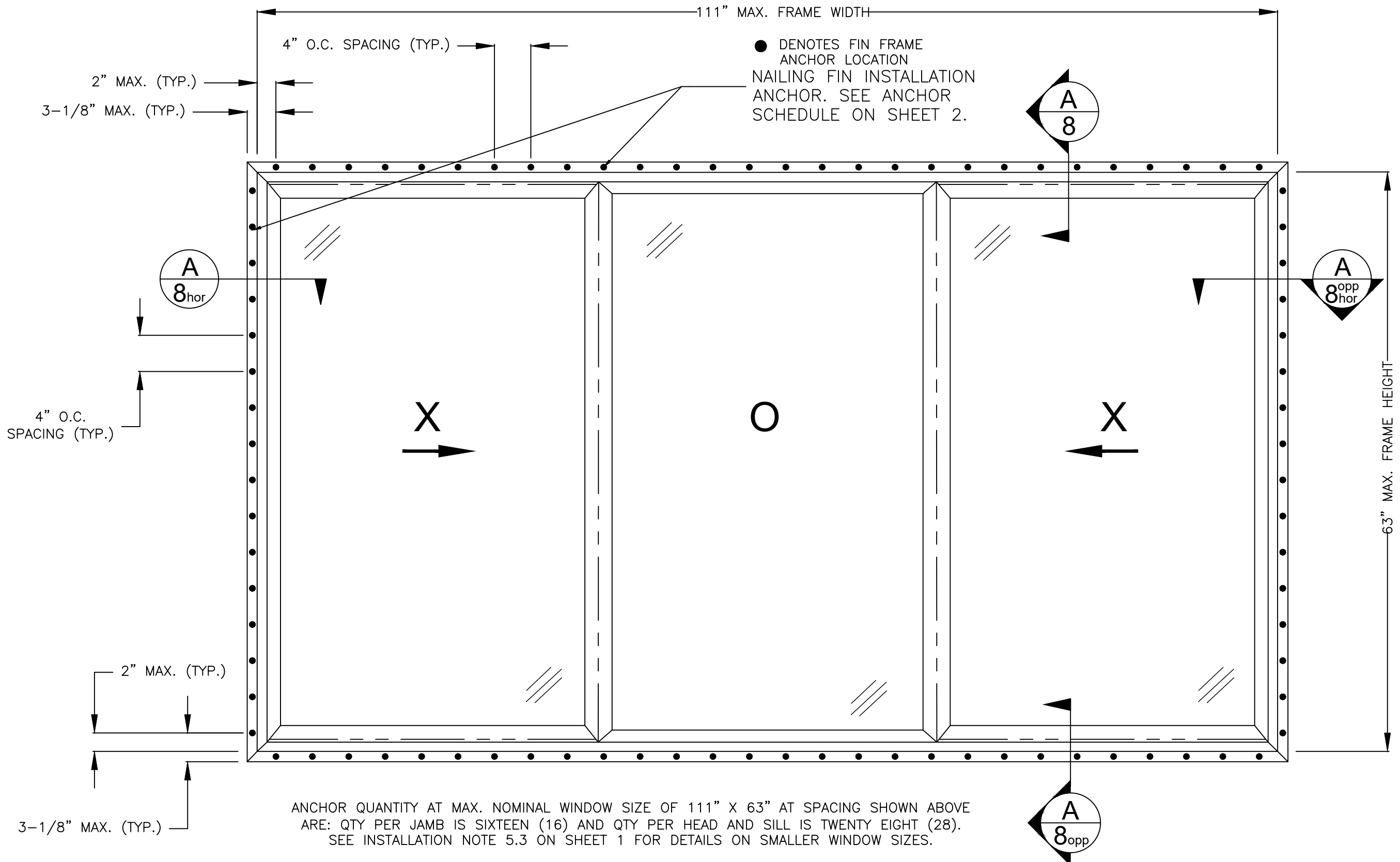
SERIES 8700 VINYL HORIZONTAL SLIDING WINDOW EXTERIOR VIEW (111" X 63" NOMINAL SIZE SHOWN) FIN FRAME ANCHOR LOCATIONS AND QUANTITIES
