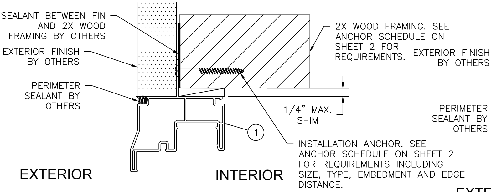
A 8 VERTICAL CROSS SECTION AT HEAD SHOWN. SILL AND HORIZONTAL CROSS SECTION THROUGH JAMBS SAME. NAILING FIN FRAME INSTALLATION
