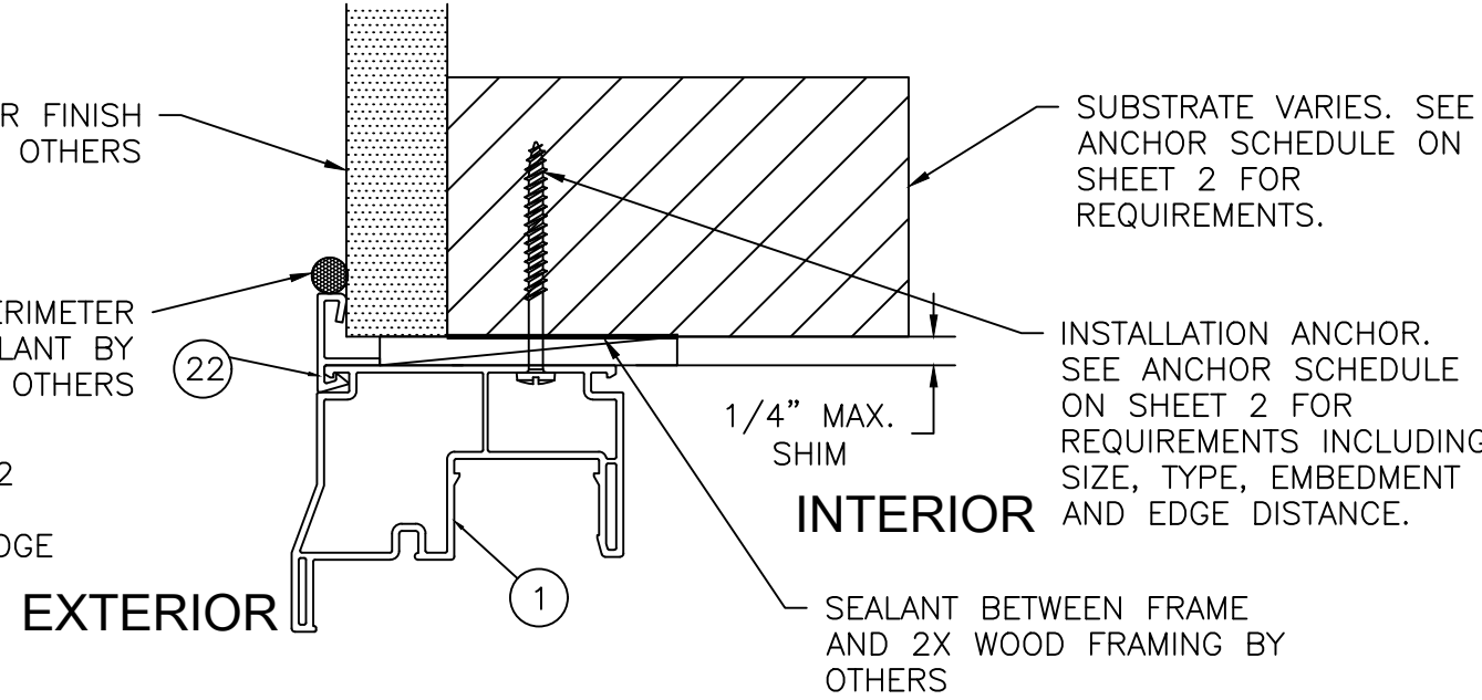
C 8 VERTICAL CROSS SECTION AT HEAD SHOWN. HORIZONTAL THROUGH JAMBS SAME. SNAP-ON FLANGE THROUGH-FRAME INSTALLATION
