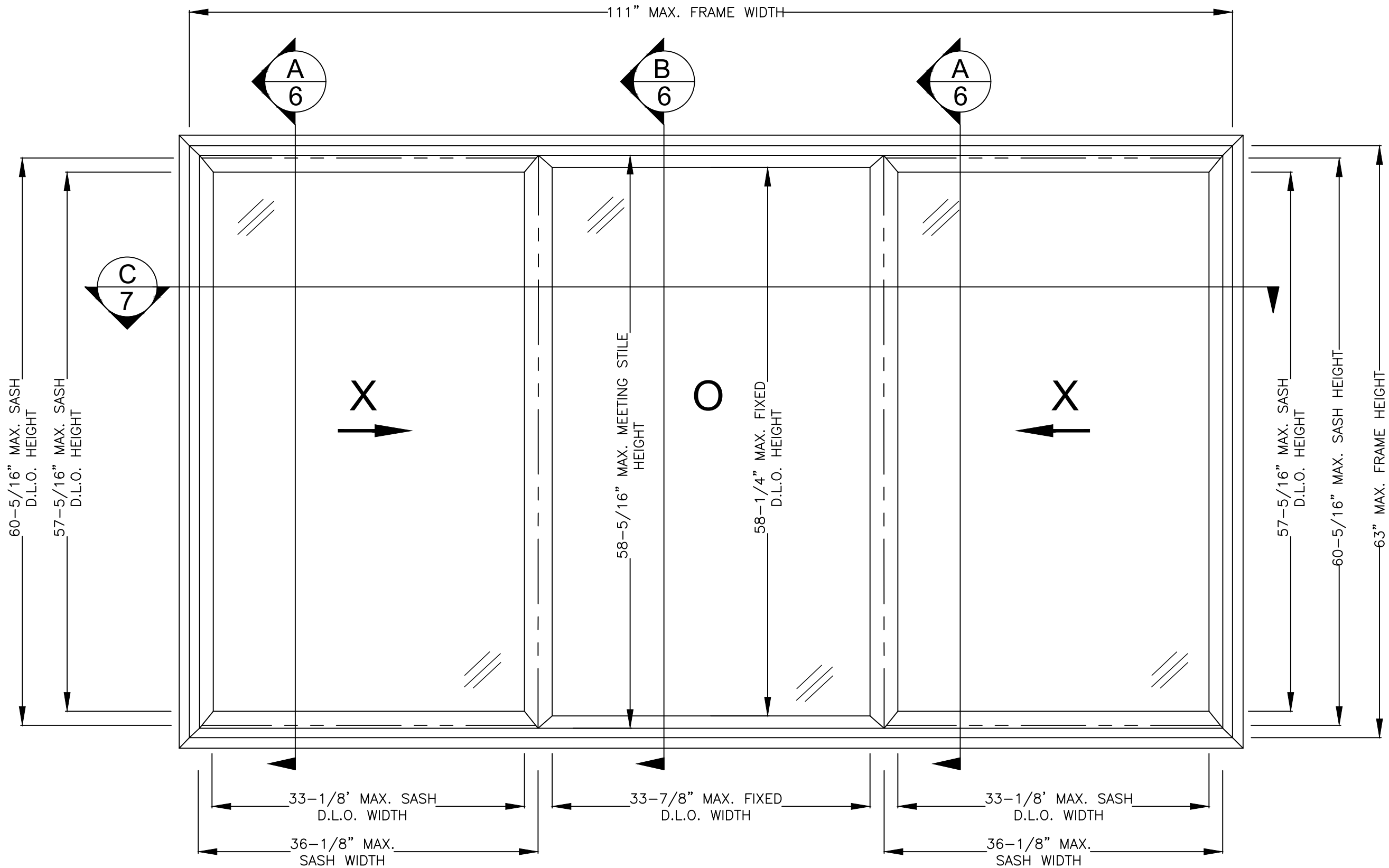
SERIES 8700 VINYL HORIZONTAL SLIDING WINDOW EXTERIOR VIEW - FIN FRAME SHOWN (FOR THROUGH FRAME ANCHORING, FIN IS REMOVED) 111" X 63" NOMINAL SIZE SHOWN XOX SHOWN
