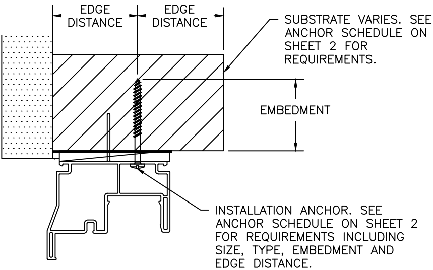
EMBEDMENT AND EDGE DISTANCE THROUGH-FRAME INSTALLATION - HEAD & JAMBS
