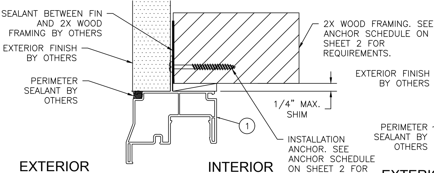
A 8 VERTICAL CROSS SECTION AT HEAD SHOWN. SILL AND HORIZONTAL CROSS SECTION THROUGH JAMBS SAME. NAILING FIN FRAME INSTALLATION
