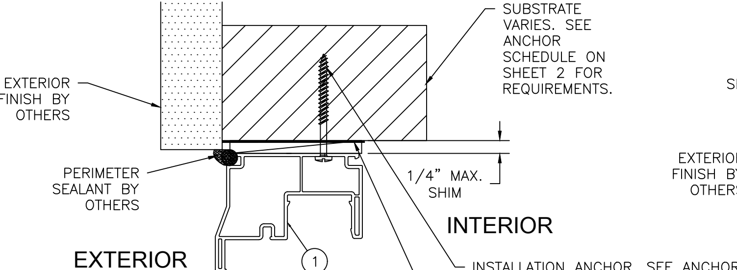
B 8 VERTICAL CROSS SECTION AT HEAD SHOWN. HORIZONTAL THROUGH JAMBS SAME. THROUGH-FRAME INSTALLATION
