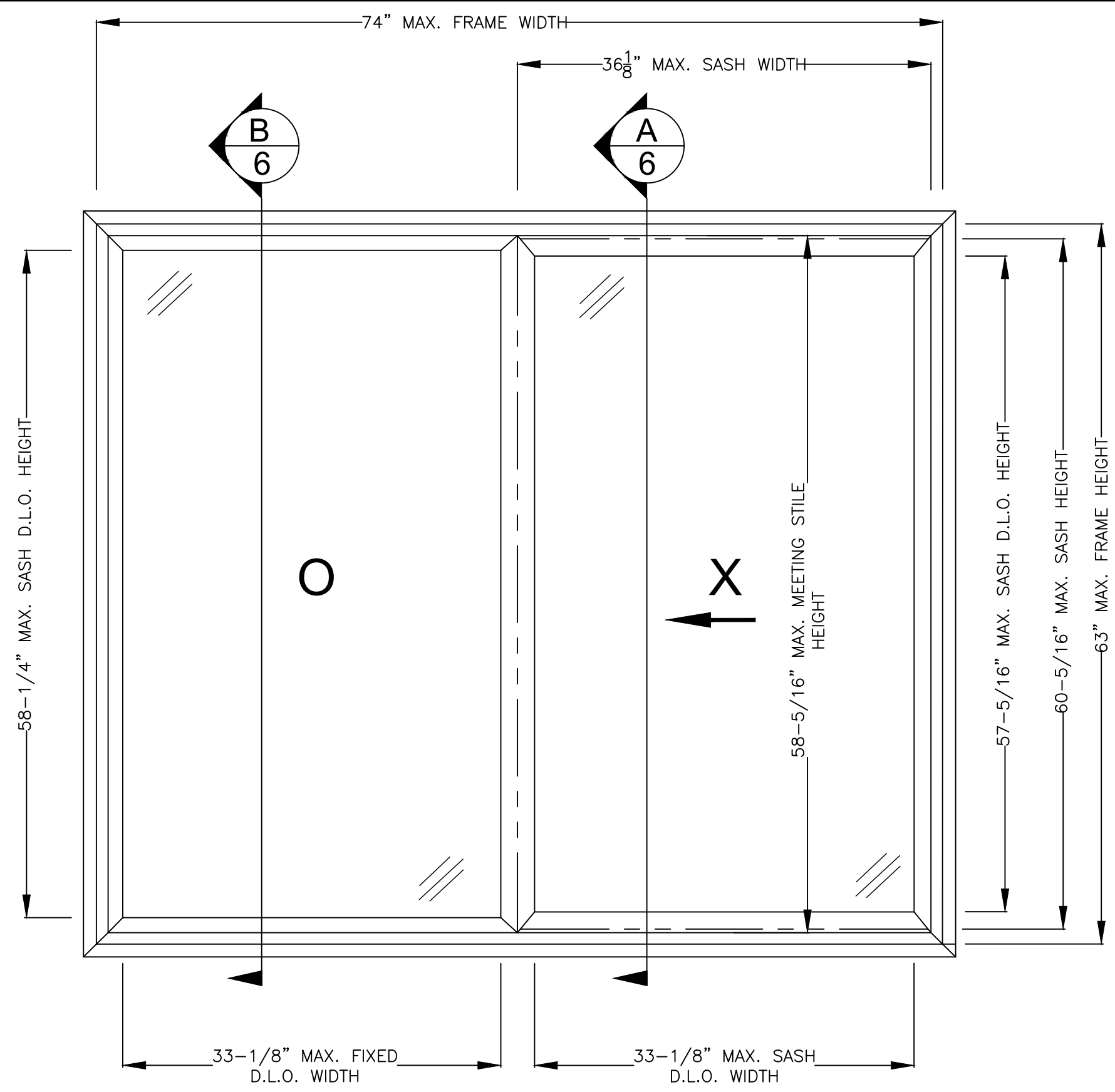
SERIES 8700 VINYL HORIZINTAL SLIDING WINDOW EXTERIOR VIEW - FIN FRAME SHOWN (FOR THROUGH FRAME ANCHORING, FIN IS REMOVED) 74" x 63" NOMINAL SIZE SHOWN OX SHOWN - XO ENVELOPED
