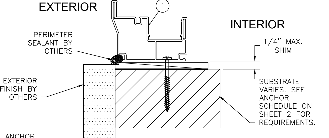
C 8 VERTICAL CROSS SECTION AT HEAD SHOWN. HORIZONTAL THROUGH JAMBS SAME. SNAP-ON FLANGE THROUGH-FRAME INSTALLATION
