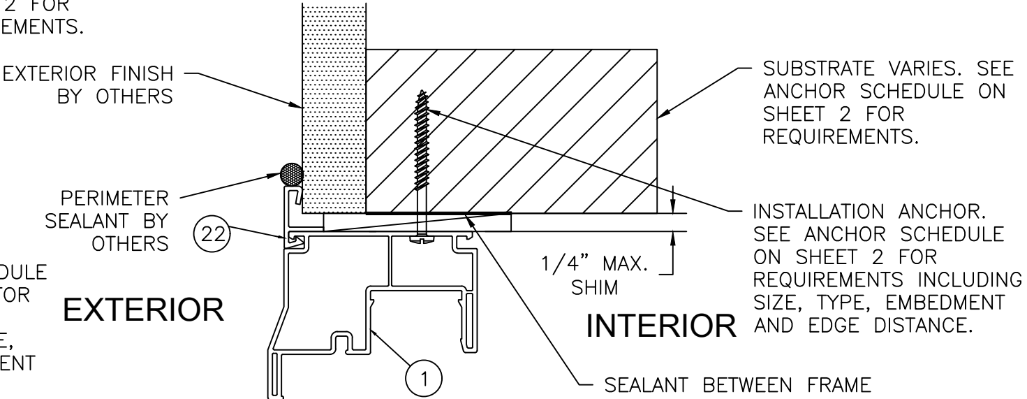
C 8 VERTICAL CROSS SECTION AT HEAD SHOWN. HORIZONTAL THROUGH JAMBS SAME. SNAP-ON FLANGE THROUGH-FRAME INSTALLATION
