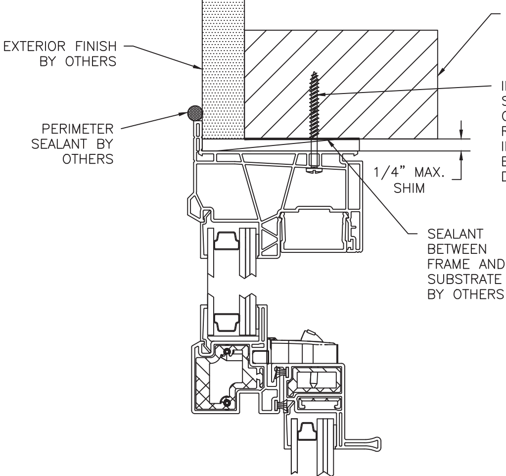
A VERTICAL CROSS SECTION THROUGH-FRAME INSTALLATION FLANGE
