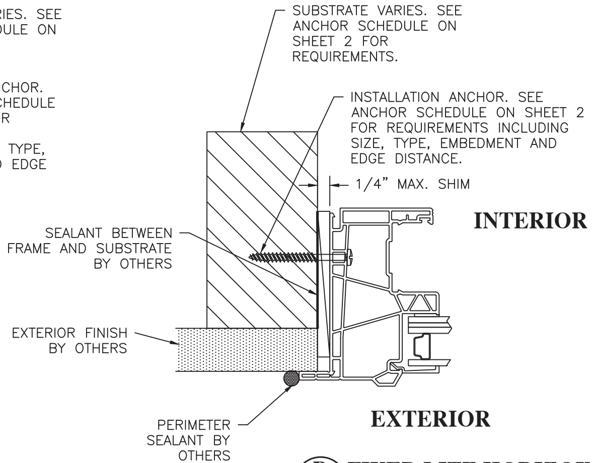
B FIXED LITE HORIZONTAL CROSS SECTION THROUGH-FRAME INSTALLATION FLANGE
