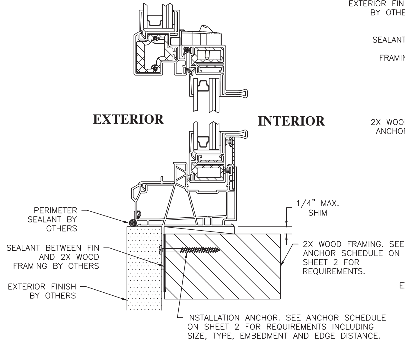
A 5 VERTICAL CROSS SECTION NAILING FIN FRAME INSTALLATION (SHOWN W/O FLANGE)
