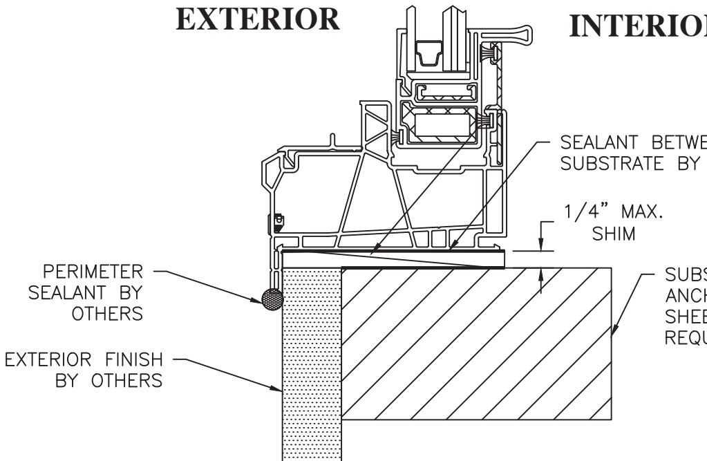
A VERTICAL CROSS SECTION THROUGH-FRAME INSTALLATION FLANGE
