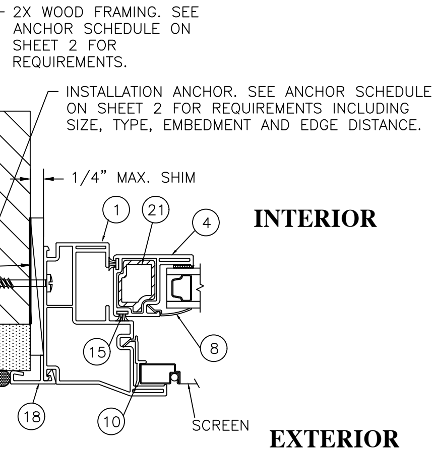
C 11 SASH LITE HORIZONTAL CROSS SECTION SNAP-ON FLANGE THROUGH-FRAME INSTALLATION
