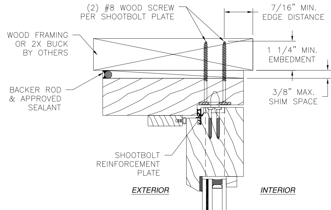
SHOOTBOLT STRIKE INSTALLATION WOOD FRAME OR 2X BUCK
