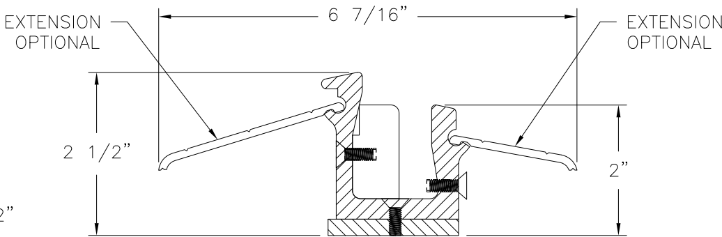
THRESHOLD ASSEMBLY
