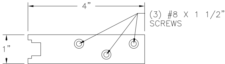
SHOOTBOLT REINFORCEMENT PLATE 1/4" THICKNESS, STAINLESS STEEL
