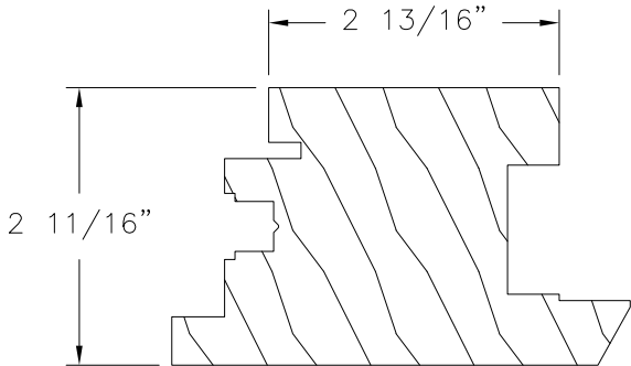
INACTIVE MEETING STILE MAHOGANY
