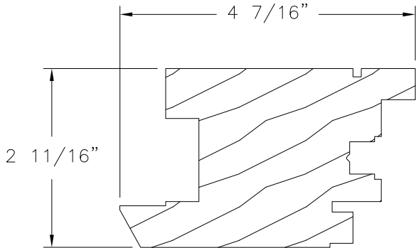
ACTIVE MEETING STILE MAHOGANY
