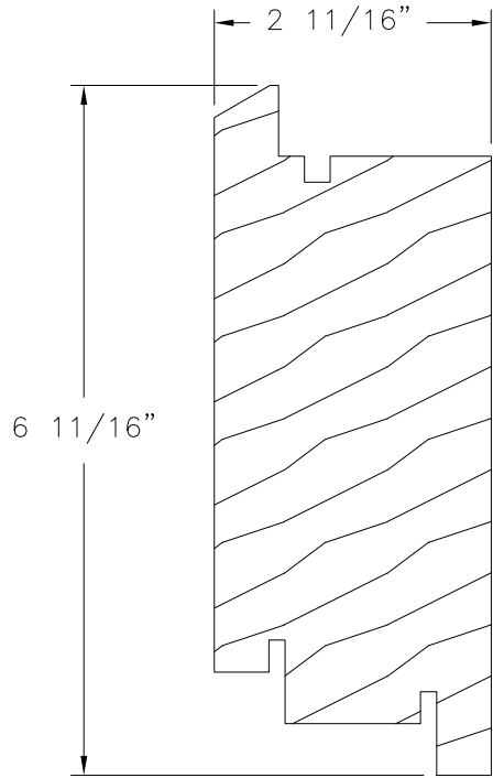
BOTTOM RAIL MAHOGANY
