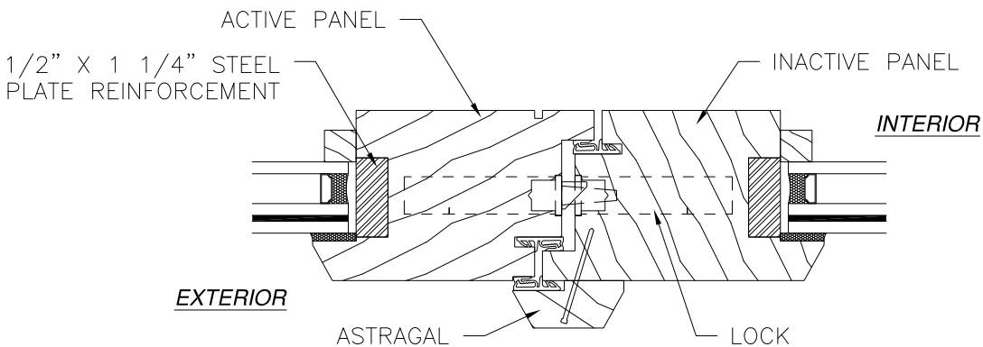
MEETING STILE CONNECTION
