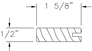
STOP MAHOGANY
