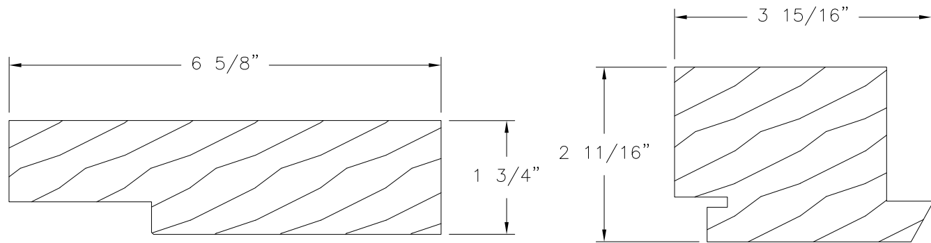
MAIN FRAME MAHOGANY
