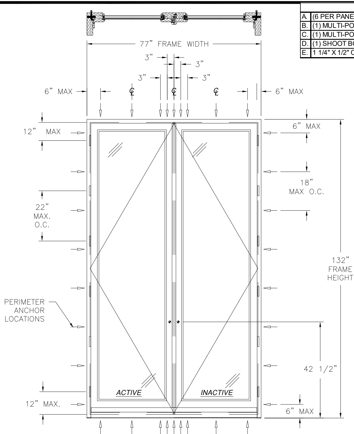
8200 WOOD SIDE-HINGED INSWING DOUBLE DOOR IMPACT HVHZ EXTERIOR VIEW
