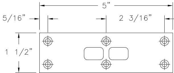
SHOOTBOLT PLATE STAINLESS STEEL
