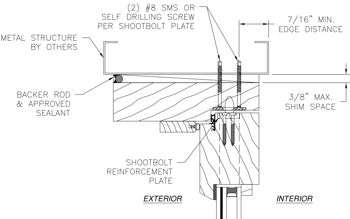
SHOOTBOLT STRIKE INSTALLATION METAL STRUCTURE
