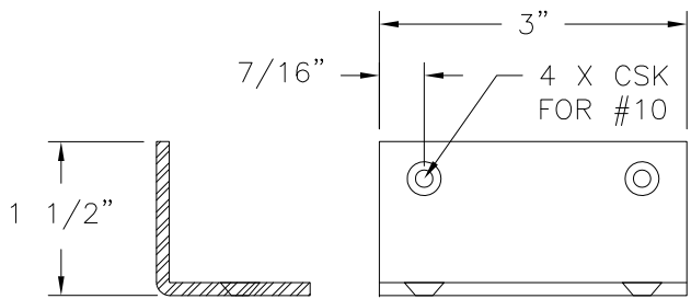
ANGLE 6063-T5 ALUMINUM 1/8" THICK
