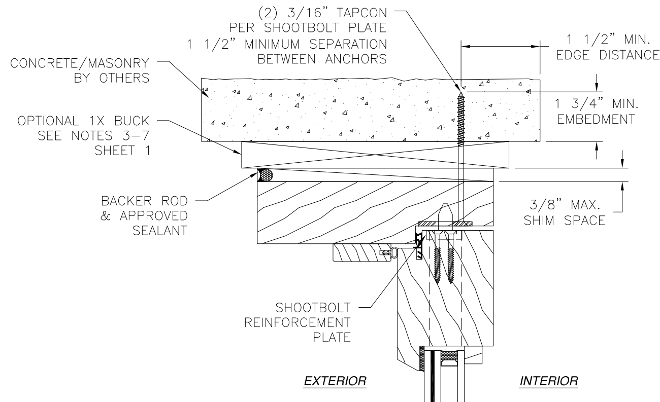
SHOOTBOLT STRIKE INSTALLATION CONCRETE/MASONRY
