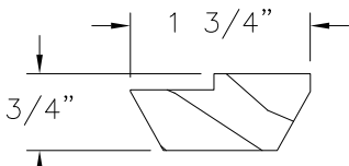
ASTRAGAL MAHOGANY
