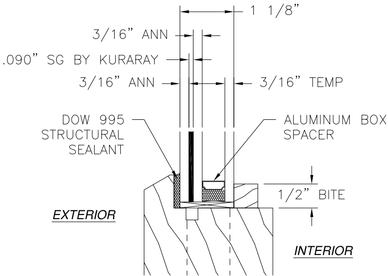
GLASS DETAIL A
