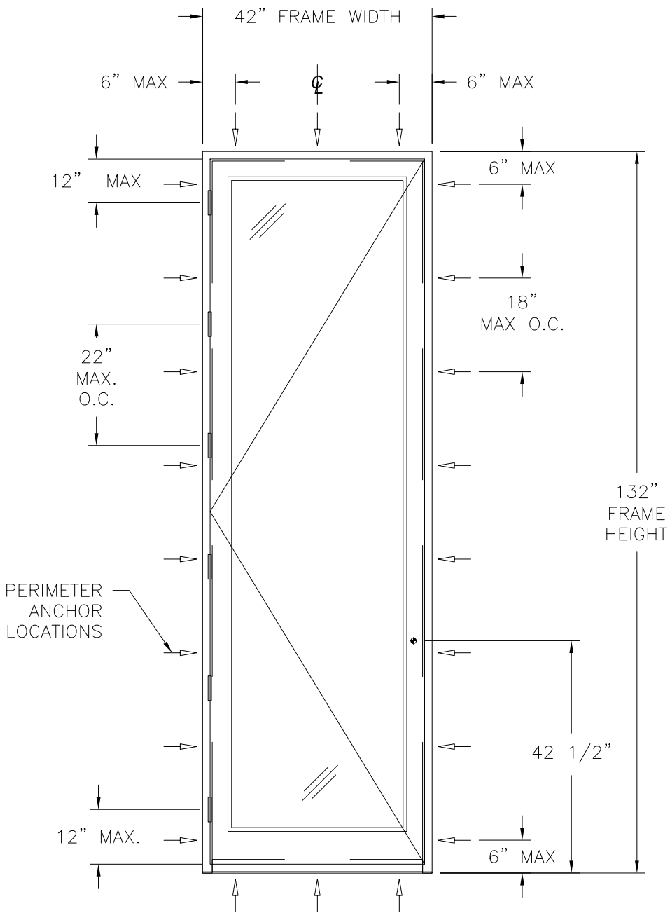
7100 WOOD SIDE-HINGED OUTSWING DOOR IMPACT HVHZ EXTERIOR VIEW
