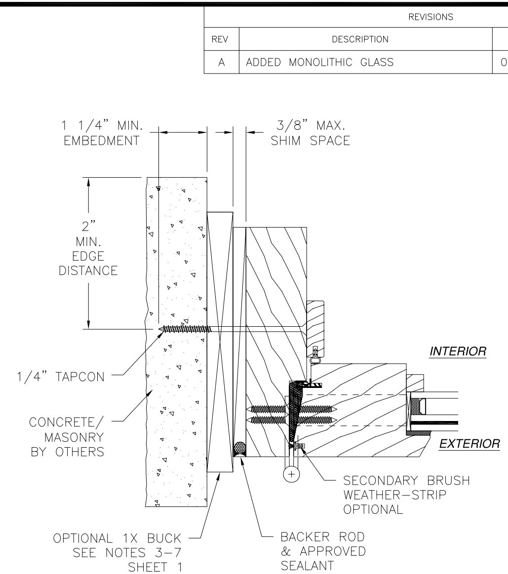
JAMB INSTALLATION DETAIL CONCRETE/MASONRY INSTALLATION
