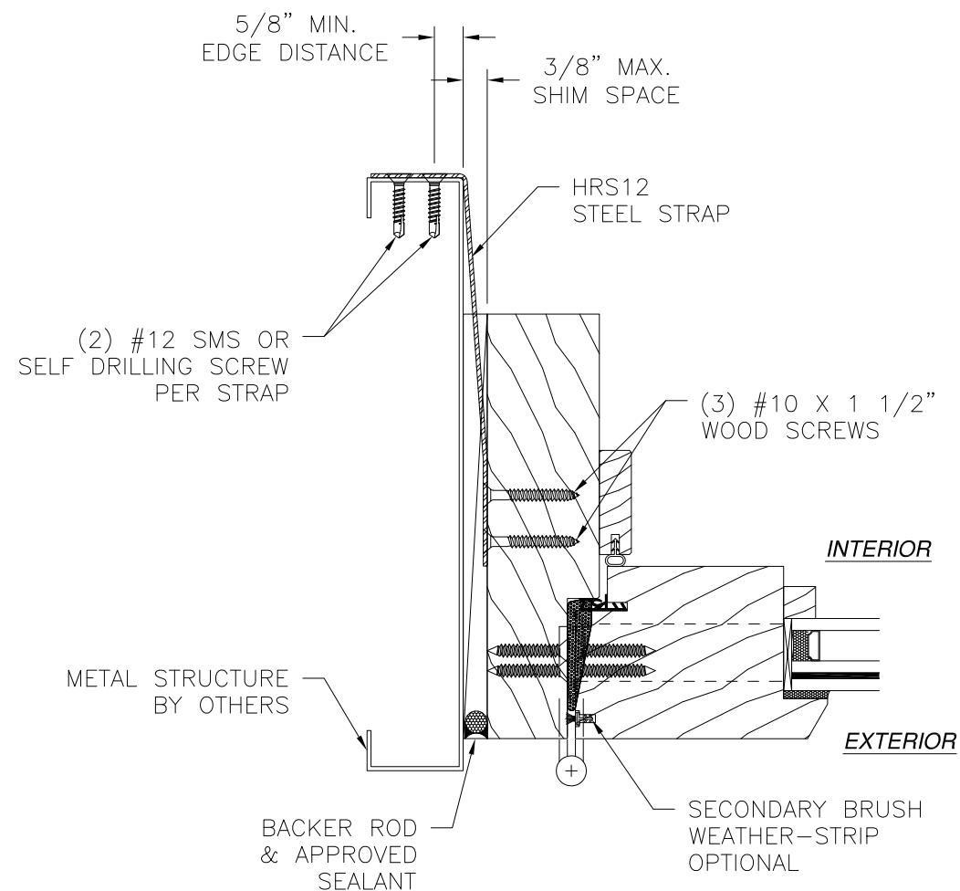
JAMB INSTALLATION DETAIL METAL STRUCTURE INSTALLATION WITH HRS12 STEEL STRAP
