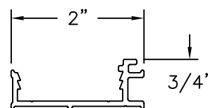
GLAZING CLIP ALUMINUM 6063-T5
