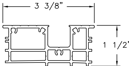
COMMERCIAL FLUSH GUIDE THRESHOLD ALUMINUM 6063-T5
