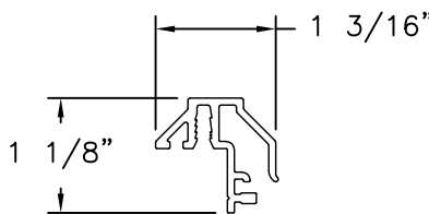
ASTRAGAL ALUMINUM 6063-T5
