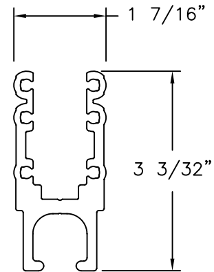
STANDARD CORNER BRACKET ALUMINUM 6063-T5
