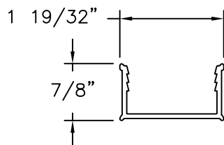
GLAZING CLIP ALUMINUM 6063-T5
