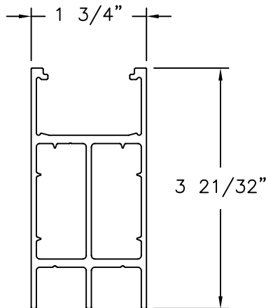
STRENGTHENED RAIL ALUMINUM 6063-T5
