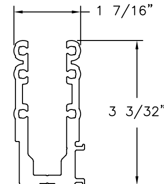
STRENGTHENED CORNER BRACKET ALUMINUM 6063-T5
