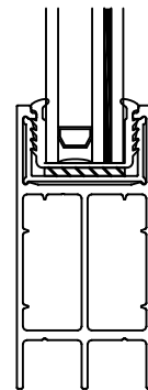
STRENGTHENED RAIL
