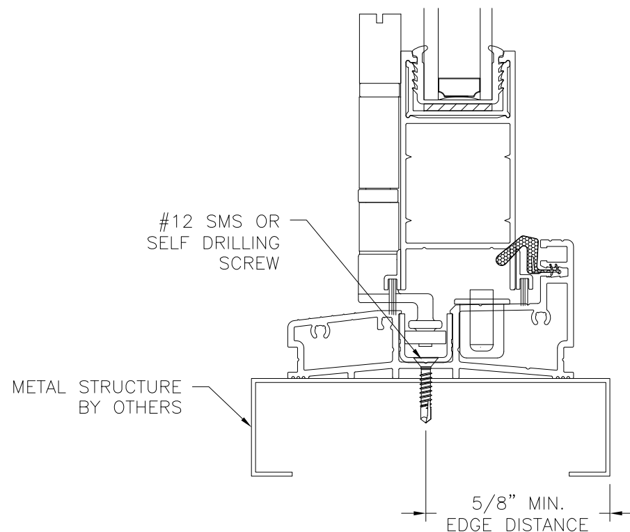
VERTICAL CROSS SECTION METAL STRUCTURE INSTALLATION STANDARD THRESHOLD SHOW SEE SHEET 7 FOR COMMERCIAL FLUSH GUIDE THRESHOLD INSTALLATION
