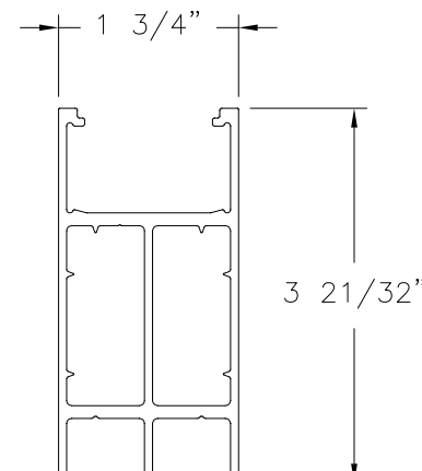
STRENGTHENED RAIL ALUMINUM 6063-T5
