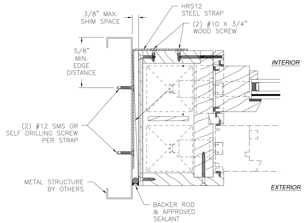
JAMB INSTALLATION DETAIL METAL STRUCTURE INSTALLATION WITH STEEL STRAP
