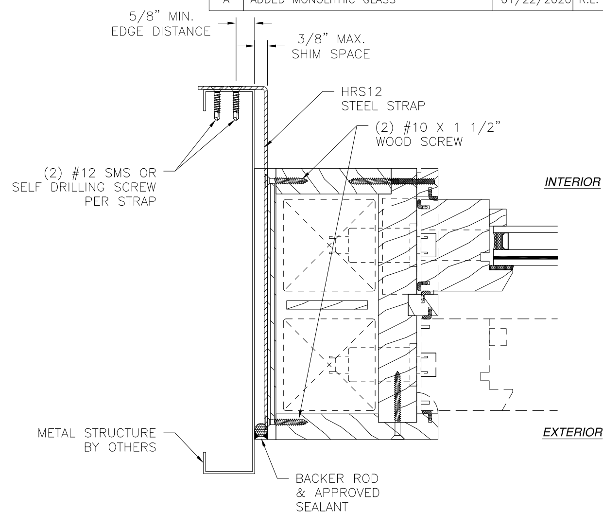
JAMB INSTALLATION DETAIL METAL STRUCTURE INSTALLATION WITH STEEL STRAP
