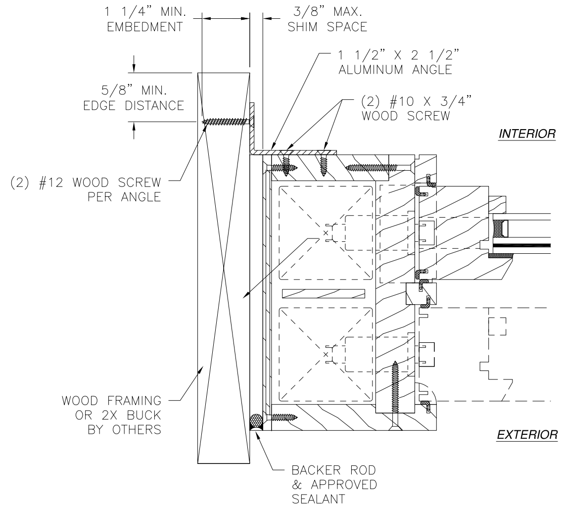
JAMB INSTALLATION DETAIL WOOD FRAMING OR 2X BUCK INSTALLATION WITH ALUMINUM ANGLE
