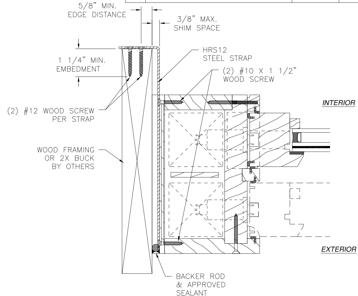
JAMB INSTALLATION DETAIL WOOD FRAMING OR 2X BUCK INSTALLATION WITH STEEL STRAP
