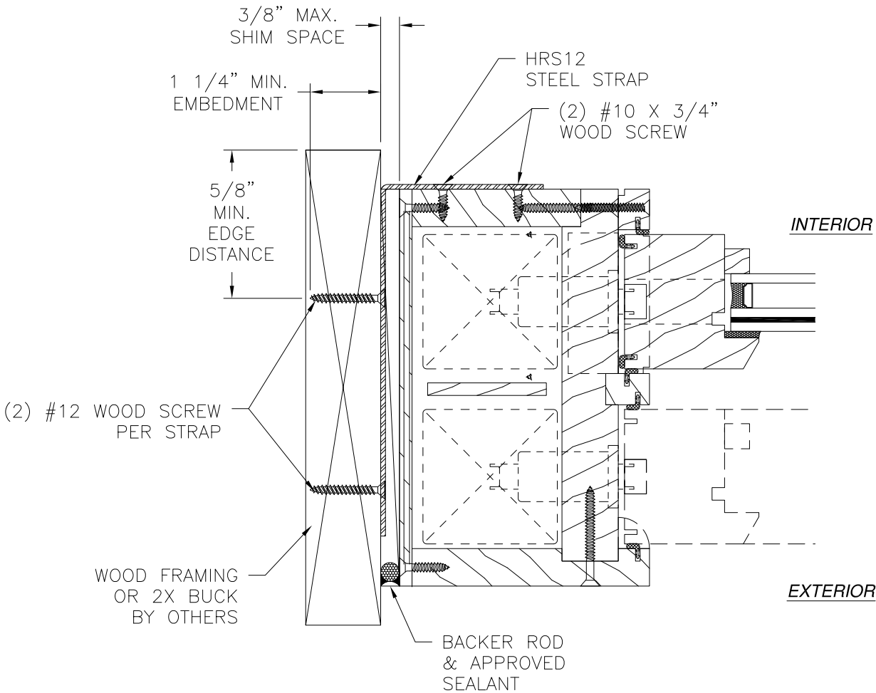
JAMB INSTALLATION DETAIL WOOD FRAMING OR 2X BUCK INSTALLATION WITH STEEL STRAP
