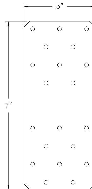
HTP37Z STRAP GALVANIZED STEEL
