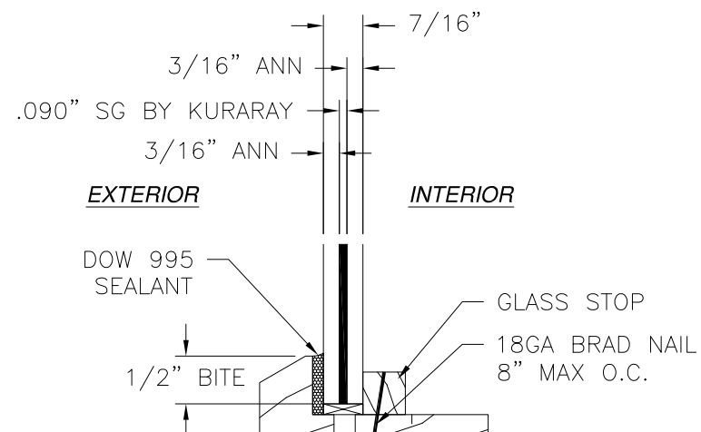
GLAZING DETAIL B
