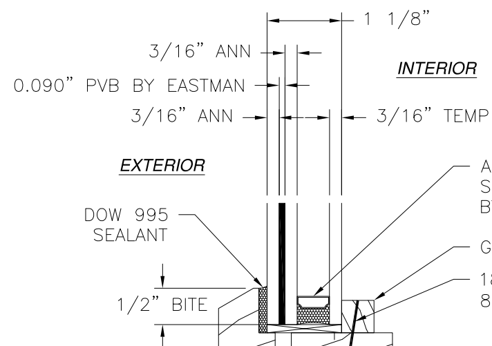
GLAZING DETAIL A
