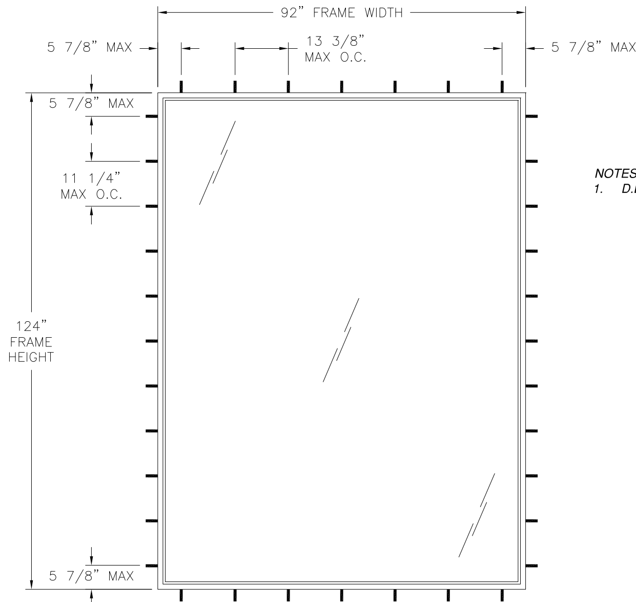
RS-1000I FIXED WINDOW EXTERIOR VIEW
