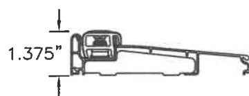
INSWING THRESHOLD
