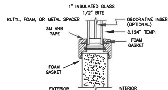
TYPICAL GLAZING DETAIL NON-IMPACT GLASS
