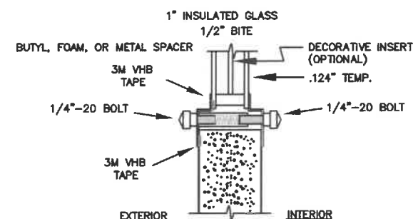
TYPICAL GLAZING DETAIL NON-IMPACT GLASS
