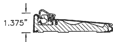
INSWING THRESHOLD
