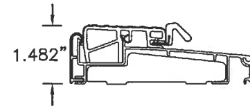
Z-SERIES O/S THRESHOLD
