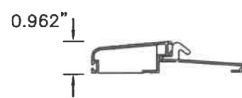
BUMPER O/S THRESHOLD
