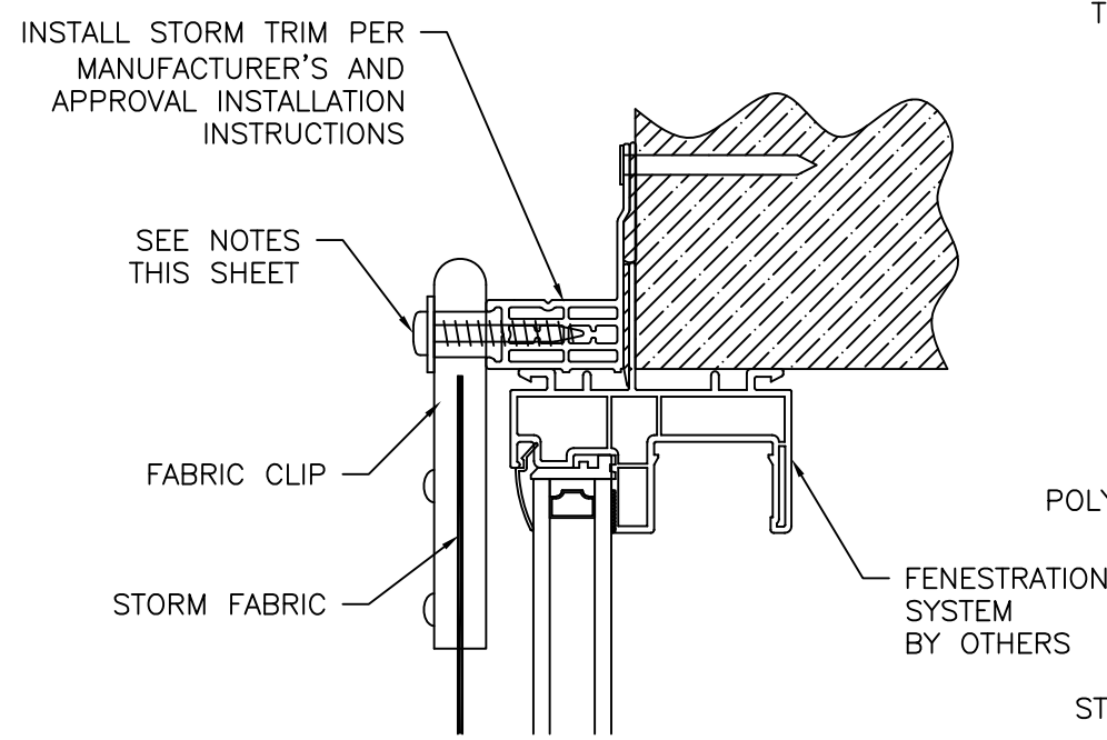
FABRIC INSTALLATION WITH FABRIC CLIP
