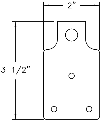
FABRIC CLIP PLASTIC, BY TOWN & COUNTRY
