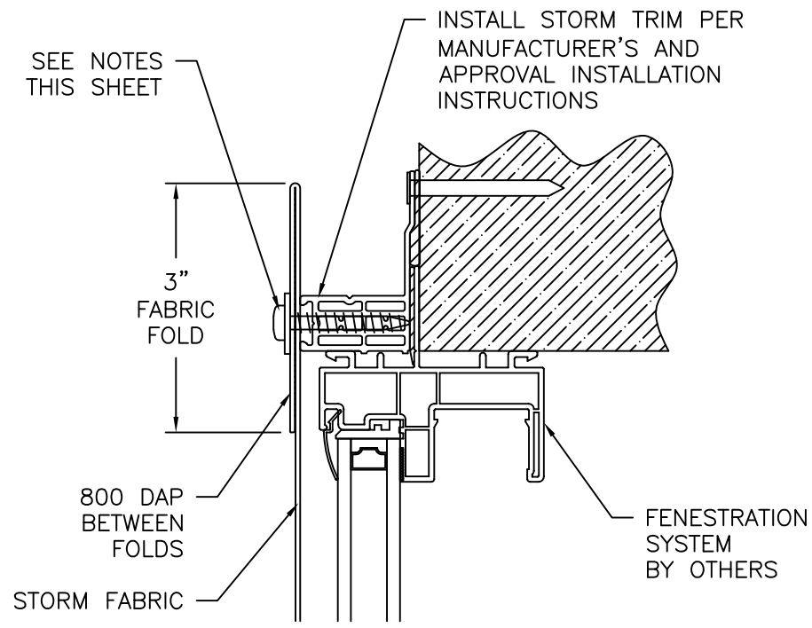
FABRIC INSTALLATION WITH FABRIC FOLDING
