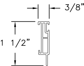
ISOLATOR STRUT (WH811) ALUMINUM 6063-T5
