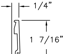
GLAZING STOP (SH884) ALUMINUM 6063-T5
