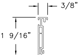
ISOLATOR STRUT (WH809) ALUMINUM 6063-T5
