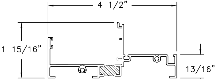
FRAME JAMB (SH814) ALUMINUM 6063-T5
