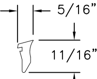
WEDGE GASKET (WH416) EPDM, 70±5 DUROMETER BY TREMCO
