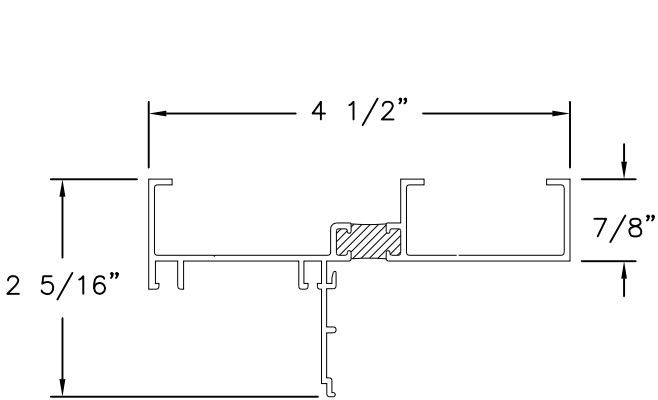
FRAME HEAD (SH812) ALUMINUM 6063-T5
