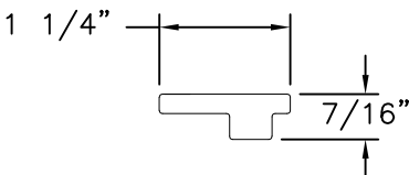
SETTING BLOCK (SB882) 85 DUROMETER BY US ALUMINUM
