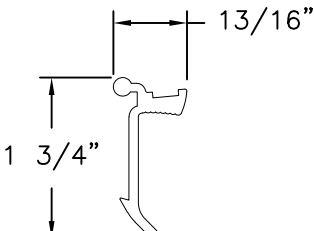
INTERLOCK (SH858) ALUMINUM 6063-T5
