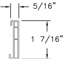
HEAD THERMAL ISOLATOR (WH808) ALUMINUM 6063-T5
