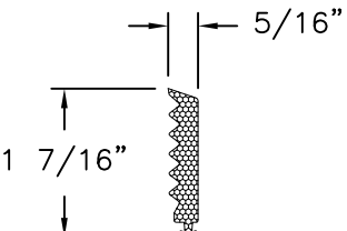
SPONGE GASKET (NP881) EPDM, 70 DUROMETER BY TREMCO
