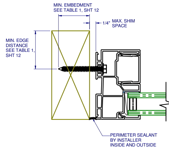
C 10 HORIZONTAL SECTION TYPICAL JAMB ANCHORAGE THRU-FRAME BOX WOOD FRAMING HEAD & SILL DETAILS SIMILAR
