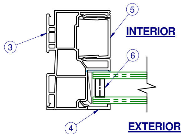
SECTION B - B ALT. BOX FRAME
