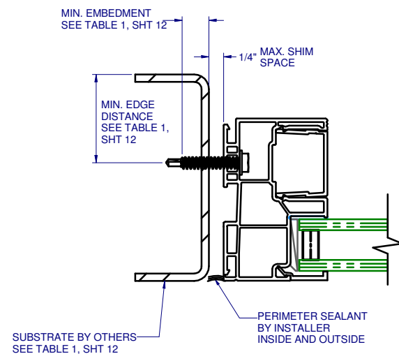
D 10 HORIZONTAL SECTION TYPICAL JAMB ANCHORAGE THRU-FRAME BOX FRAME METAL FRAMING HEAD & SILL DETAILS SIMILAR
