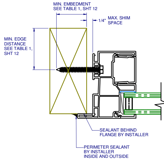
C 9 HORIZONTAL SECTION TYPICAL JAMB ANCHORAGE THRU-FRAME FLANGE WOOD FRAMING HEAD & SILL DETAILS SIMILAR
