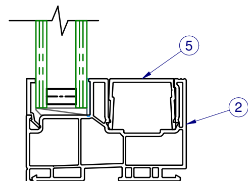
SECTION A - A FLANGE FRAME
