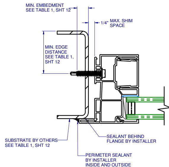
D 9 HORIZONTAL SECTION TYPICAL JAMB ANCHORAGE THRU-FRAME FLANGE METAL FRAMING HEAD & SILL DETAILS SIMILAR
