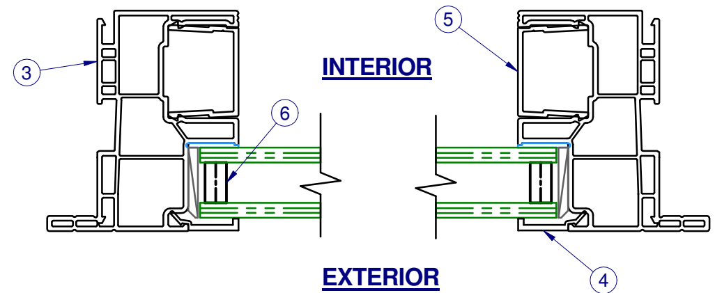
SECTION B - B FLANGE FRAME
