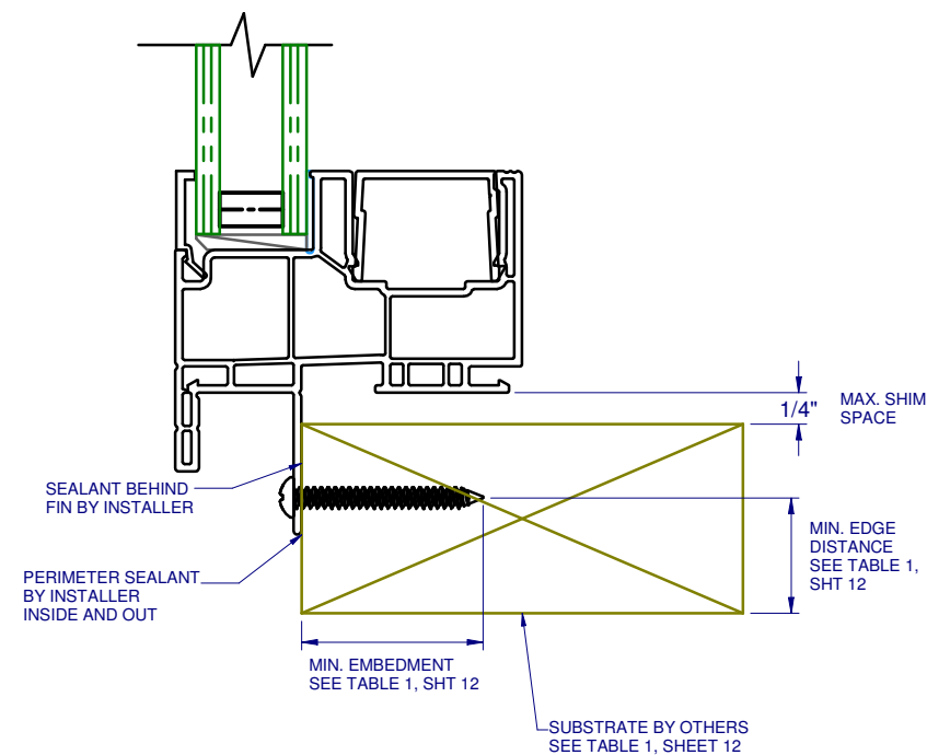
A 11 VERTICAL SECTION TYPICAL SILL & HEAD ANCHORAGE THRU-FIN FIN / FLANGE WOOD FRAMING
