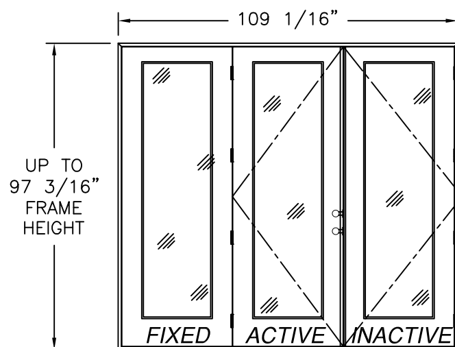
DOUBLE W/SIDELITE (OXX, XXO) EXTERIOR VIEW FULL LITE SHOWN, 3/4 & 1/2 LITE SIMILAR
