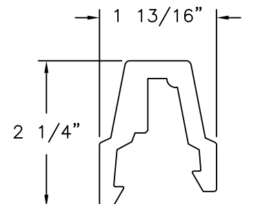
MULLION COVER (B) FOAM PVC
