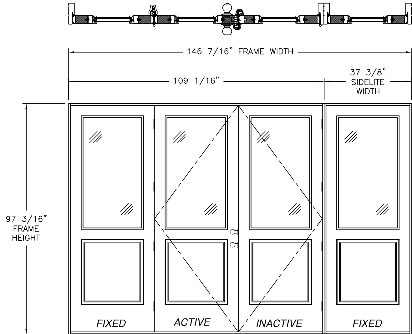
SERIES PATIO DOOR LITE OUTSWING (OXX/O) 8' UNIT EXTERIOR VIEW 1/2 LITE PANELS REFER TO SHEET 5 FOR HARDWARE AND NOTES
