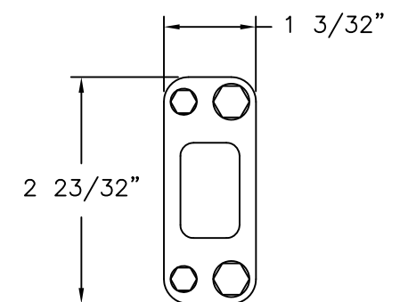
DEADBOLT KEEPER STAINLESS STEEL (KWIKSET 980)
