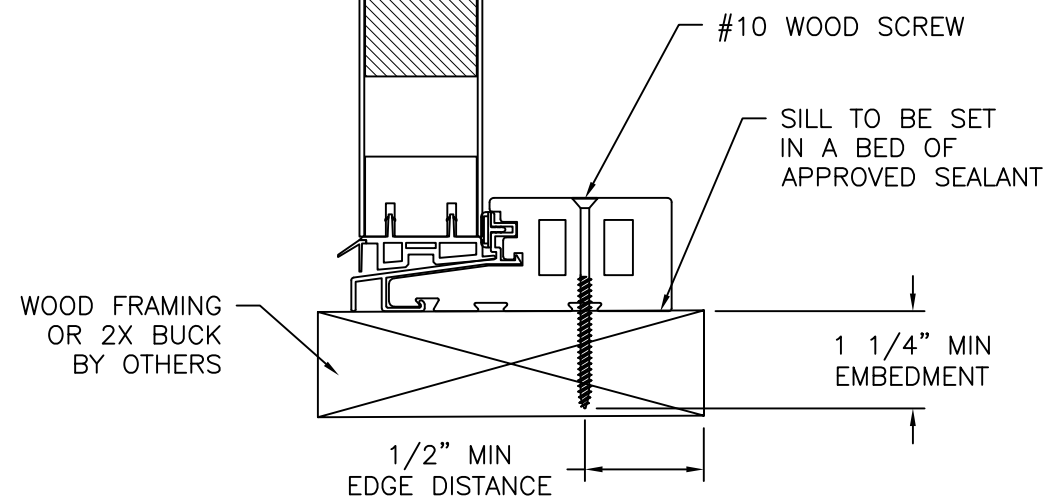
SIDELITE DOOR INSTALLATION DETAIL 2X BUCK/WOOD FRAMING INSTALLATION FULL LITE SHOWN, 3/4 & 1/2 LITE SIMILAR
