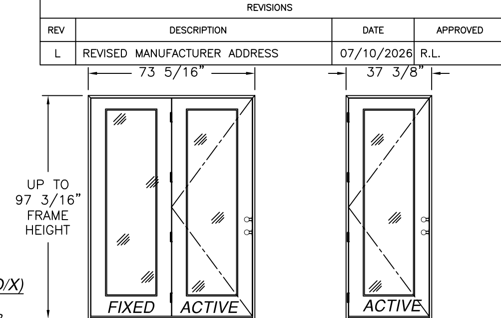
SINGLE (X) EXTERIOR VIEW FULL LITE SHOWN, 3/4 & 1/2 LITE SIMILAR
