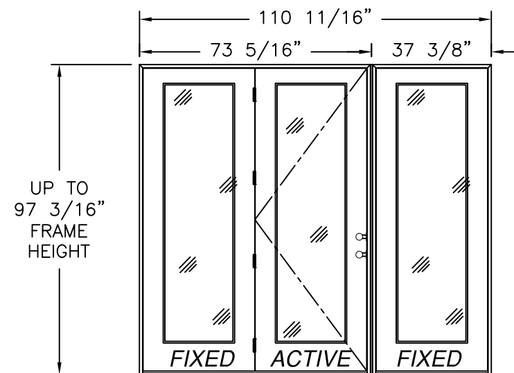
SINGLE W/SIDELITE MULL. (OX/O, O/XO)
