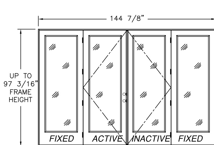
DOUBLE W/SIDELITE (OXXO)
