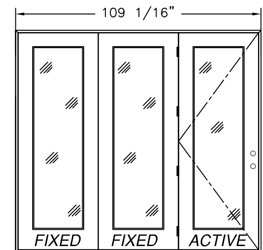
SINGLE W/SIDELITES (OOX, XOO)
