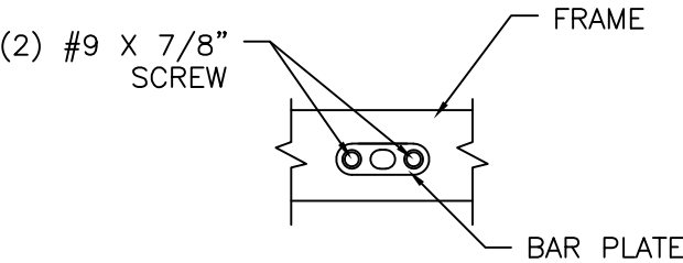
DRIVE BAR PLATE DETAIL
