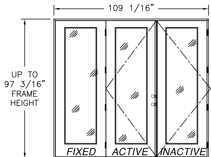
DOUBLE W/SIDELITE (OXX, XXO)
