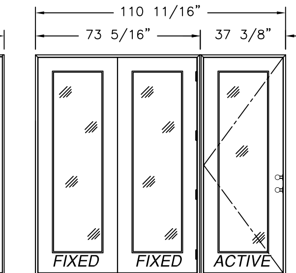
SINGLE W/SIDELITES MULL. (OO/X)
