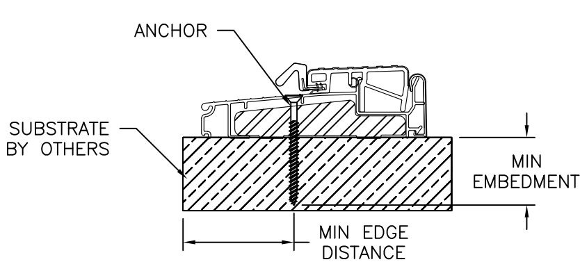
ENDURA THRESHOLD ZOB4565
