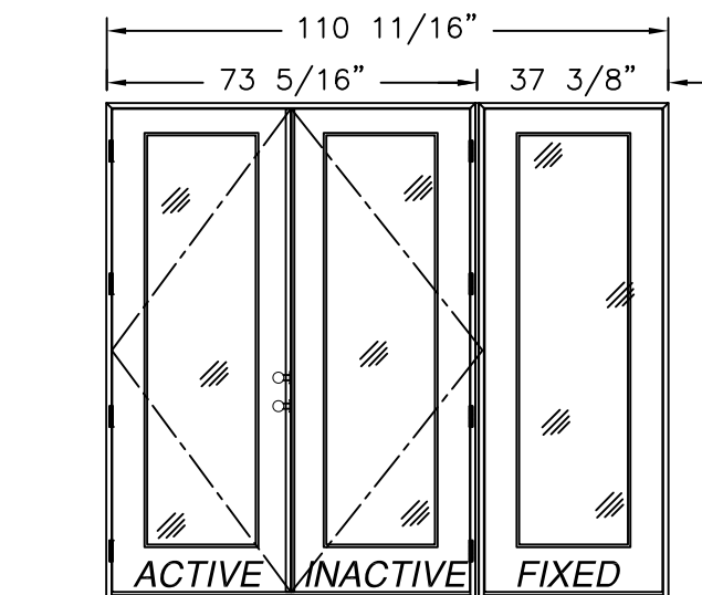
DOUBLE W/SIDELITE MULL. (XX/O, O/XX)
