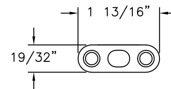
DRIVE BAR PLATE STAINLESS STEEL
