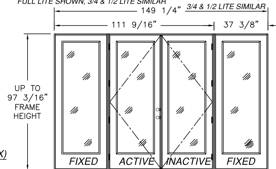
DOUBLE W/SIDELITES MULL. (O/XX/O)
