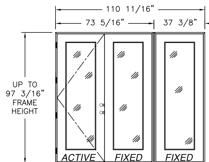
SINGLE W/SIDELITES MULL. (XO/O, O/OX)
