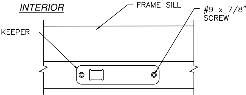
INTERIOR SILL KEEPER DETAIL
