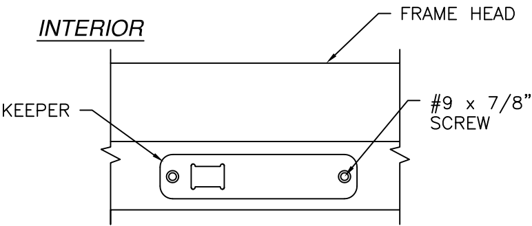
INTERIOR HEAD KEEPER DETAIL
