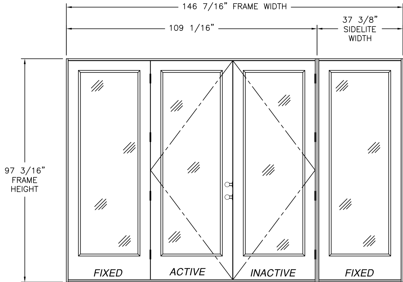
SERIES SLPS OUT-SWING SIDE-HINGED DOOR W/SIDELITES (OXX/O) 8' UNIT EXTERIOR VIEW FULL LITE PANELS REFER TO SHEET 5 FOR HARDWARE AND NOTES
