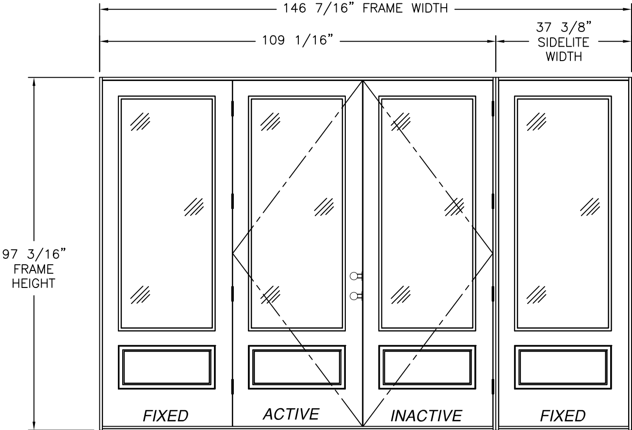
SERIES SLPS OUT-SWING SIDE-HINGED DOOR W/SIDELITES (OXX/O) 8' UNIT EXTERIOR VIEW 3/4 LITE PANELS REFER TO SHEET 5 FOR HARDWARE AND NOTES
