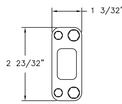
DEADBOLT KEEPER STAINLESS STEEL (KWIKSET 980)
