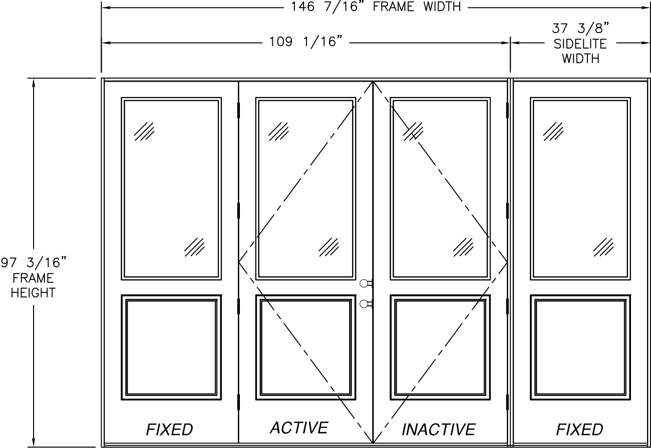
SERIES SLPS OUT-SWING SIDE-HINGED DOOR W/SIDELITES (OXX/O) 8' UNIT EXTERIOR VIEW 1/2 LITE PANELS REFER TO SHEET 5 FOR HARDWARE AND NOTES
