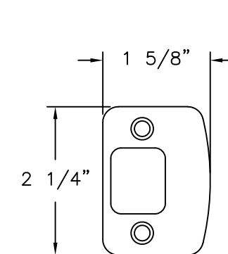
LATCH KEEPER STAINLESS STEEL
