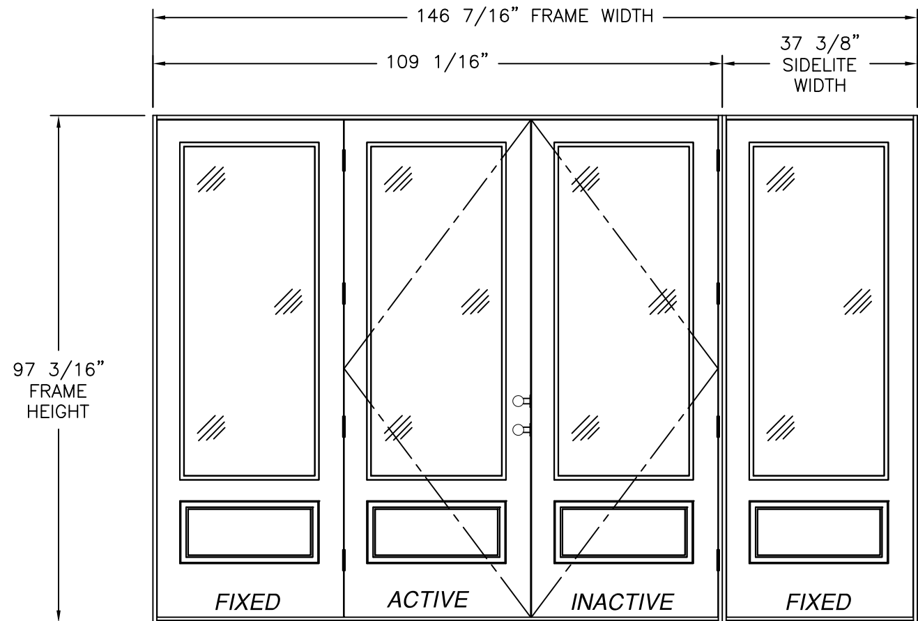
SERIES SLPS OUT-SWING SIDE-HINGED DOOR W/SIDELITES (OXX/O)
