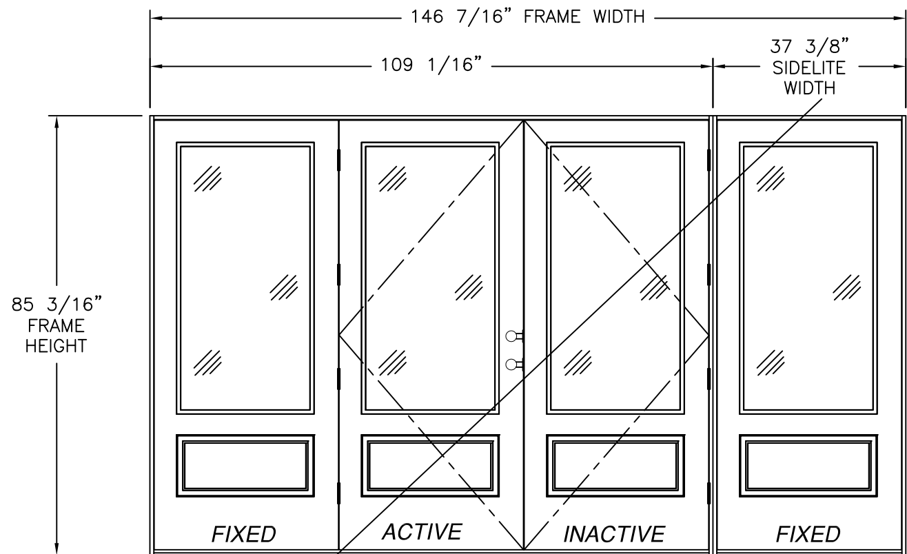
SERIES SLPS OUT-SWING SIDE-HINGED DOOR W/SIDELITES (OXX/O)
