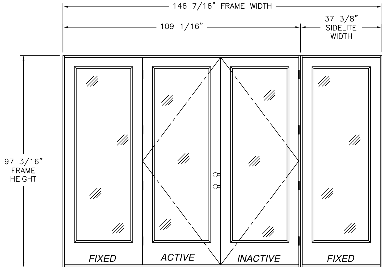
SERIES SLPS OUT-SWING SIDE-HINGED DOOR W/SIDELITES (OXX/O)
