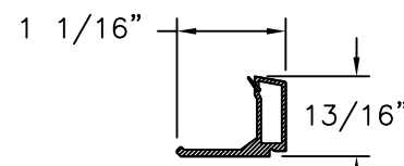
GLAZING BEAD FOAM PVC
