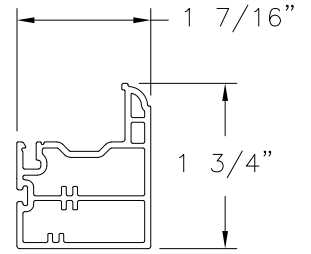
LOCK RAIL VINYL PVC (10005521)
