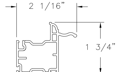
BOTTOM RAIL VINYL PVC (10005526)
