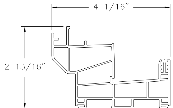
SILL FRAME VINYL PVC (10005084)
