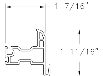
KEEPER RAIL VINYL PVC (10005522)
