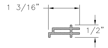
LOCK RAIL REINFORCEMENT EXTRUDED ALUMINUM (10006201)
