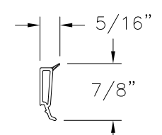
GLAZING BEAD VINYL PVC (10005470)
