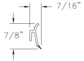
INTERLOCK GLAZING BEAD VINYL PVC (10005551)
