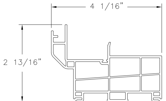
HEAD FRAME VINYL PVC (10005085)
