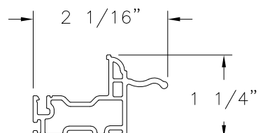
TOP RAIL VINYL PVC (10005525)
