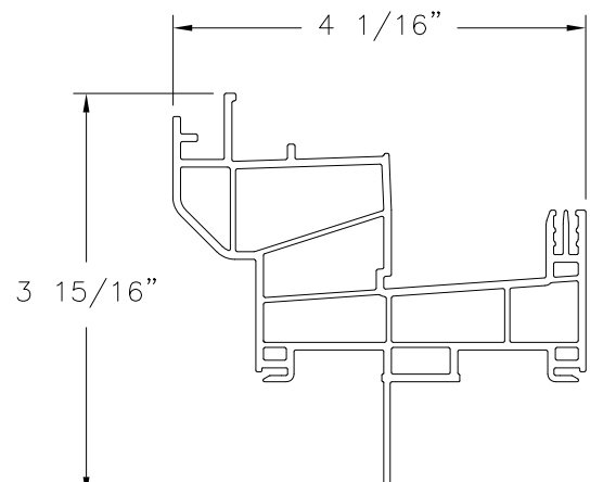
SILL FRAME FIN INSTALLATION VINYL PVC (10005084)
