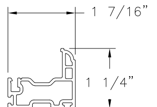
TOP STILE VINYL PVC (10005524)
