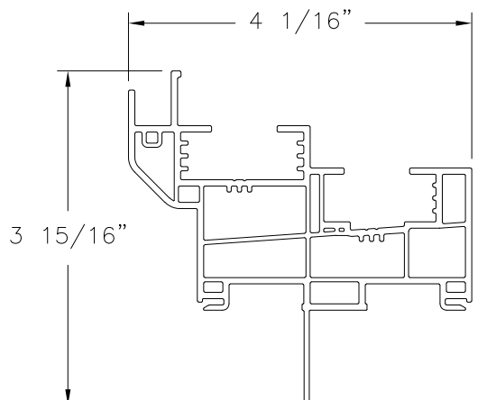
JAMB FRAME FIN INSTALLATION VINYL PVC (10005083)
