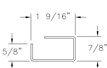
⑫ SASH REINFORCEMENT STEEL (RF-S019)
