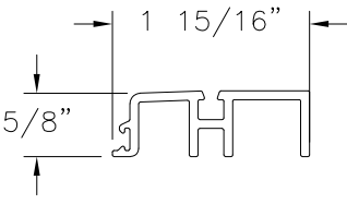
⑤ SILL ADAPTOR RIGID PVC (RH-S018)
