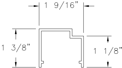
③② SASH REINFORCEMENT ALUMINUM 6063-T5 (S-15463)
