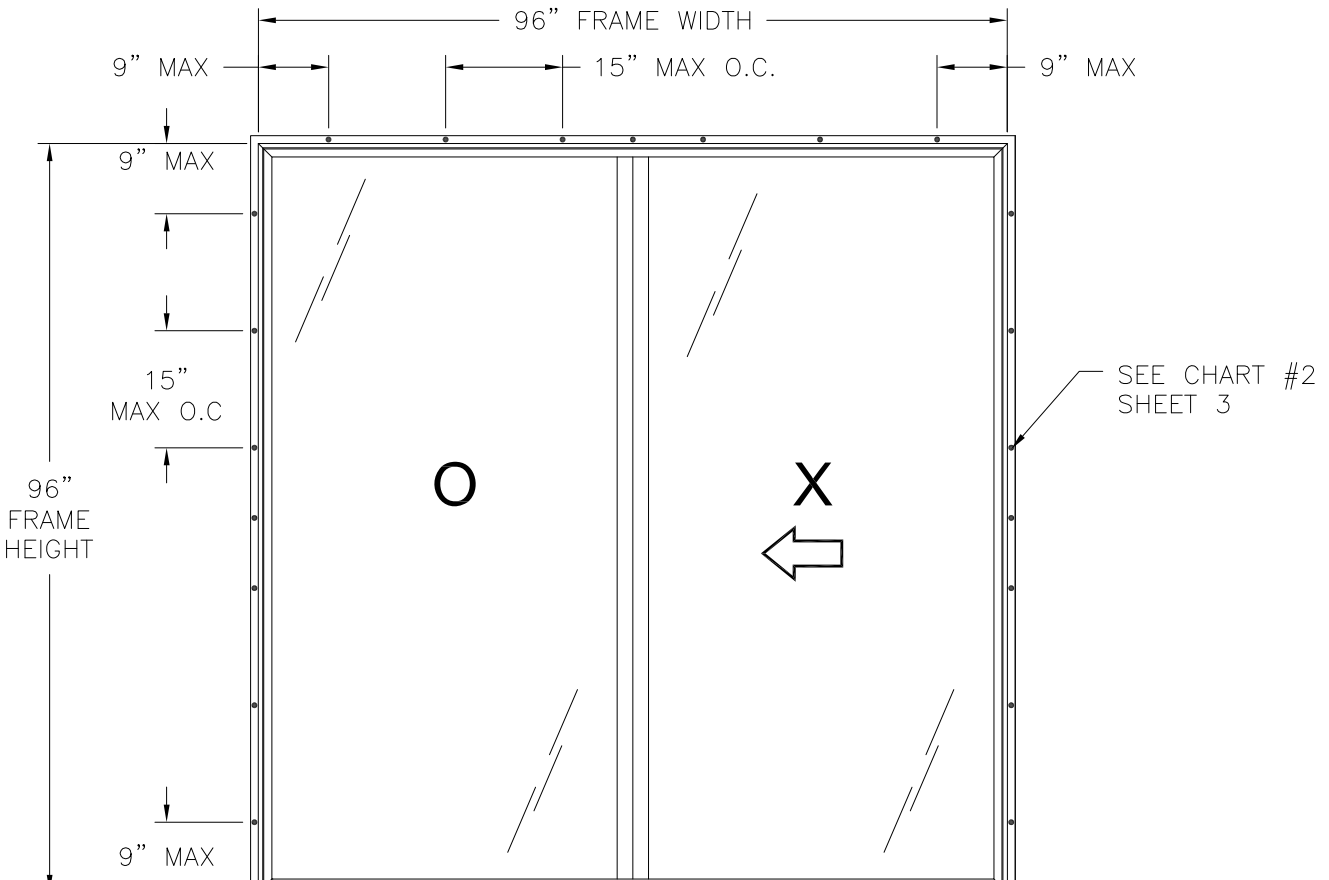
SERIES SI4100V VINYL SLIDING GLASS DOOR OX & XO EXTERIOR VIEW FIN INSTALLATION
