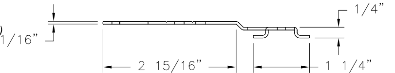
INSTALLATION STRIP GALVANIZED STEEL G60
