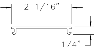
⑪ SASH STOP RIGID PVC (RH-S029)
