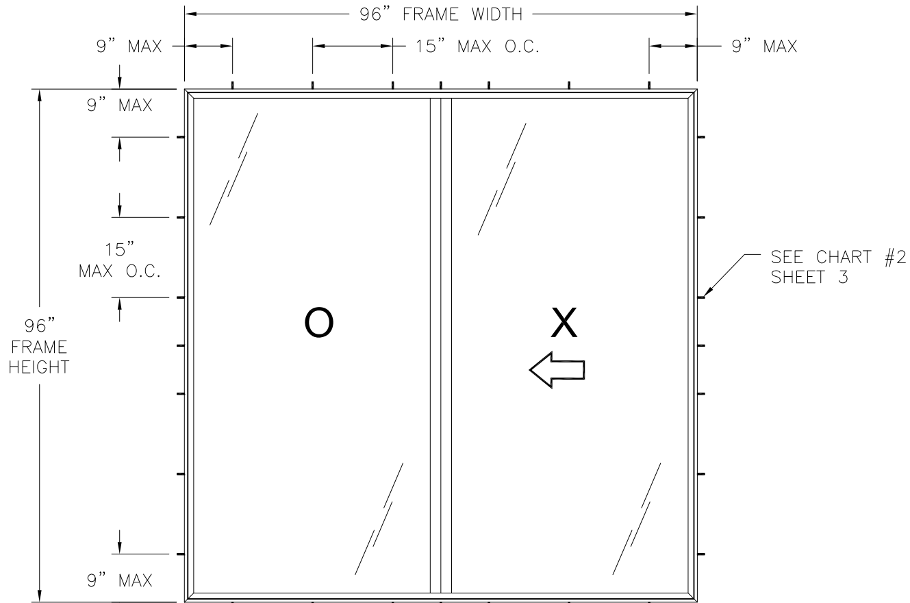
SERIES SI4100V VINYL SLIDING GLASS DOOR OX & XO EXTERIOR VIEW FRAME AND STRIP INSTALLATION
