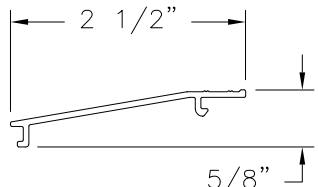
⑧ SEUIL SILL EXTRUDED ALUMINUM (S-14307)
