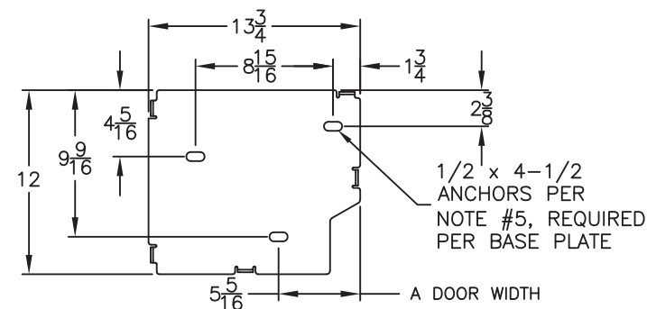
DETAIL G SIDE COLUMN BASE MOUNTING
