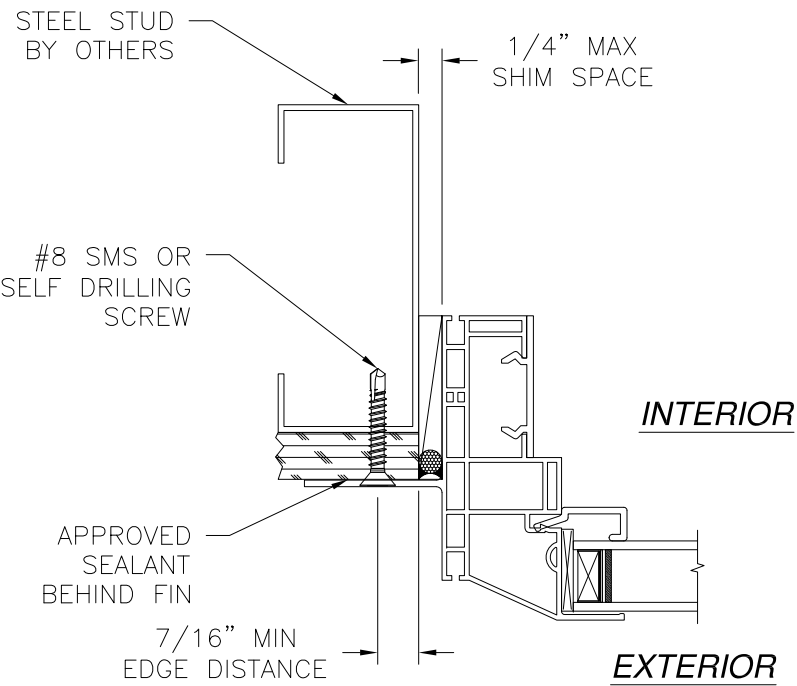
JAMB INSTALLATION DETAIL STEEL STUD INSTALLATION
