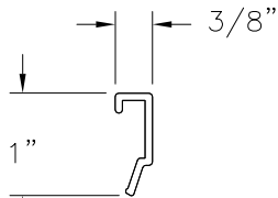
GLAZING BEAD PVC (V-819)
