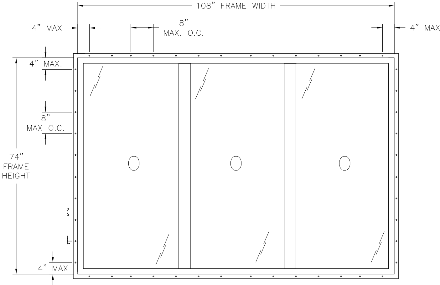
SERIES 3540 PW CHS TRIPLE FIXED WINDOW EXTERIOR VIEW
