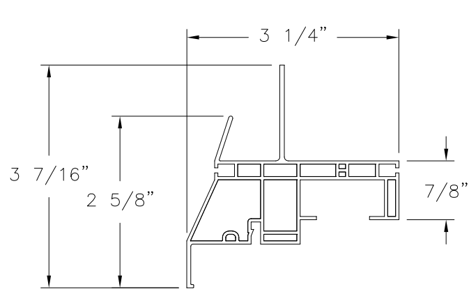
MAIN FRAME WITH "J" CHANNEL PVC (V-538)
