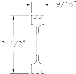
INTERMEDIATE JAMB REINFORCEMENT ALUMINUM 6063-T5 (M-1994)
