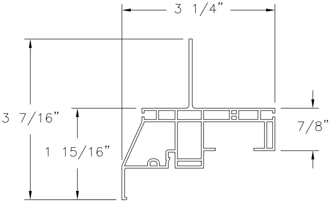
MAIN FRAME WITHOUT "J" CHANNEL PVC (V-634)
