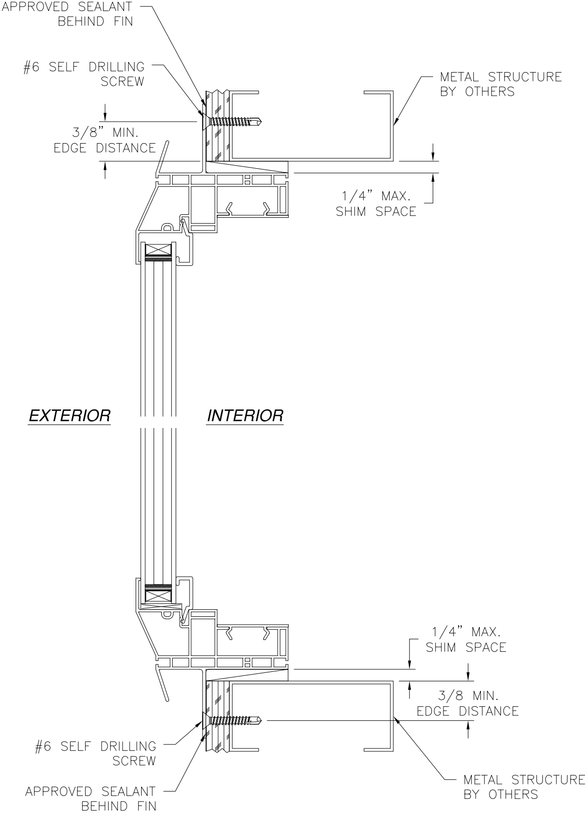
VERTICAL CROSS SECTION METAL STRUCTURE INSTALLATION
