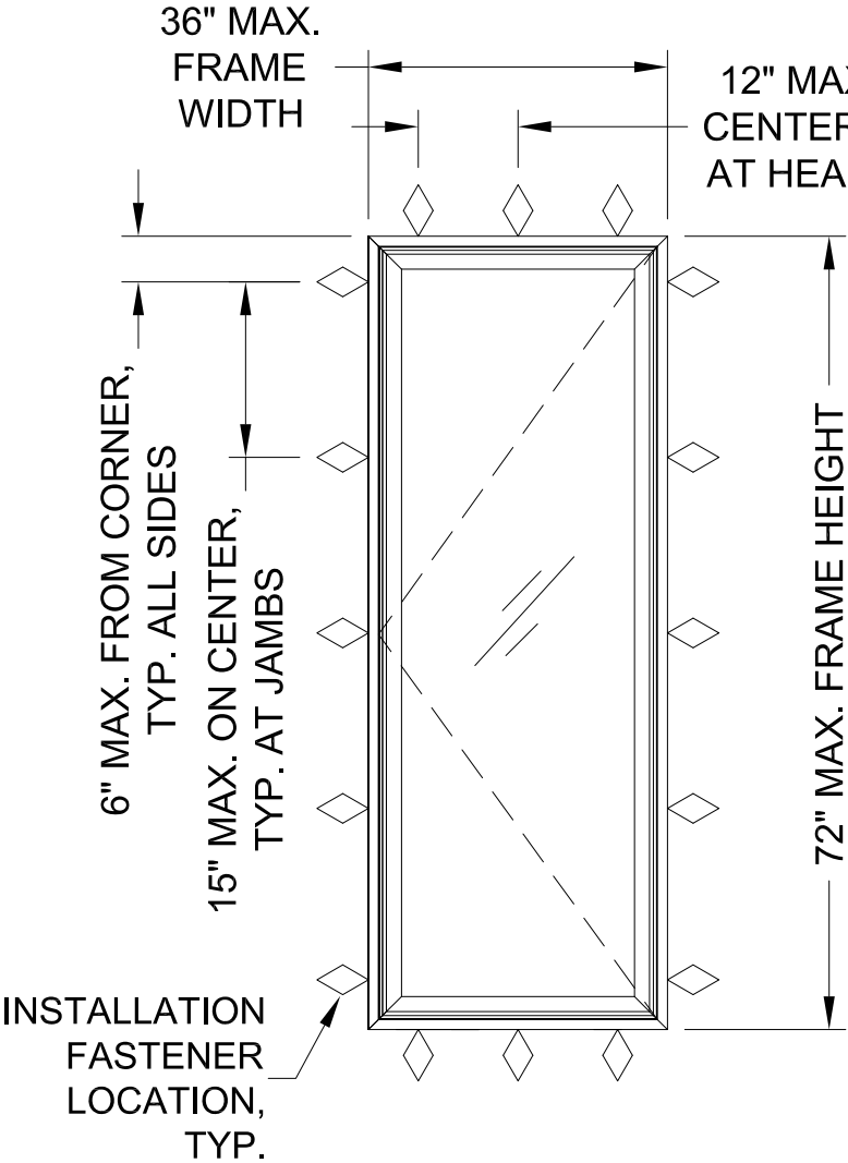
FLANGE / EQUAL LEG ELEVATION SEE DETAILS SHEETS 2
