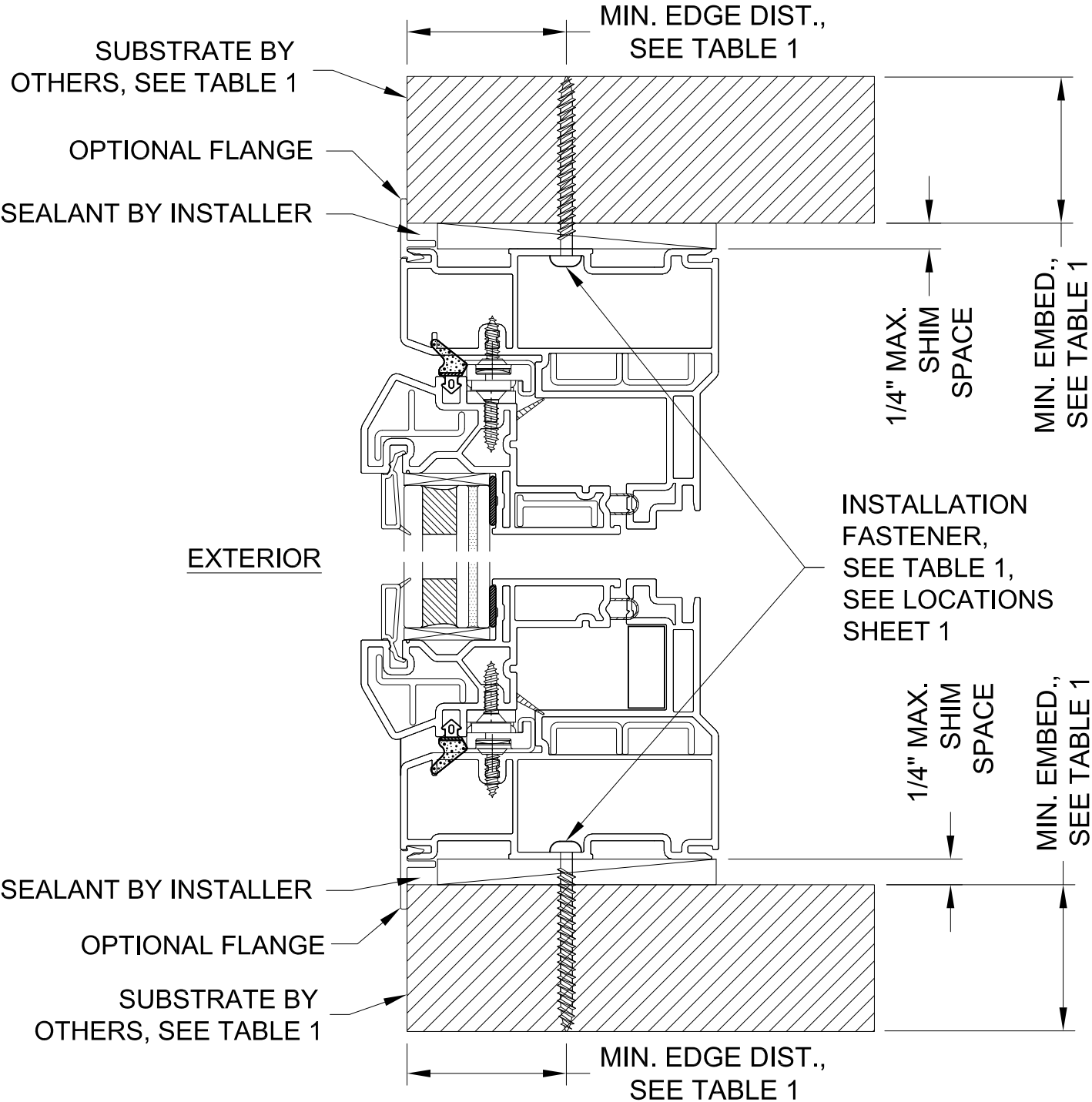
TYPICAL FLANGE / EQUAL LEG FRAME VERTICAL SECTION
