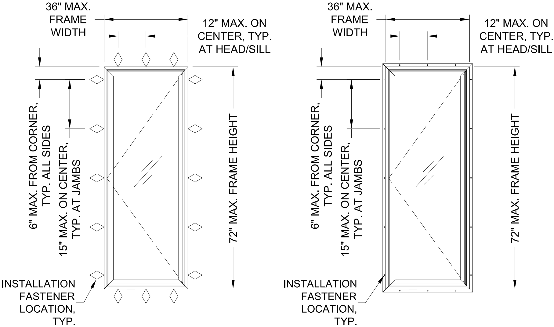
FLANGE / EQUAL LEG ELEVATION SEE DETAILS SHEETS 2
