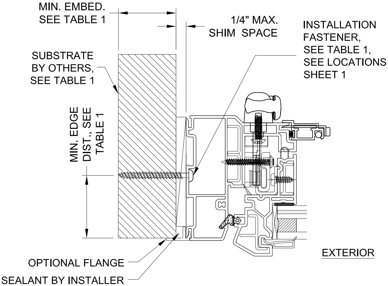
TYPICAL FLANGE / EQUAL LEG JAMB HORIZONTAL SECTION LOCK JAMB AND HINGE JAMB SIM. INSTALLATION
