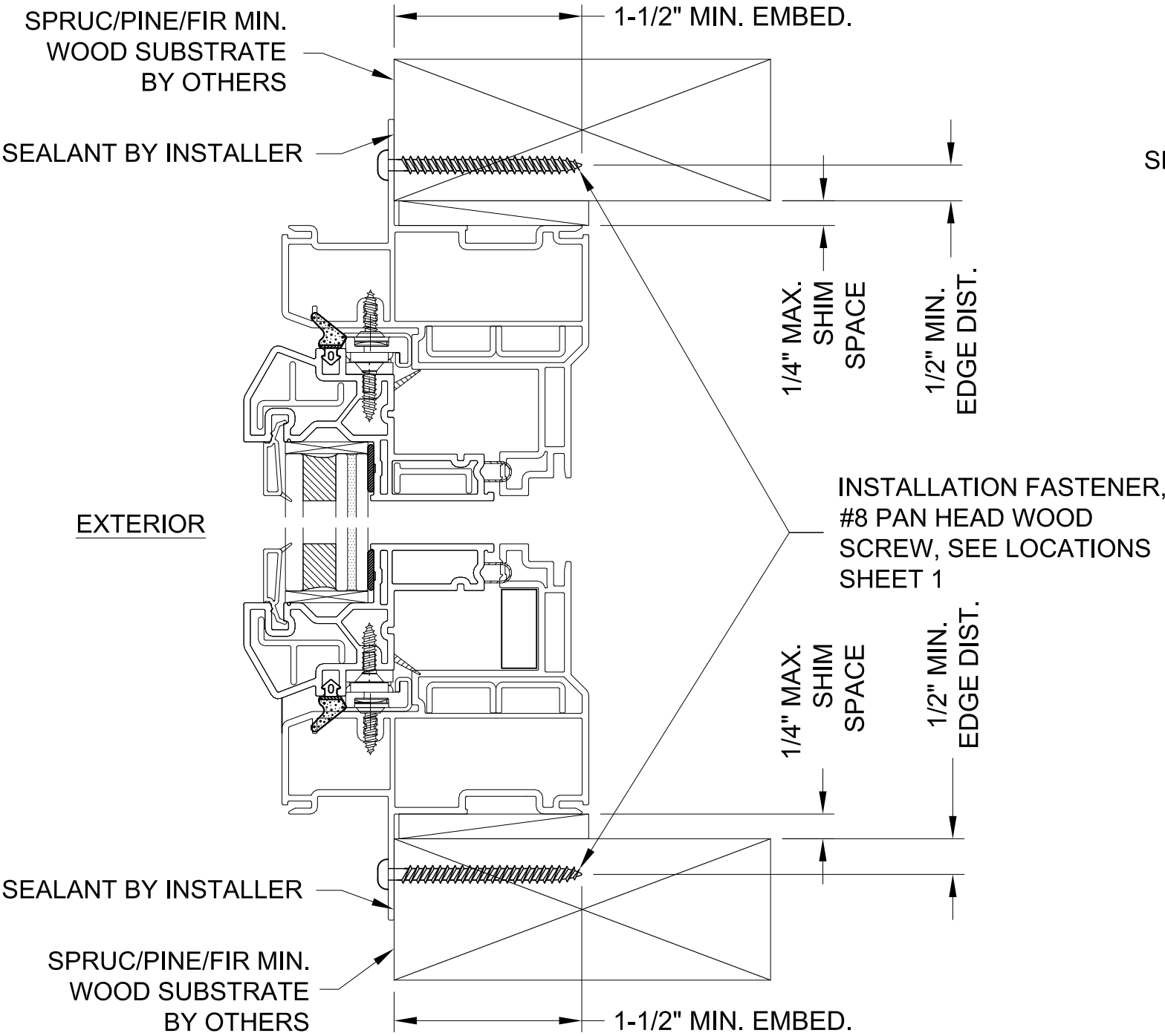
TYPICAL FIN FRAME VERTICAL SECTION
