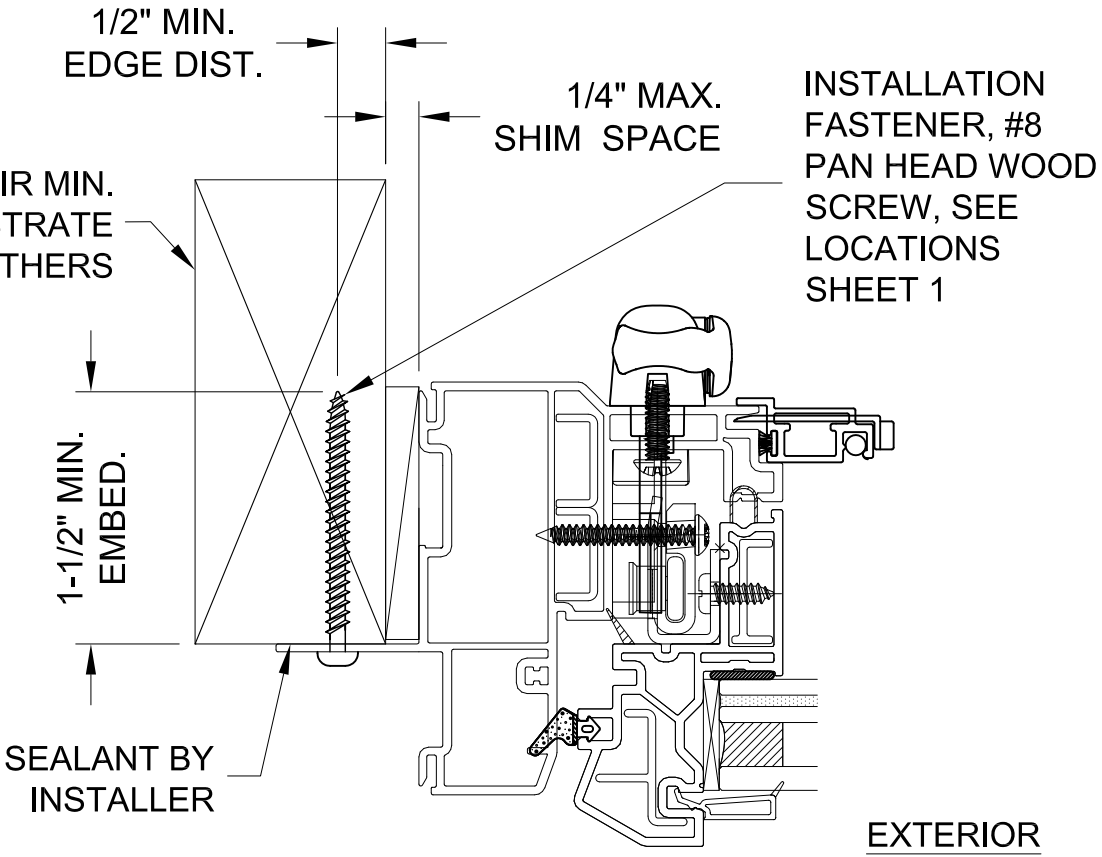
TYPICAL FIN JAMB HORIZONTAL SECTION LOCK JAMB AND HINGE JAMB SIM. INSTALLATION
