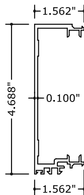
E5 VERTICAL MULLION MALE
