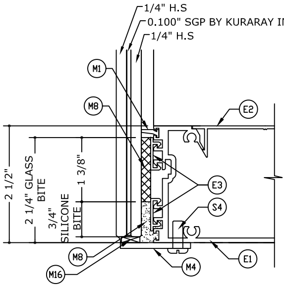
GLAZING DETAIL - GLASS TYPE 'A' SINGLE SPAN (LARGE & SMALL MISSILE )
