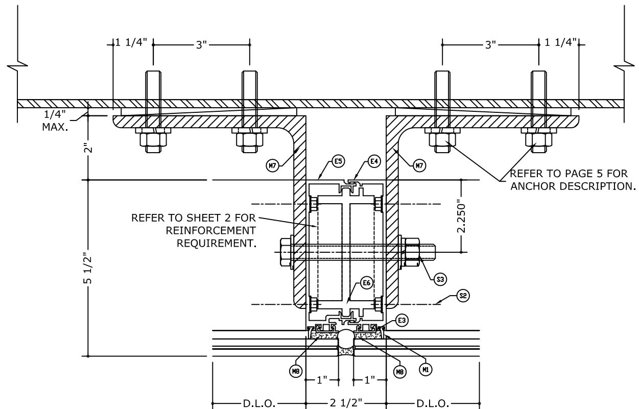
5.1 CONDITION AT MULLION BOTTOM N.T.S
