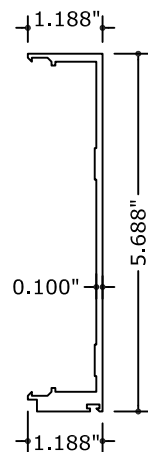
E9 VERTICAL MULLION FEMALE
