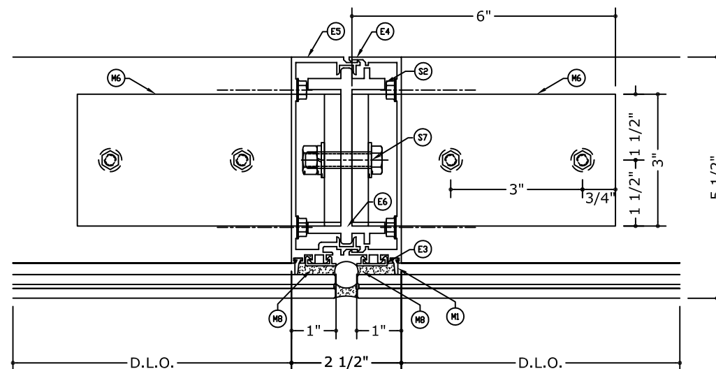
5 CONDITION AT MULLION BOTTOM N.T.S
