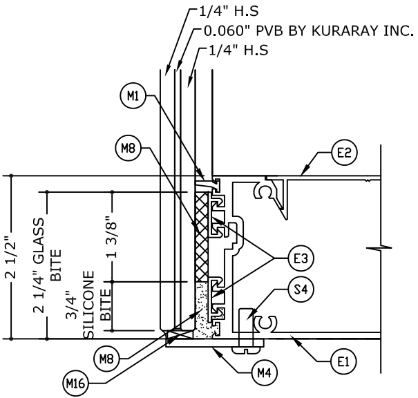
GLAZING DETAIL - GLASS TYPE 'C' TWIN SPAN (SMALL MISSILE )
