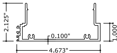
E8 EXPANSION JOINT TOP
