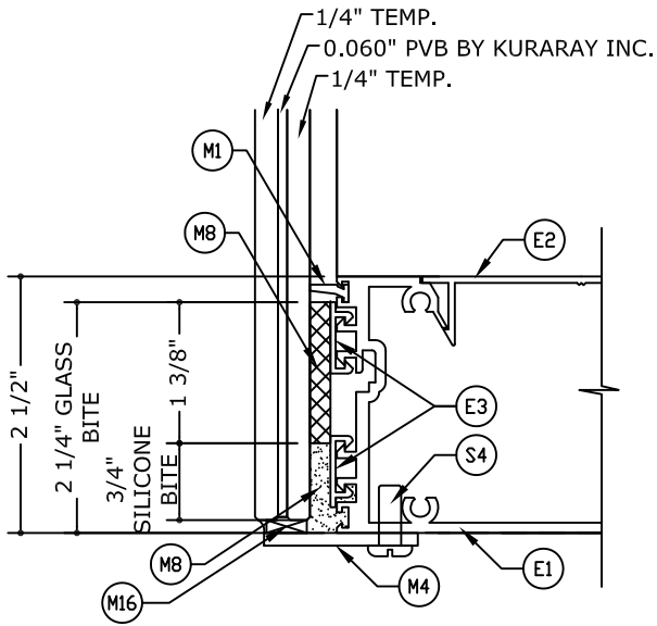
GLAZING DETAIL - GLASS TYPE 'D' TWIN SPAN (SMALL MISSILE )
