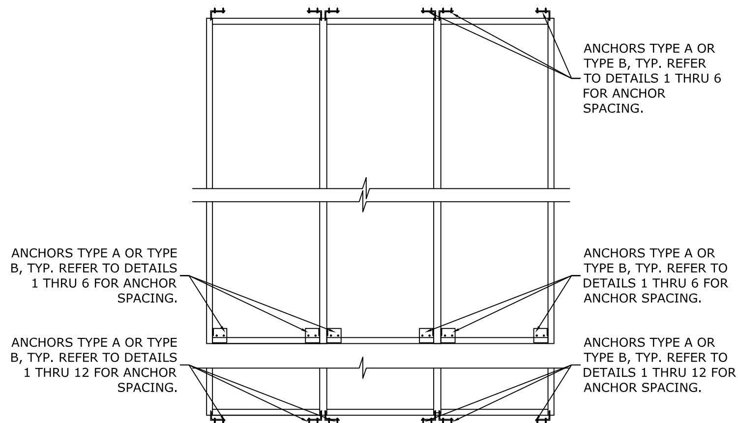
TYPICAL ANCHOR LAYOUT
