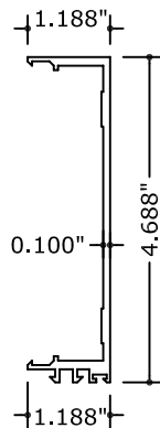
E4 VERTICAL MULLION FEMALE
