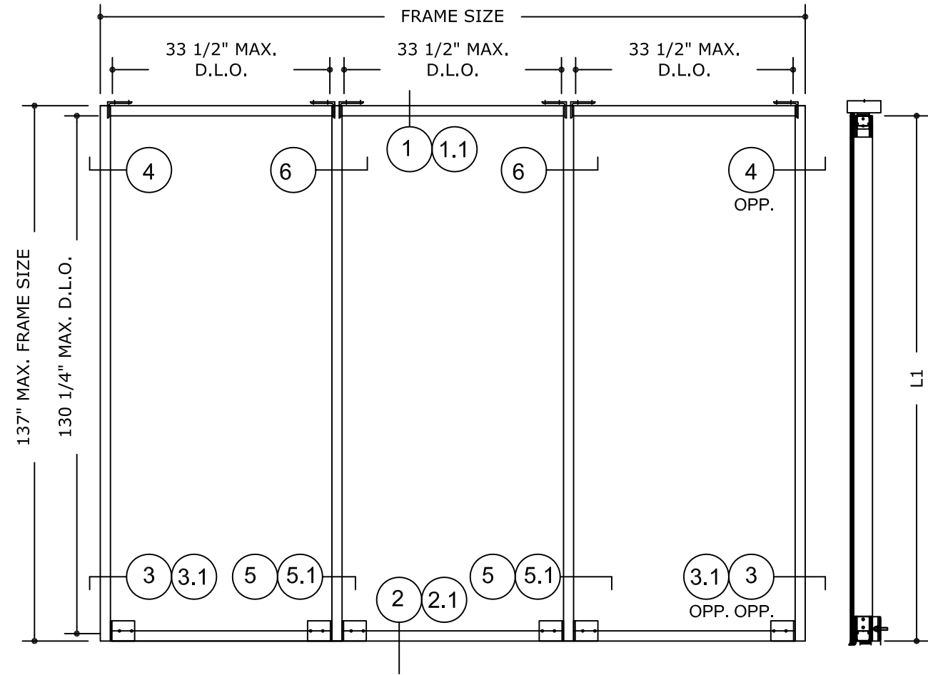
TYPICAL ELEVATION SINGLE SPAN N.T.S.
