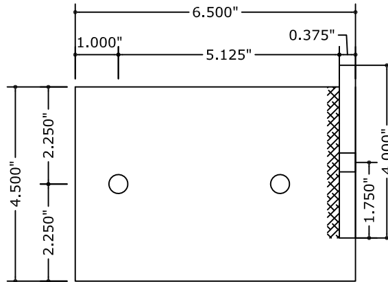
M14 ANCHOR BRACKET (AT JAMBS)
