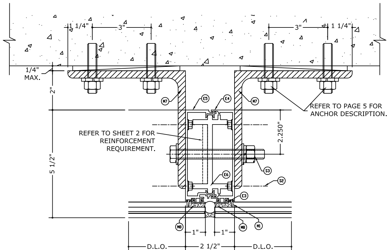
5 CONDITION AT MULLION BOTTOM N.T.S
