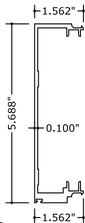
E10 VERTICAL MULLION MALE
