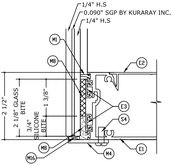
GLAZING DETAIL - GLASS TYPE 'B' TWIN SPAN (LARGE MISSILE )
