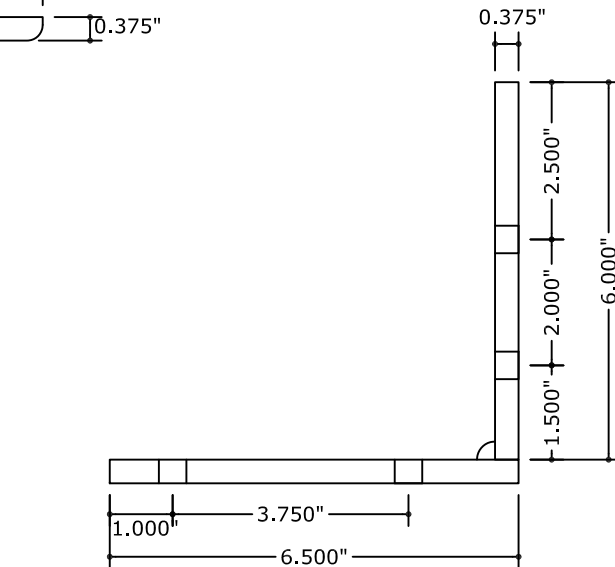
M7 ALUMINUM ANGLE
