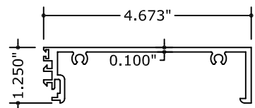
E7 EXPANSION JOINT BOTTOM
