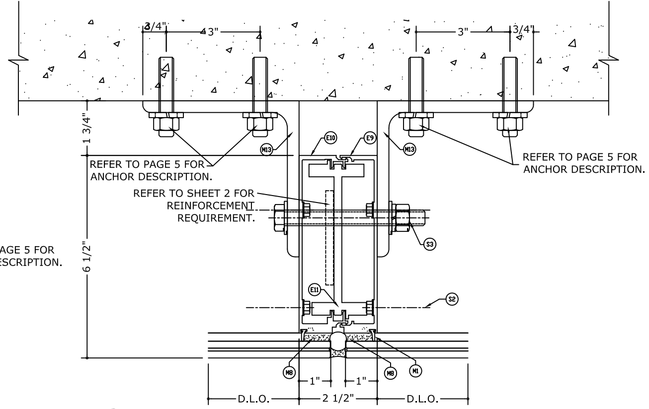
8.1 MID ANCHOR AT MULLION N.T.S
