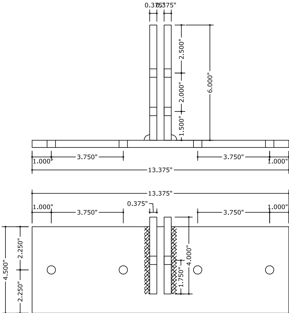
M15 ANCHOR BRACKET (AT MULLIONS)
