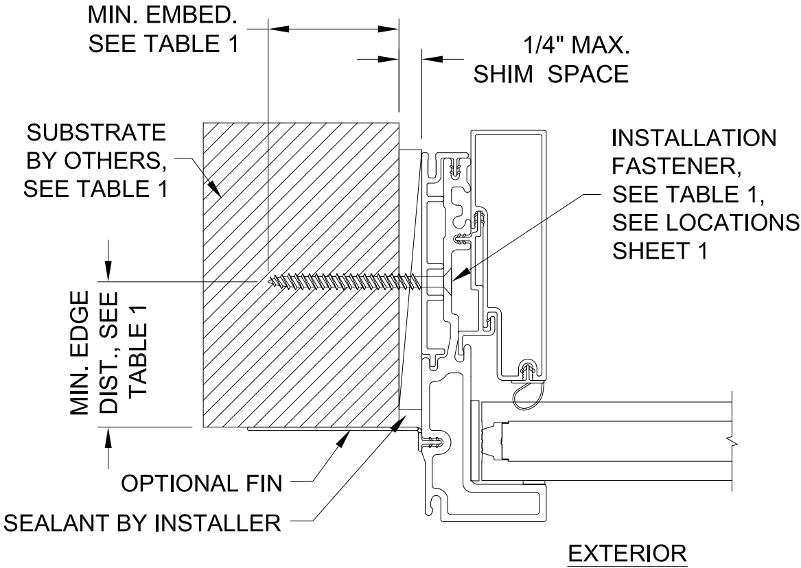
TYPICAL SECTION POLYGON 15/16"
