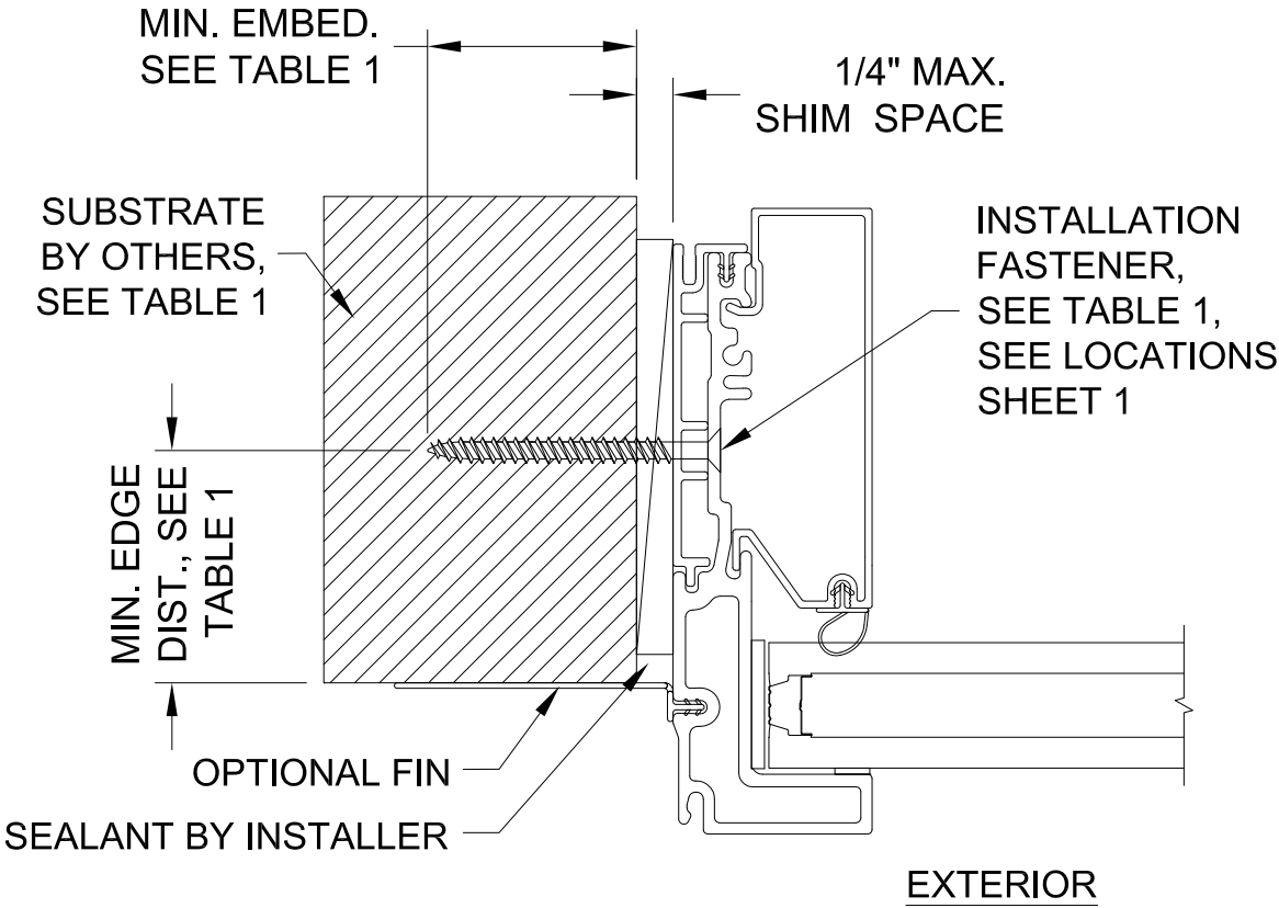
TYPICAL SECTION RECTANGLE 15/16"
