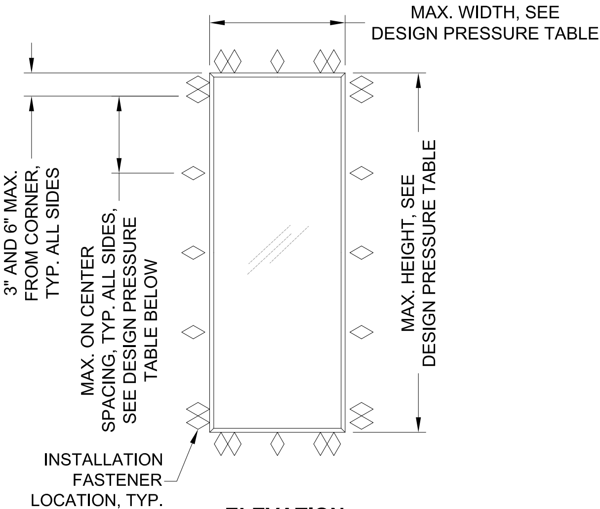
ELEVATION SEE DETAILS SHEETS 2 AND 3
