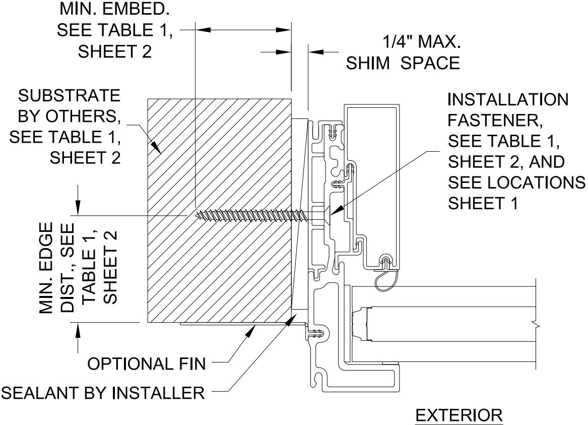
TYPICAL SECTION POLYGON 1-1/4"
