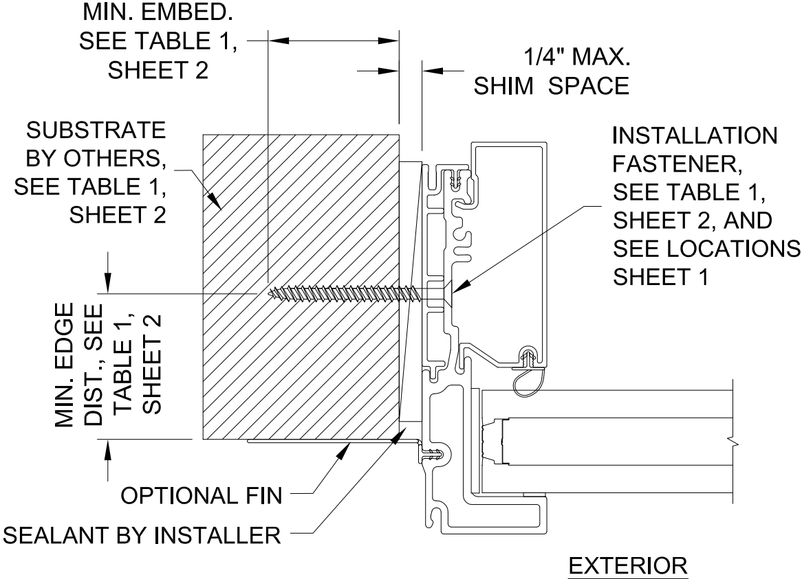
TYPICAL SECTION RECTANGLE 1-1/4"
