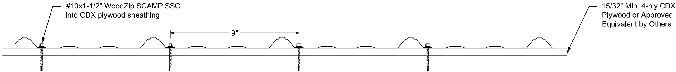
Fastener Pattern at Eave, Ridge and 3' O.C. in Field
