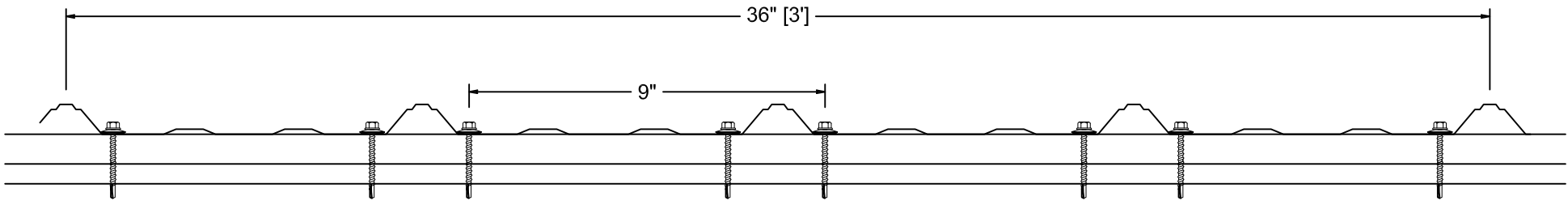
Fastener Pattern at Eave
