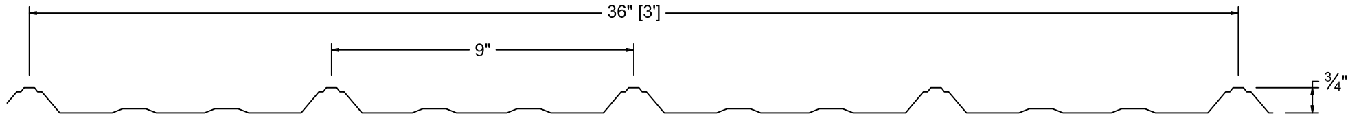
South Rib Profile
