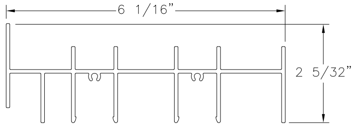
FRAME HEAD 2TRACK, FLANGE ALUMINUM 6005-T5 (M-2526)
