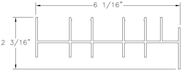
FRAME JAMB 2TRACK, FLANGE ALUMINUM 6005-T5 (M-2529)
