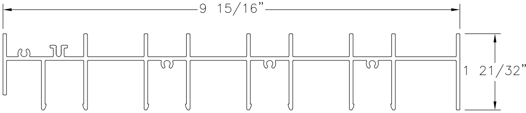
FRAME HEAD 4TRACK, FINLESS ALUMINUM 6005-T5 (M-2525)
