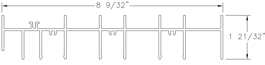
FRAME HEAD 3TRACK, FINLESS ALUMINUM 6005-T5 (M-2525)
