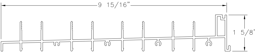
FRAME SILL 4TRACK ALUMINUM 6005-T5 (M-2527)
