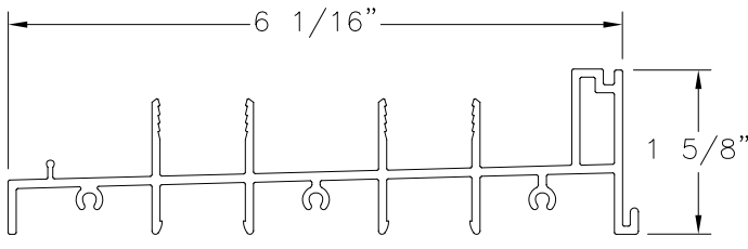
FRAME SILL 2TRACK ALUMINUM 6005-T5 (M-2527)
