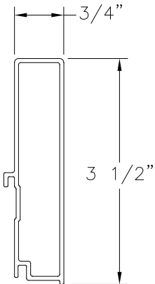
3 1/2 inch SILL EXTENDER ALUMINUM 6063-T5 .062" THICK
