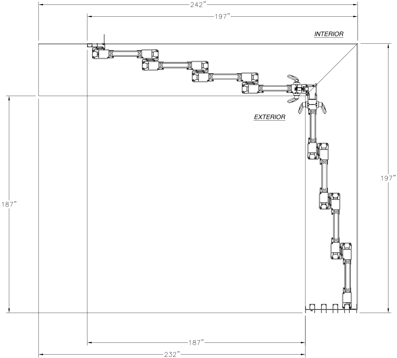
SERIES 120/130/140 ALUMINUM SGD INSIDE CORNER PLAN VIEW
