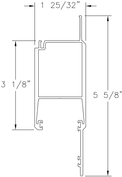
PANEL TOP STILE, INSIDE CORNER ALUMINUM 6005-T5 (M-2513)
