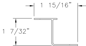
FIXED PANEL STILE RETAINER ALUMINUM 6063-T5 (M-2519)
