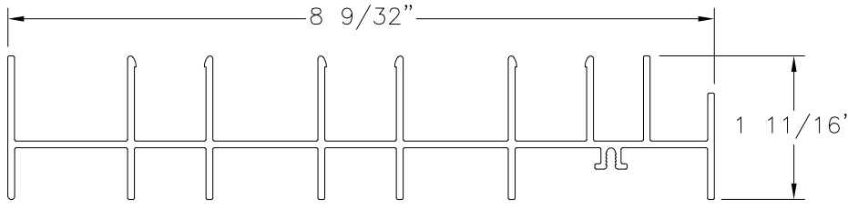
FRAME JAMB 3TRACK, FINLESS ALUMINUM 6005-T5 (M-2528)
