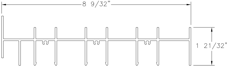
FRAME HEAD 3TRACK, FLANGE ALUMINUM 6005-T5 (M-2526)
