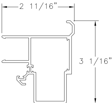
CORNER PANEL ADAPTER ALUMINUM 6005-T5 (M-2515)
