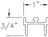
SILL SNAP-IN ROLLER TRACK ALUMINUM 6063-T5 (M-2511)
