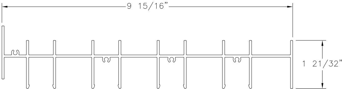
FRAME HEAD 4TRACK, FLANGE ALUMINUM 6005-T5 (M-2526)
