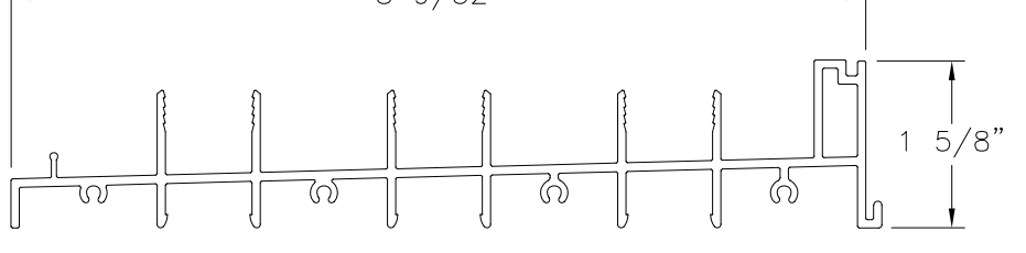
FRAME SILL 3TRACK ALUMINUM 6005-T5 (M-2527)
