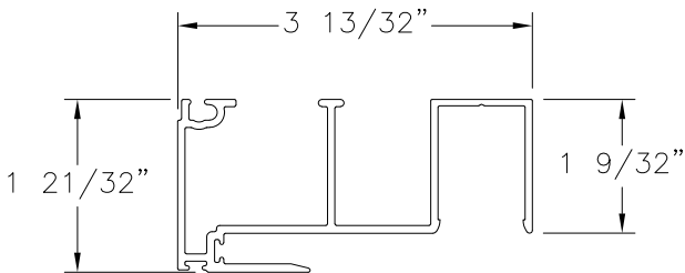
POCKET HOOK STRIP WITH OPTIONAL RISER ALUMINUM 6063-T5 (M-2534)
