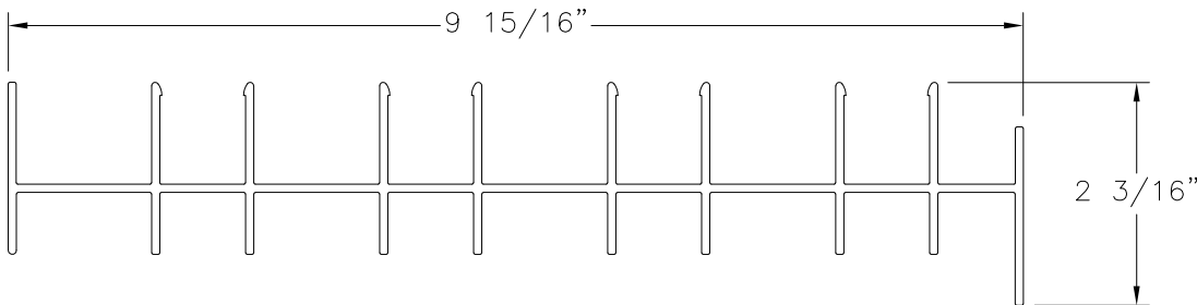
FRAME JAMB 4TRACK, FLANGE ALUMINUM 6005-T5 (M-2529)
