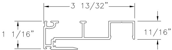
POCKET HOOK STRIP WITHOUT OPTIONAL RISER ALUMINUM 6063-T5 (M-2533)
