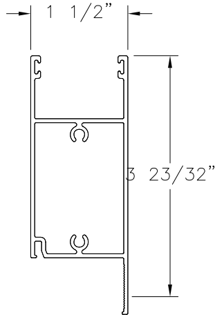
PANEL TOP RAIL ALUMINUM 6005-T5 (M-2500)
