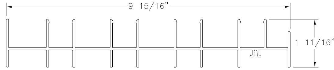
FRAME JAMB 4TRACK, FINLESS ALUMINUM 6005-T5 (M-2528)
