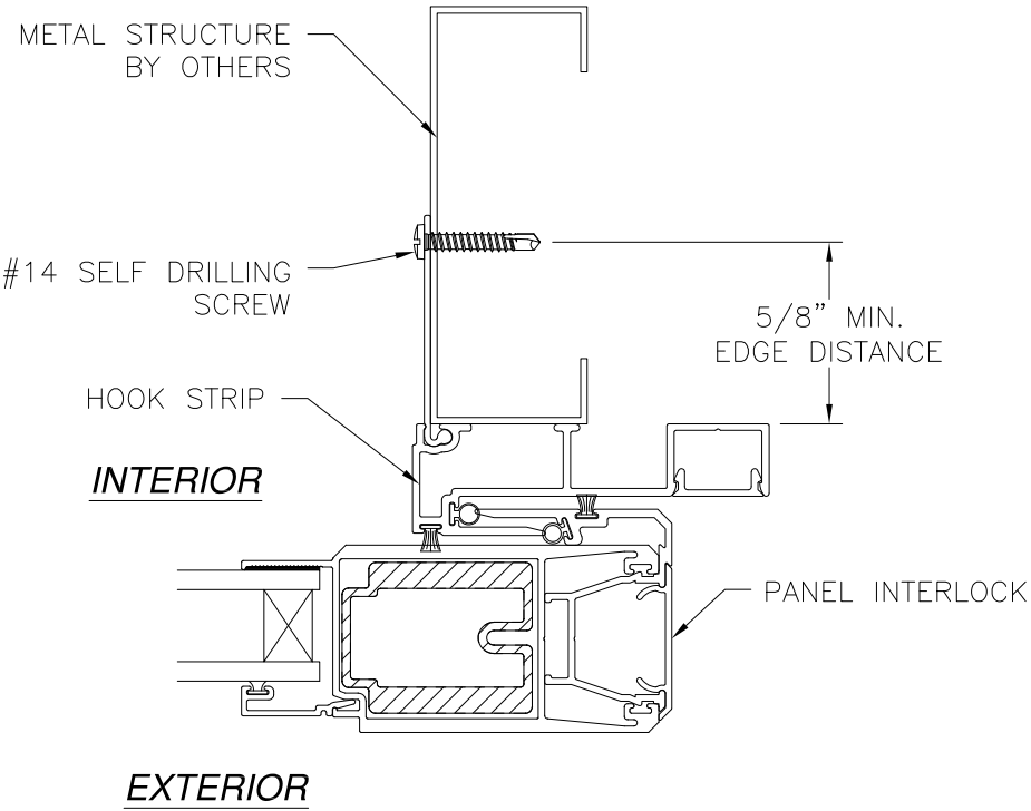
HOOK STRIP (M-2533) INSTALLATION METAL STRUCTURE
