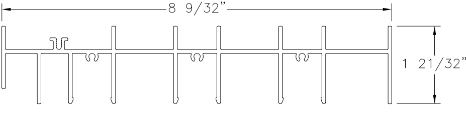
FRAME HEAD 3TRACK, FINLESS ALUMINUM 6005-T5 (M-2520)
