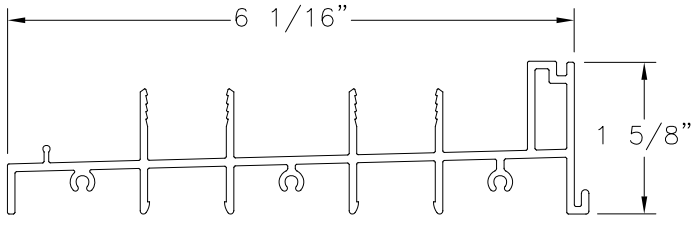
FRAME SILL 2TRACK ALUMINUM 6005-T5 (M-2522)
