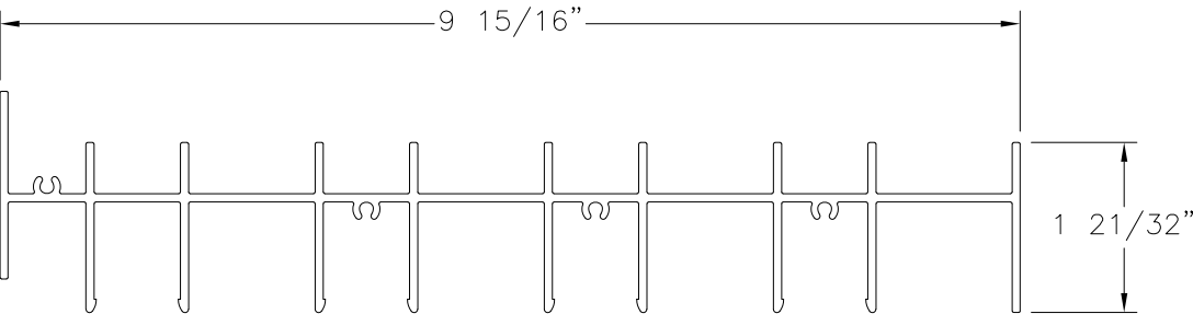
FRAME HEAD 4TRACK, FLANGE ALUMINUM 6005-T5 (M-2520)
