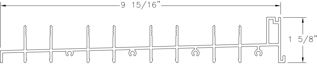
FRAME SILL 4TRACK ALUMINUM 6005-T5 (M-2522)
