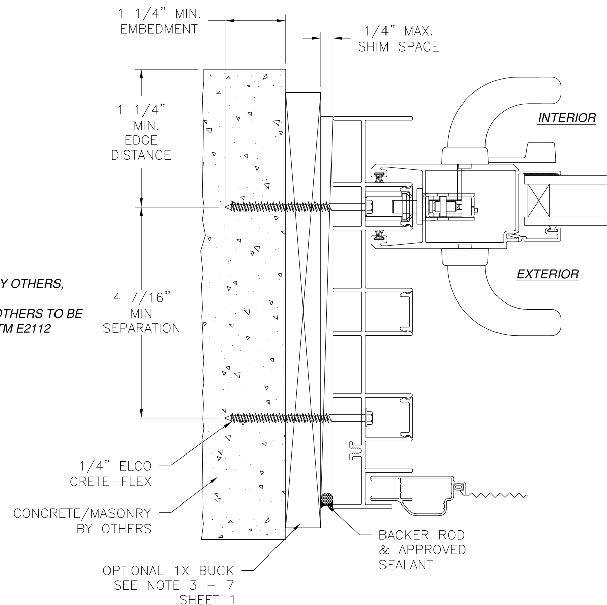
JAMB INSTALLATION DETAIL CONCRETE/MASONRY INSTALLATION SIGNED: 10/10/2018
