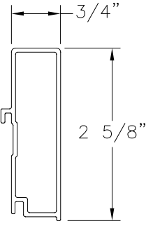
2 5/8" SILL EXTENDER ALUMINUM 6063-T5 .062" THICK
