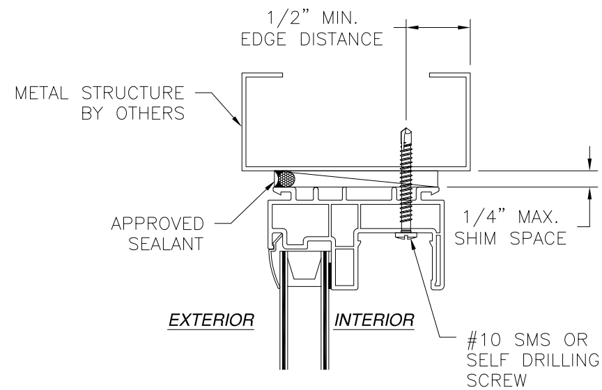
INSTALLATION DETAIL METAL STRUCTURE
