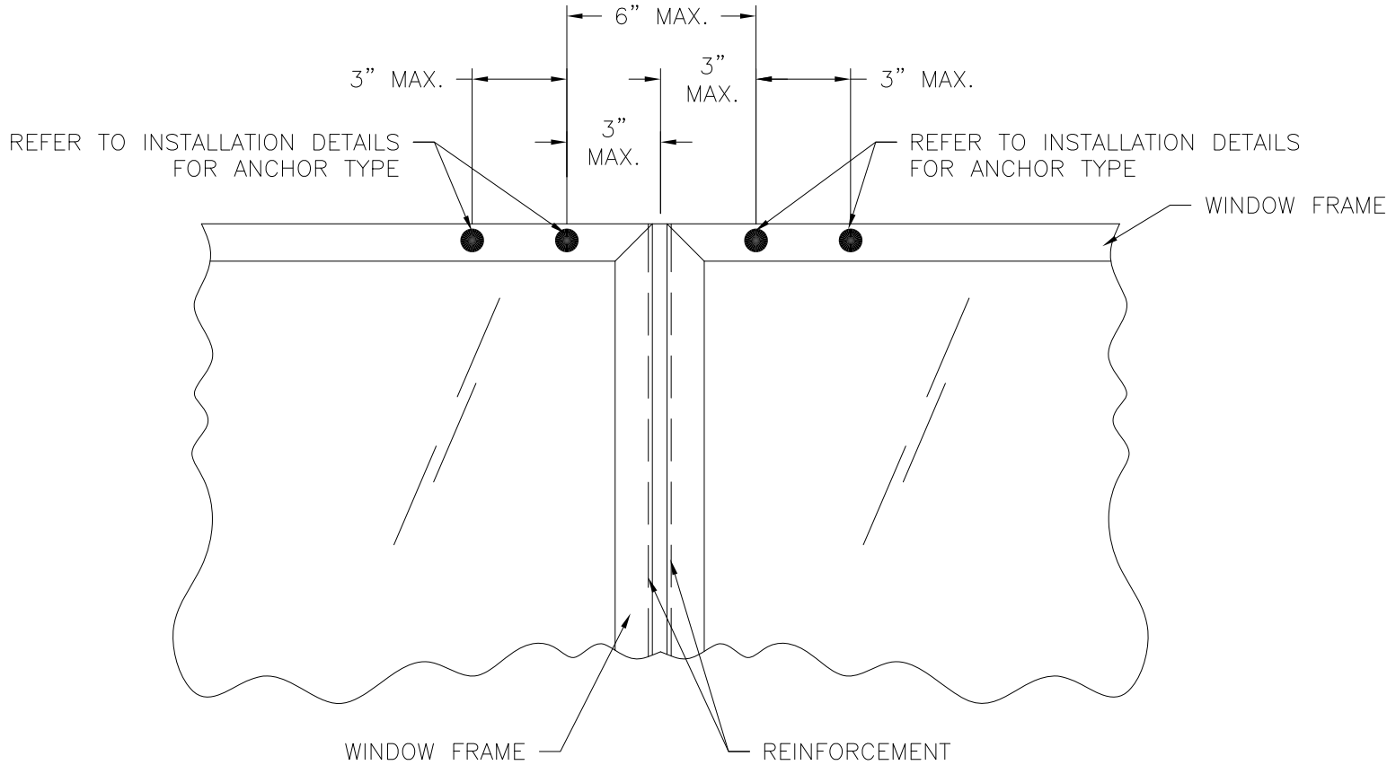
HEAD INSTALLATION DETAIL SILL SIMILAR
