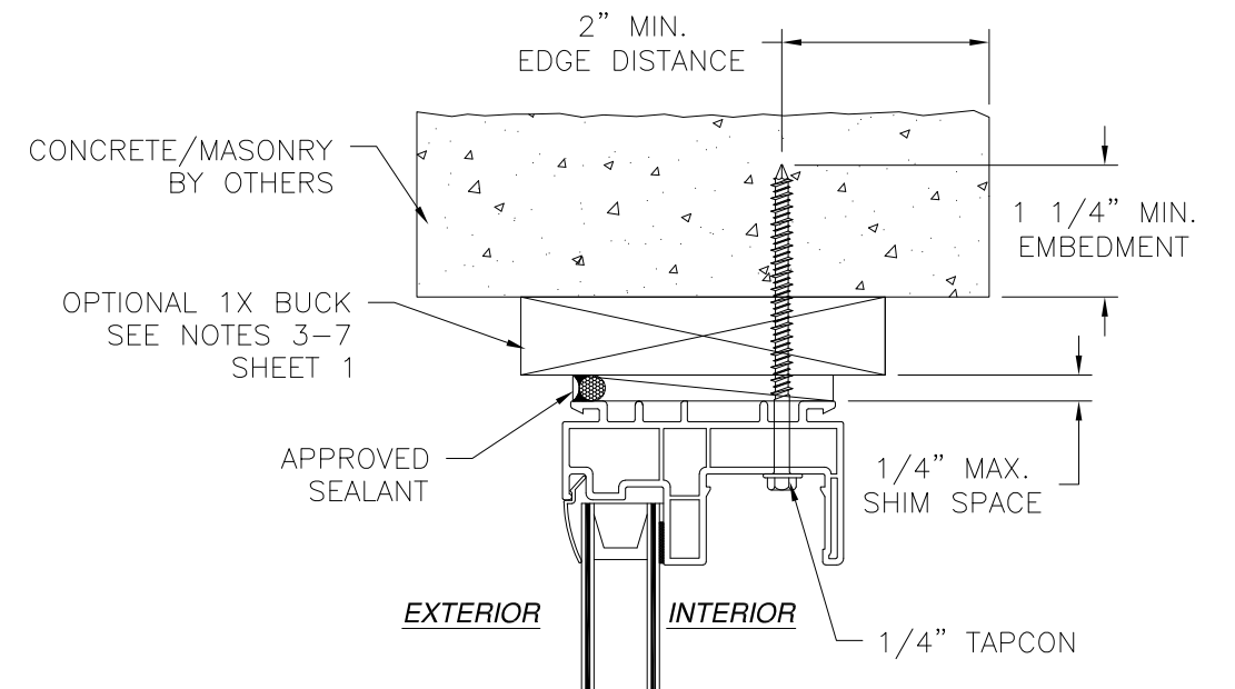
INSTALLATION DETAIL CONCRETE/MASONRY
