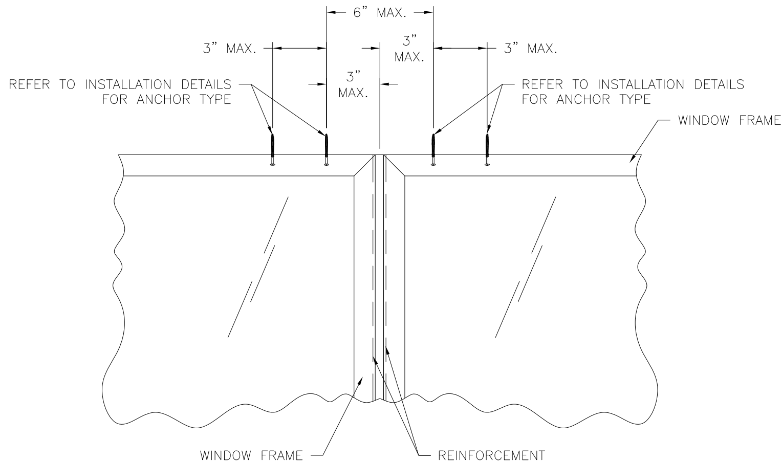
HEAD INSTALLATION DETAIL SILL SIMILAR
