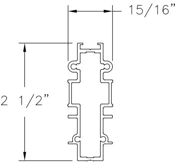
MULLION BAR REINFORCEMENT ALUMINUM 6063-T6 (T-53137)
