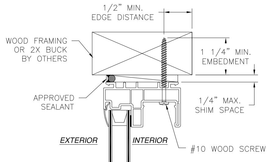
INSTALLATION DETAIL WOOD FRAMING OR 2X BUCK
