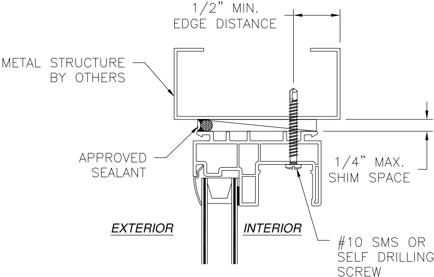
INSTALLATION DETAIL METAL STRUCTURE
