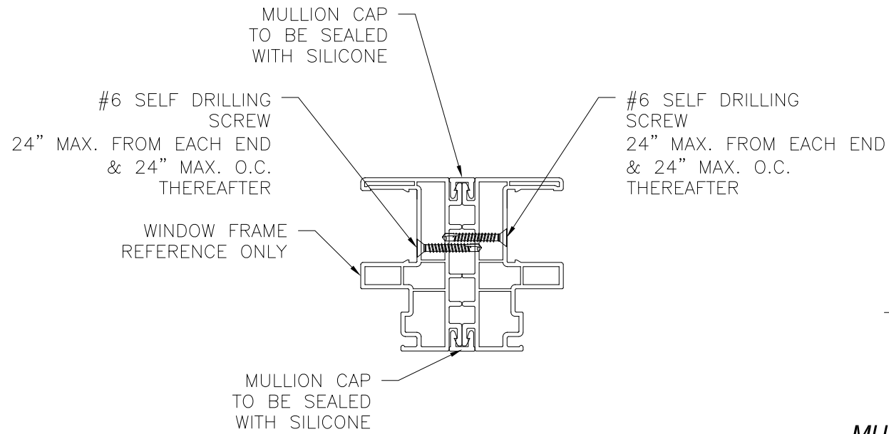
WINDOW CONNECTION DETAIL
