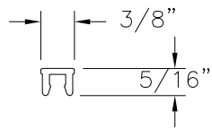
MULLION CAP VINYL PVC (600216)
