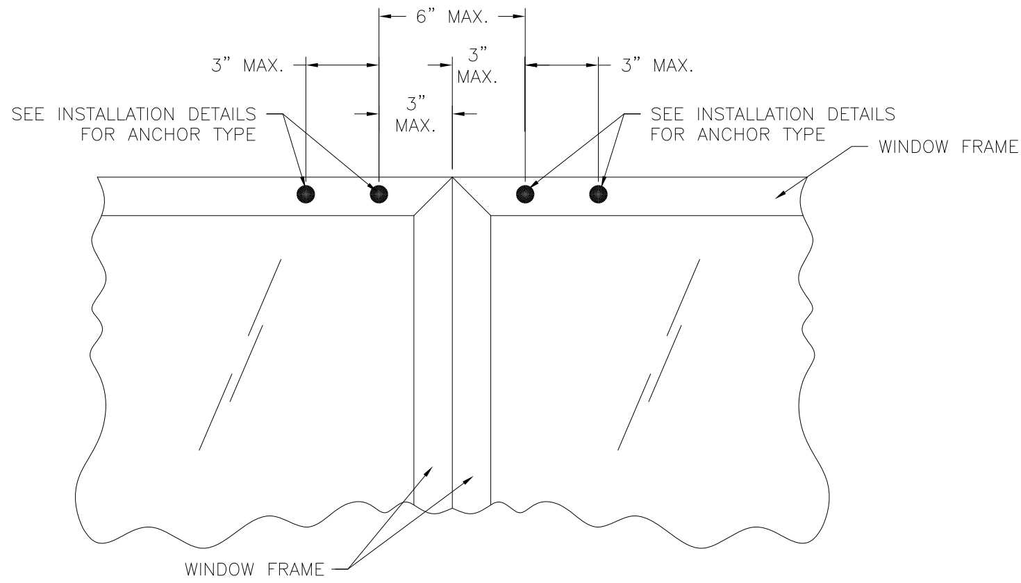
HEAD INSTALLATION DETAIL SILL SIMILAR
