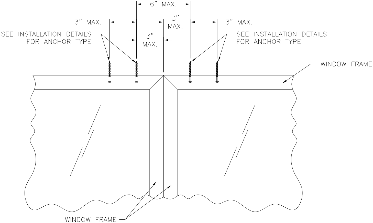
HEAD INSTALLATION DETAIL SILL SIMILAR
