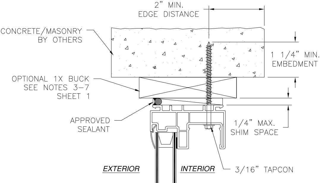
INSTALLATION DETAIL CONCRETE/MASONRY
