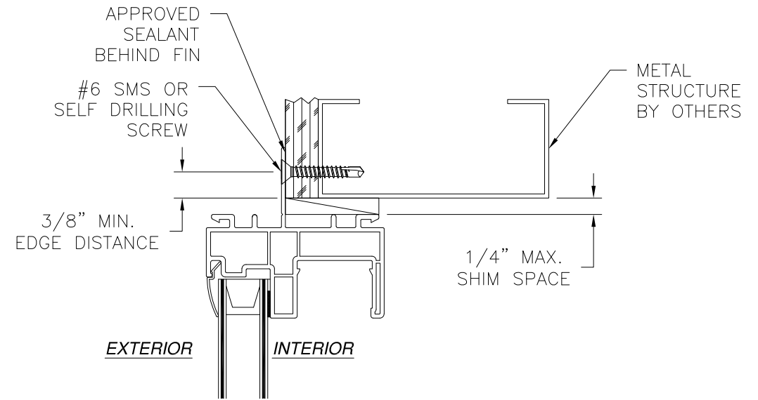
INSTALLATION DETAIL METAL STRUCTURE
