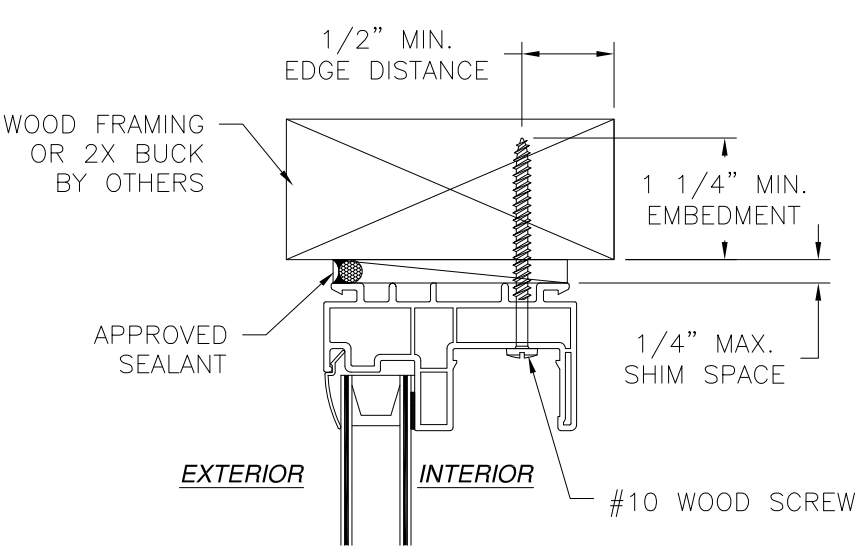
INSTALLATION DETAIL WOOD FRAMING OR 2X BUCK
