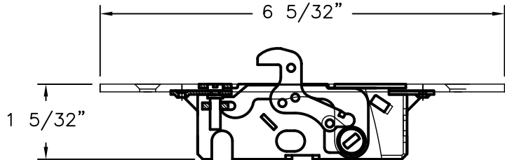
SINGLE LOCKING SYSTEM STAINLESS STEEL (SH721)
