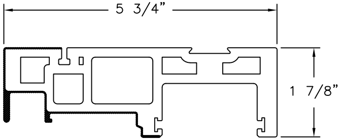
HEAD FRAME & JAMB FOAM PVC CO-EX
