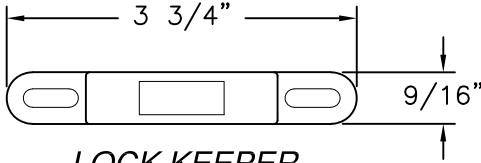
LOCK KEEPER STAINLESS STEEL (SH717)
