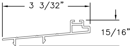
GLIDING SILL-(B) ALUMINUM
