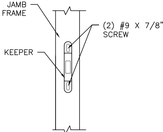
LOCK KEEPER DETAIL
