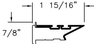
MEETING STILE INTERLOCK FOAM PVC CO-EX
